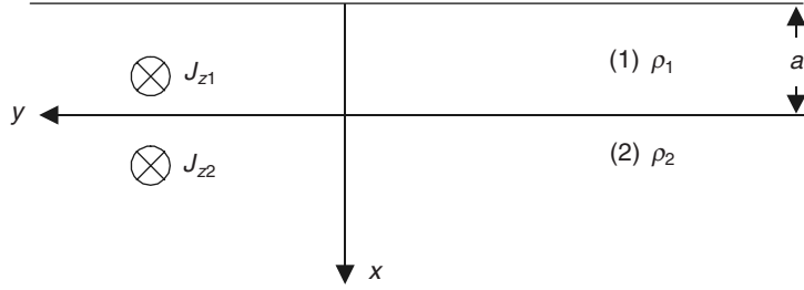
Figure 15.13 Semi-infinite metal block with a surface coating of thickness a .
