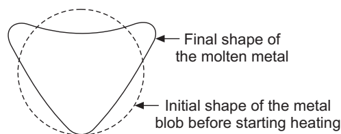
Figure 22.18(b) Change of shape of the metal blob. (The crucible coil is not shown here.)
