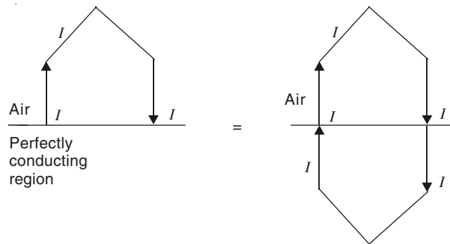
Figure 9.17 Image of a coil-end embedded partially in a perfectly conducting region, for the air-region.
