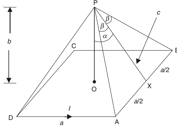
Figure 7.7 A square coil.
