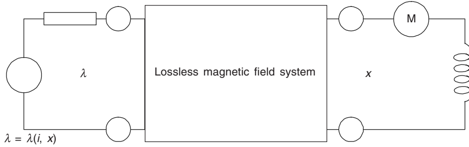
Figure 11.22 A terminal characteristic representation of a magnetic field electromechanical system.
