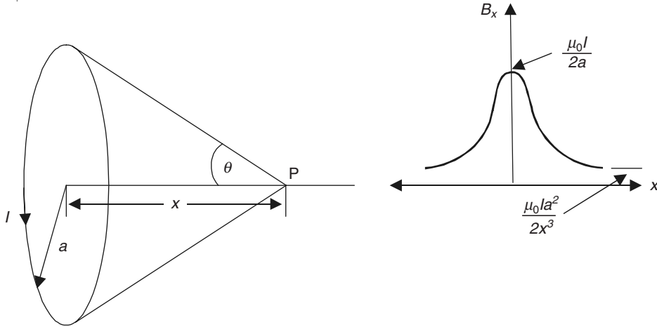
Figure 7.28 Magnetic field on the axis of a circular coil.
