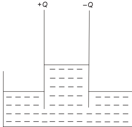
Figure 3.7 Forces pushing the liquid dielectric upwards.
