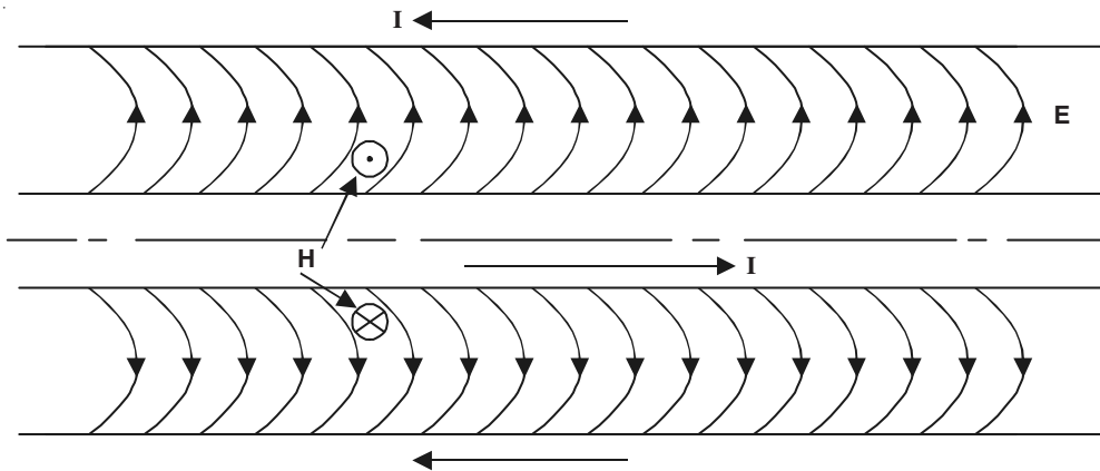
Figure 14.10 A coaxial cable having resistance and carrying a direct current.
