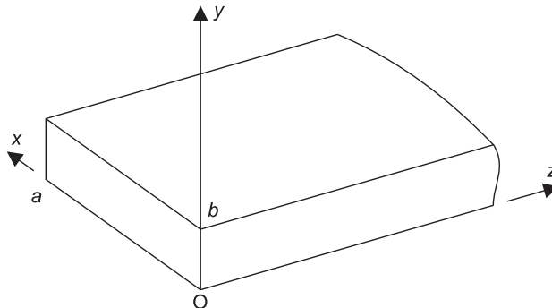
Figure 18.12 A rectangular waveguide, with cross-section a \times b , and the coordinate system as shown.
