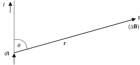
Figure 7.5 Magnetic field due to a current element.
