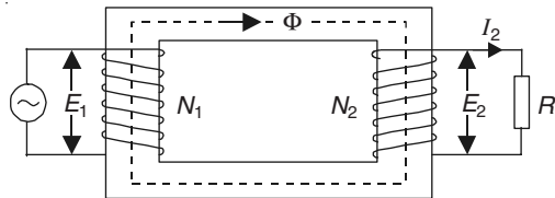
Figure 10.9 A transformer drawing a load current.
