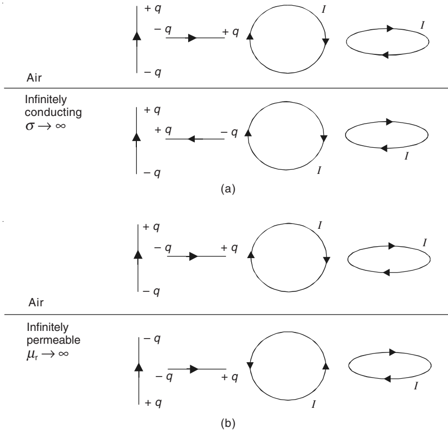
Figure 9.12 Images of doublets and current loops in the two limiting boundaries: (a) infinitely conducting and (b) infinitely permeable.
