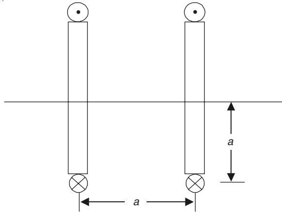
Figure 7.29 Helmholtz coils.
