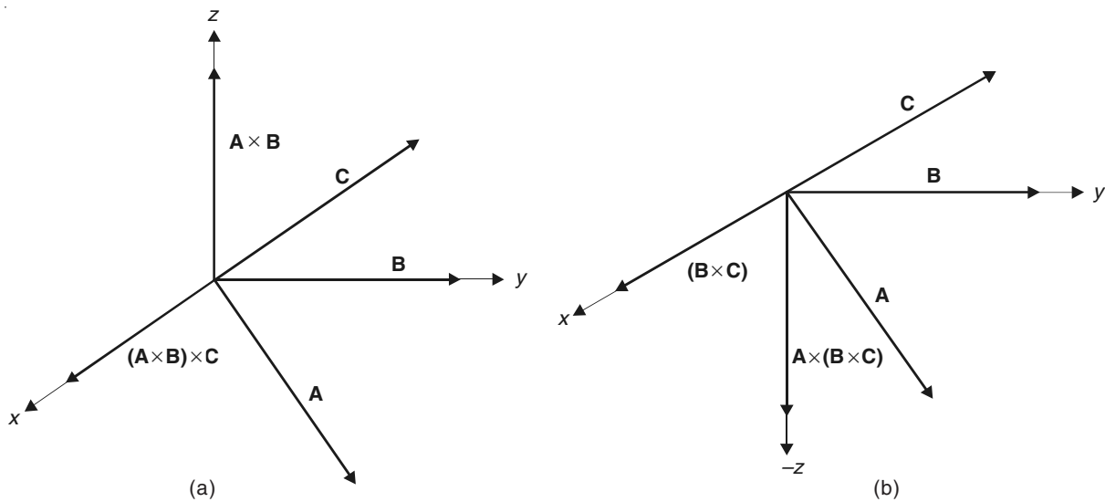
Figure 0.5 Vector triple product.
