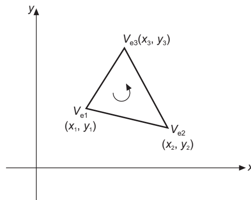
Figure 21.17 A typical triangular element.
