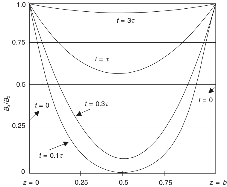
Figure 15.17 B_x as a function of z , with the time t as a parameter.
