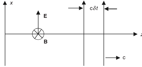
Figure 14.6 A uniform plane wave-front of \mathbf{E} field travelling forward in the +z -direction.
