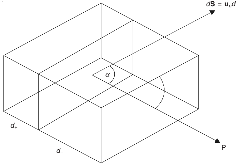
Figure 2.4 Movement of polarization charges for a distance (d_+ + d_-)
