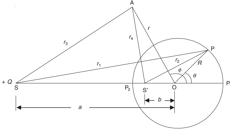
Section of the conducting sphere through the diametral plane containing the point charge Q at S
