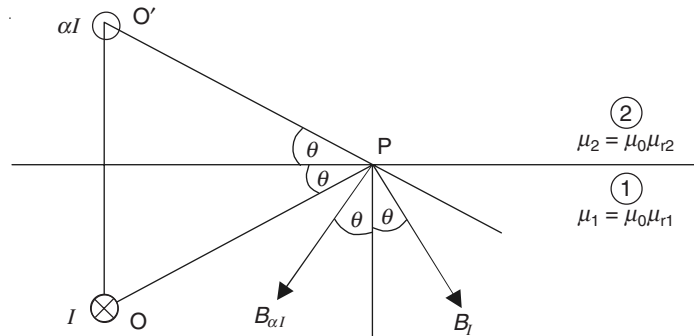
Figure 9.7 Electromagnetic image of a current-carrying conductor in a general problem.
