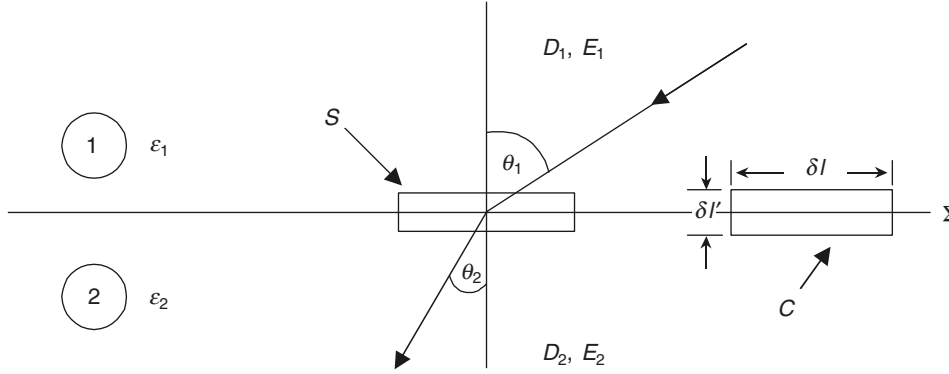
Figure 2.15 Surface of discontinuity.
