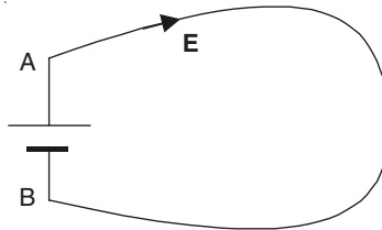
Figure 10.3 Battery loop.
