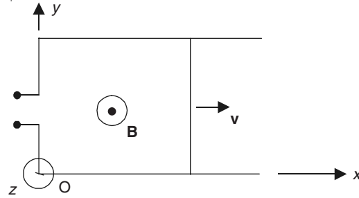
Figure 10.28 An expanding loop in a time-varying magnetic field.
