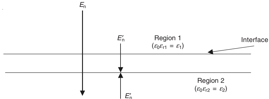
Figure 4.18 The induced field on the interface.
