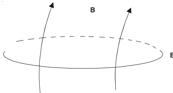
Figure 13.2 An electromagnetic field.
