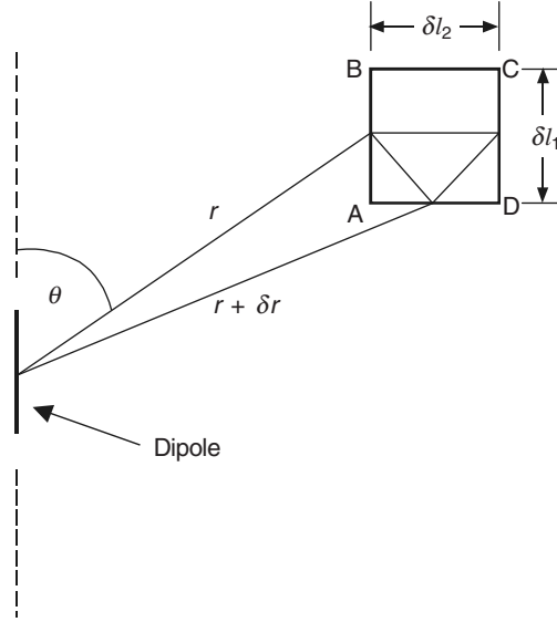
Figure 19.3 Contour for evaluating B_\phi due to the dipole.
