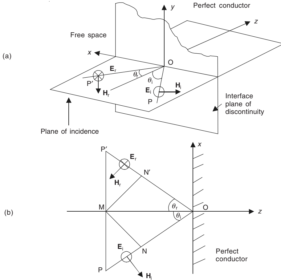
Figure 17.23 The incident and the reflected waves, for oblique incidence, with \mathbf{E} vector normal to the plane of incidence, on a perfectly conducting interface ( \sigma \rightarrow \infty ): (a) Isometric view; and (b) view along the plane of incidence.
