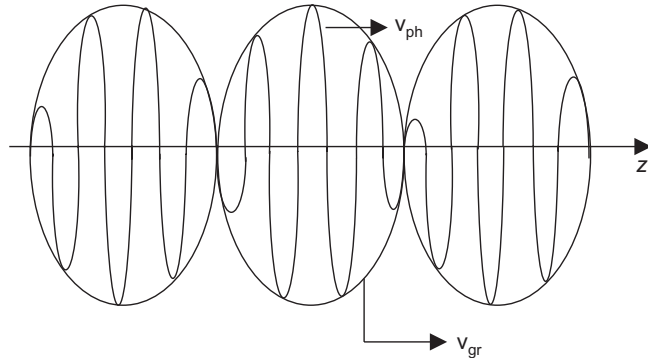
Figure 18.13(b) Sum of two sinusoidal waves of different frequencies.
