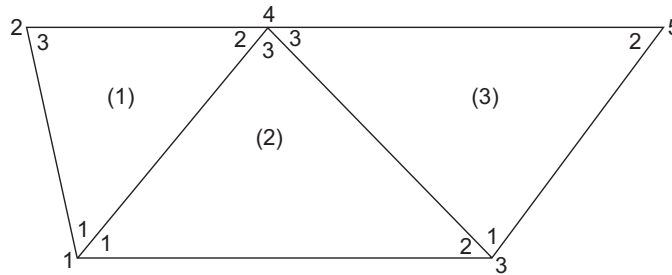
Figure 21.19 A collection of three elements.
