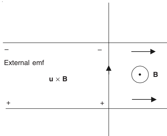
Figure 20.12 Flux-cutting emf.
