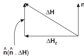
Figure A.8.2 Directions of the unit vectors.
