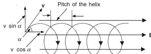
Figure 11.11 Helical path of a charged particle in a uniform \mathbf{B} field.
