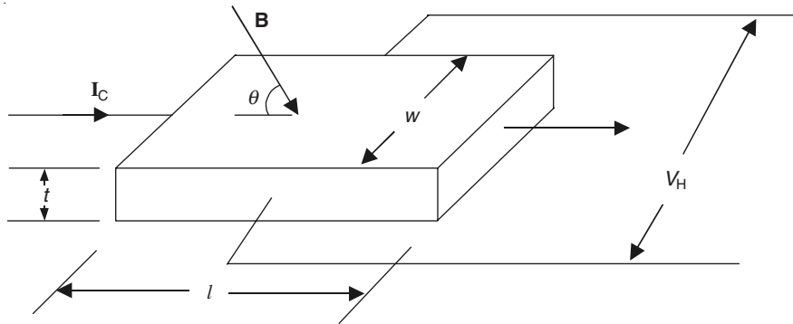
Figure 9.24 The Hall effect.
