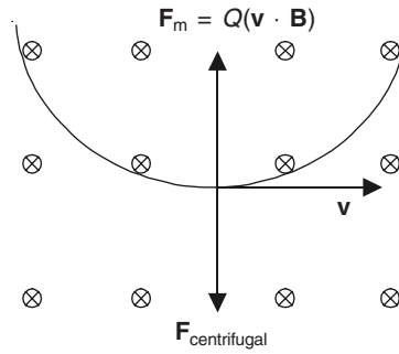
Figure 11.10 A charged particle moving at right angles to a uniform magnetic field.
