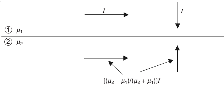
Figure 9.11 Supposed images of current elements.
