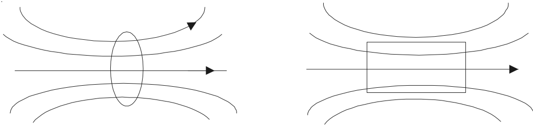
Figure 7.2 Equivalence between a current loop and a magnetic dipole.
