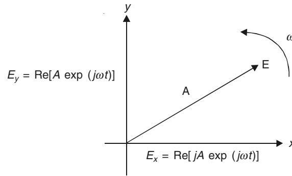
Figure 0.18 A two-dimensional rotating vector.
