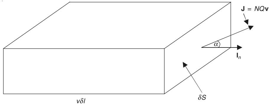
Figure 6.1 A planar surface \delta S with current across it.
