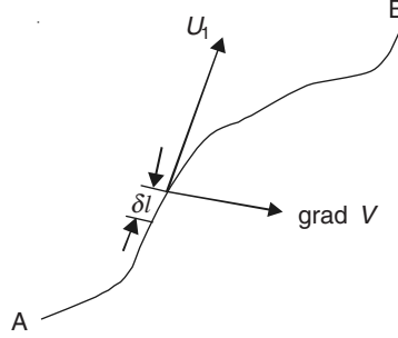
Figure 1.10 Potential difference.
