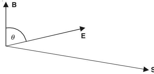
Figure 14.13(a) Poynting vector.
