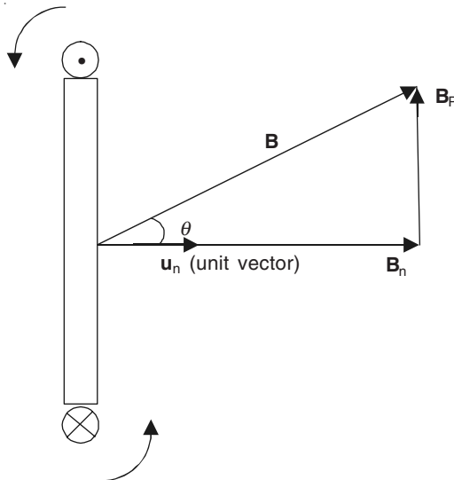
Figure 8.3 Torque of the magnetic force tending to align the vectors \mathbf{u}_n and \mathbf{B} .
