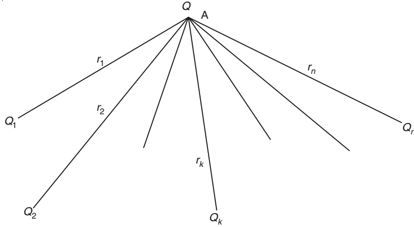
Figure 1.2 Distributed charges.
