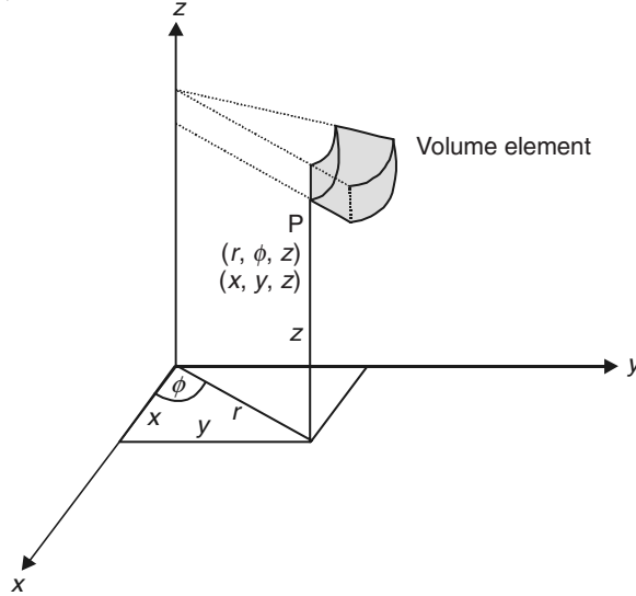
Figure 0.7 Elements in a cylindrical polar coordinate system.
