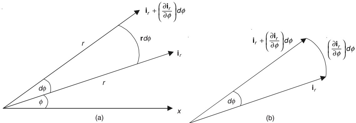
Figure A.4.6 Vector diagram for evaluating \partial \mathbf{i}_r / \partial \phi .
