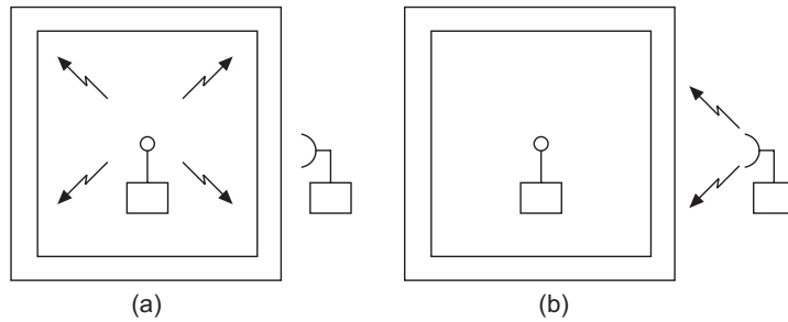
Figure 22.2 Electromagnetic shielding.
