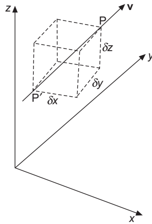
Figure 0.19 The points P and P' to illustrate the relationship between \frac{\partial \mathbf{A}}{\partial t} and \frac{d\mathbf{A}}{dt} .
