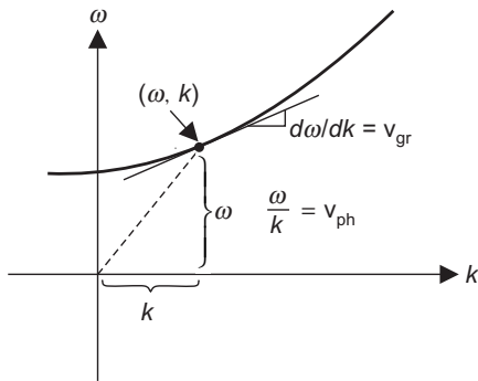
Figure 18.13(a) The slope of the line joining the point (\omega, k) and the origin is the phase velocity. The tangent of the \omega-k curve at this same point is the group velocity.
