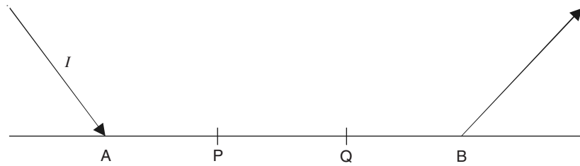
Figure 9.29 Current through a line in an anisotropic medium.
