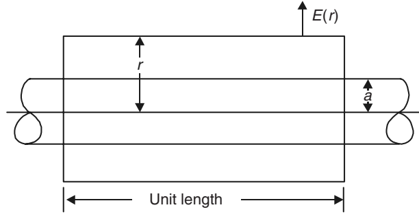
Figure 1.14 Infinitely long charged cylinder.
