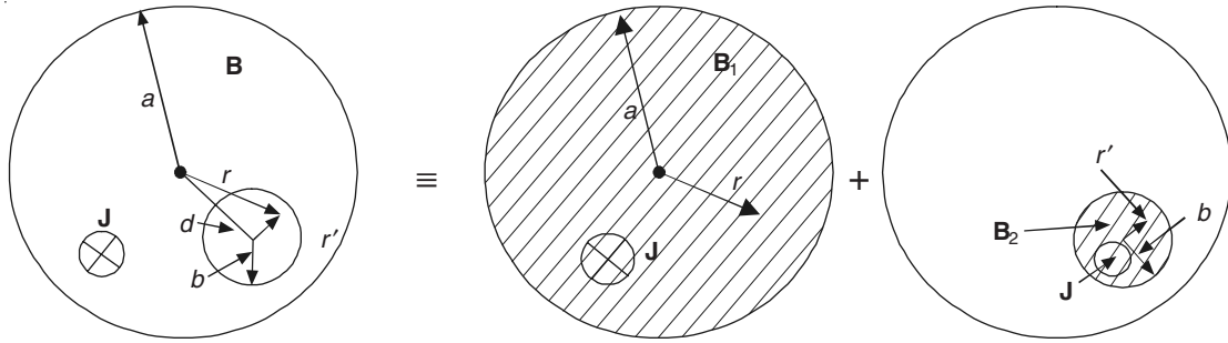
Figure 7.25 Circular conductor (with a hole) resolved into equivalent conductors.
