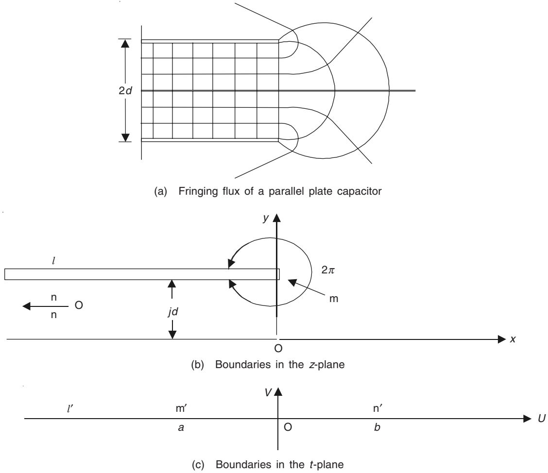
Figure 4.15 Transformations of the parallel plate capacitor with fringing at the ends.
