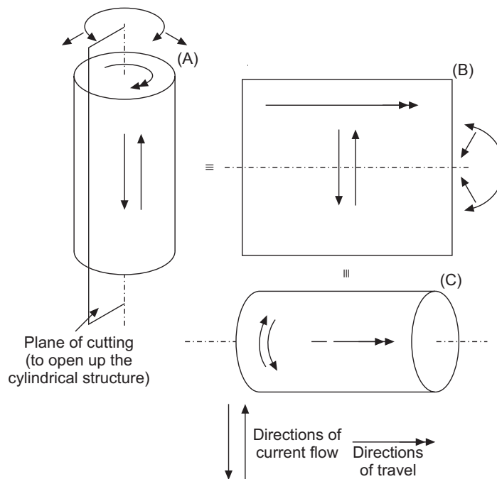
Figure 22.14 Topological manipulations to convert a cylindrical machine (A) to a flat linear machine (B), and then to a tubular linear machine (C). The direction of magnetic flux is radial in (A), normal to the plane of paper in (B), and again radial in (C).
