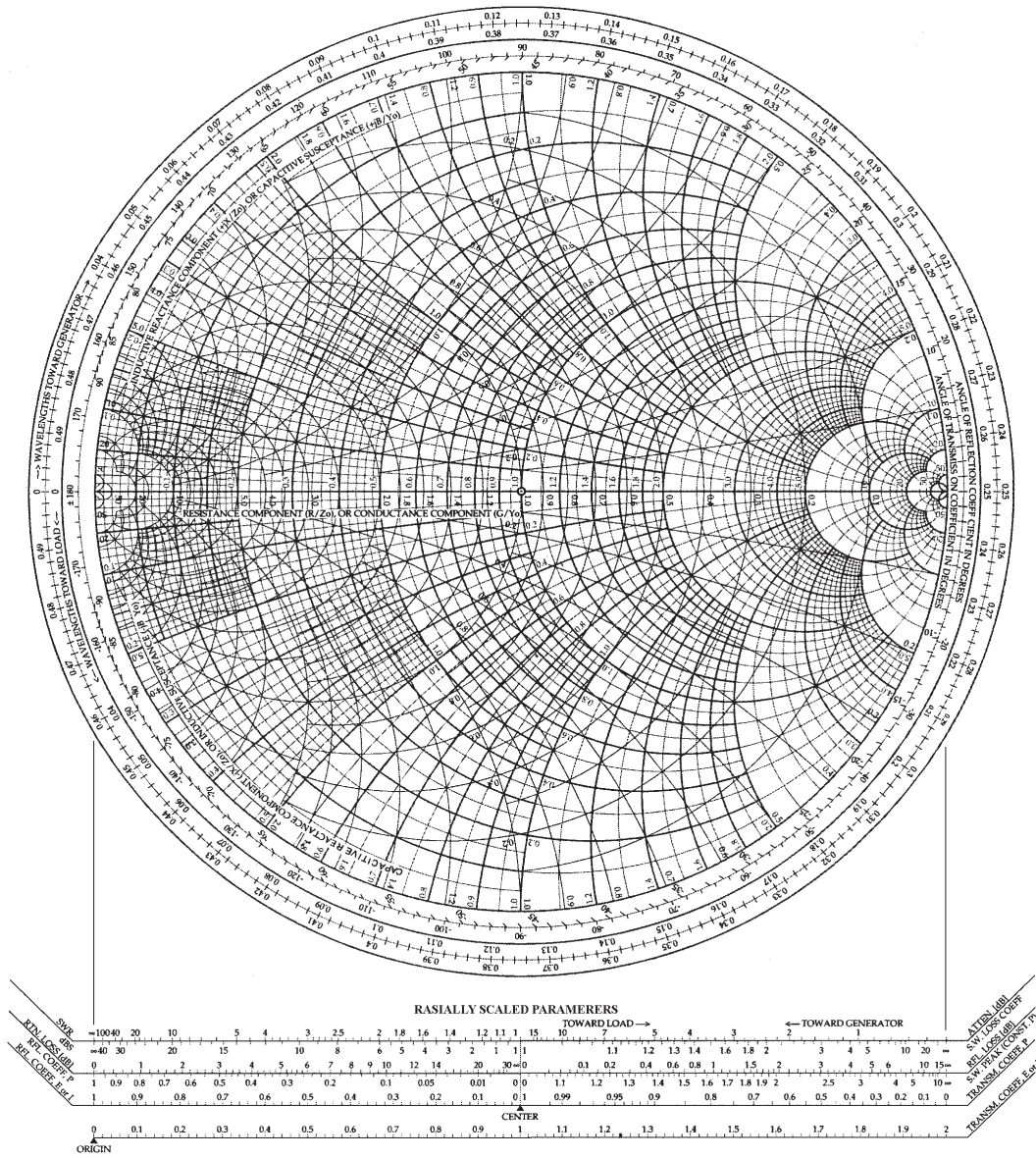
Figure A.7.8 Normalized impedance and admittance coordinates.
