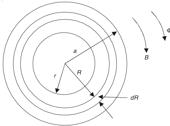
Figure 15.10 A circular conductor of radius a , carrying an alternating current.
