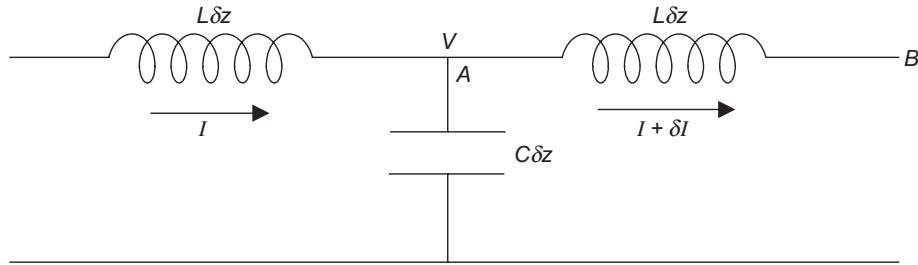
Figure 18.1 Circuit element representation of the transmission line.
