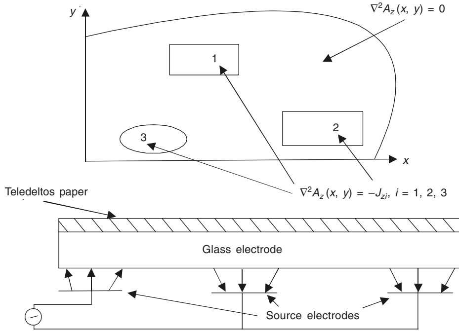
Figure 9.30 A multiple-source Poissonian and Laplacian field problem and its capacitive analogue.
