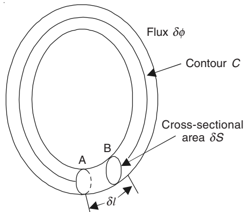
Figure 11.15 A closed filament.
