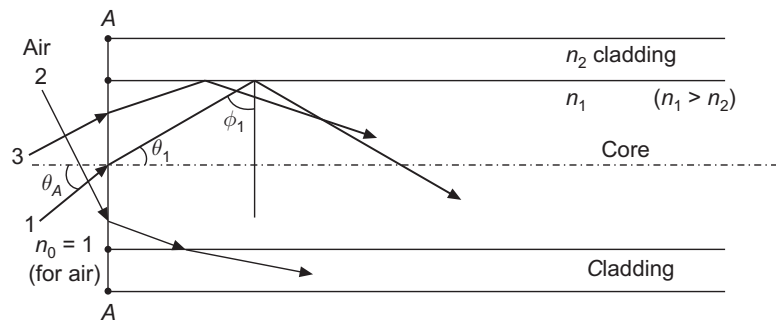
Figure 22.10 Numerical aperture and acceptance angle (longitudinal section of the fibre).
