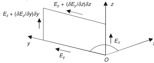
Figure 10.4 Rectangular loop in the y - z plane for evaluating the line-integral E_1 dl .
