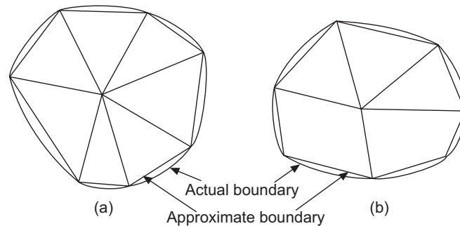
Figure 21.16 Typical irregular domain, sub-divided into (a) triangular elements only and (b) a combination of triangular and quadrilateral elements.
