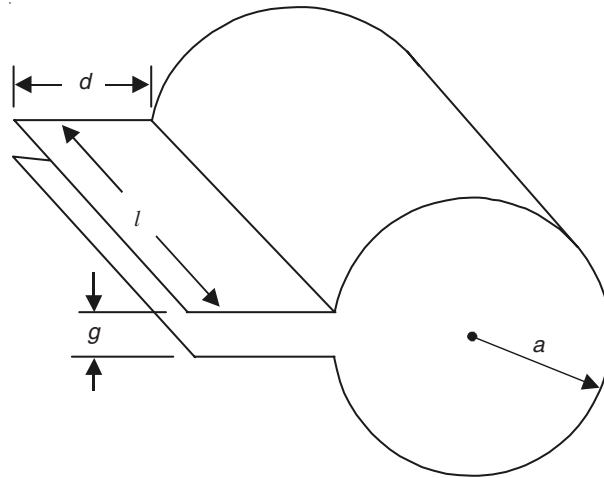
Figure 14.1 Inductor connected in parallel with a parallel plate capacitor.
