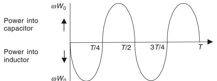
Figure 14.5 Rate of flow of energy between the inductor and the capacitor in a resonant oscillatory circuit.
