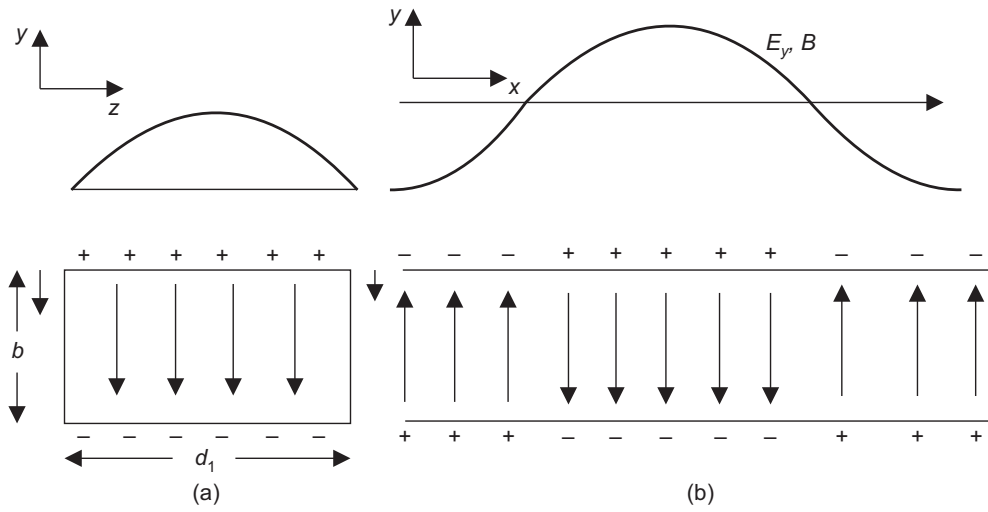
Figure 18.8 Field pattern in a rectangular waveguide (refer to Figure 17.24, for correspondence with the incident wave direction).
