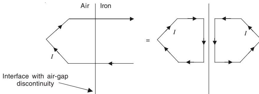
Figure 9.19 Image system for a coil-end in an infinitely long air-gap.
