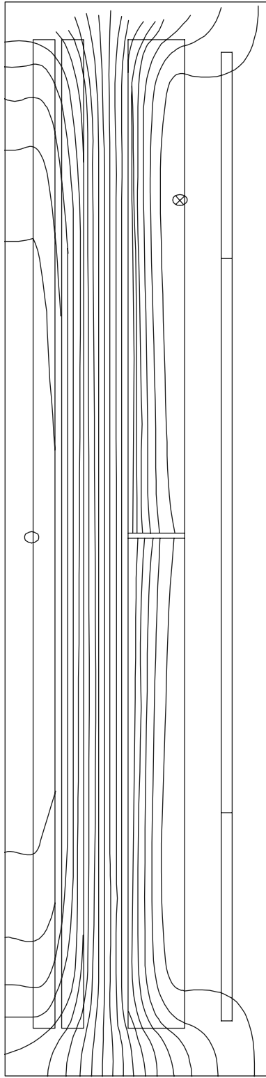
Figure 21.8 250 MVA 220 kV generator transformer window section—analysis in r - z coordinates.
