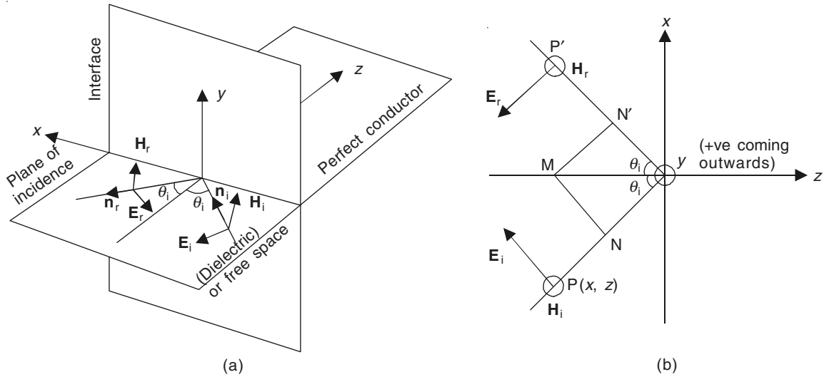
Figure 17.22 The incident and the reflected waves, for oblique incidence (with the \mathbf{E} vector in the plane of incidence) on the perfectly conducting interface ( \sigma \rightarrow \infty ): (a) Isometric view; (b) view along the plane of incidence ( z - x plane).
