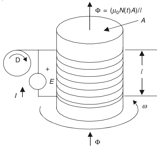
Figure 10.24 Time-varying number of turns on a coil in a uniform increasing magnetic field.
