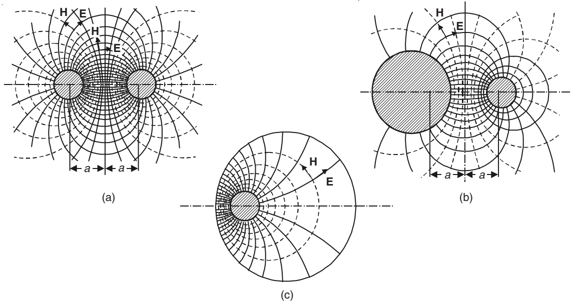
Figure A.7.1 TEM wave between parallel conductors. Bi-cylindrical coordinates are used for all three cases.
