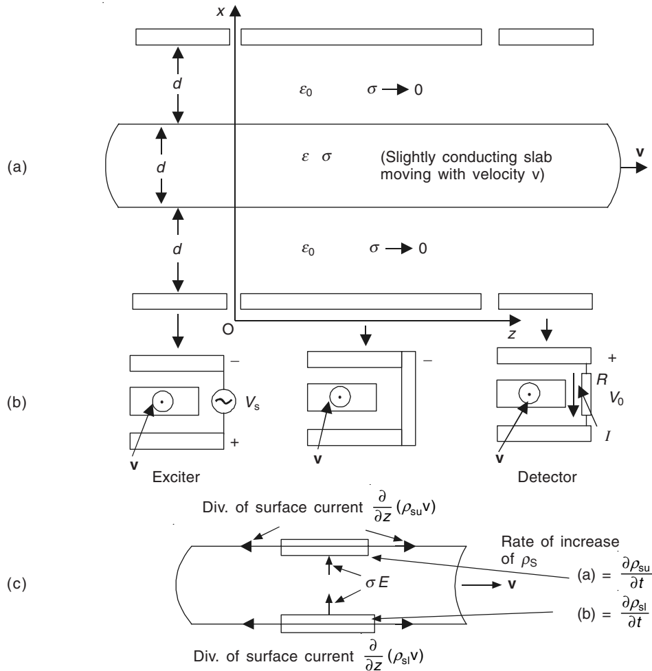
Figure 16.4 (a) A slightly conducting thin slab, moving to the right with constant velocity \mathbf{v} through electric fields imposed and constrained as shown in (b); (c) conduction currents normal to the surfaces produce a surface charge accumulation as shown.
