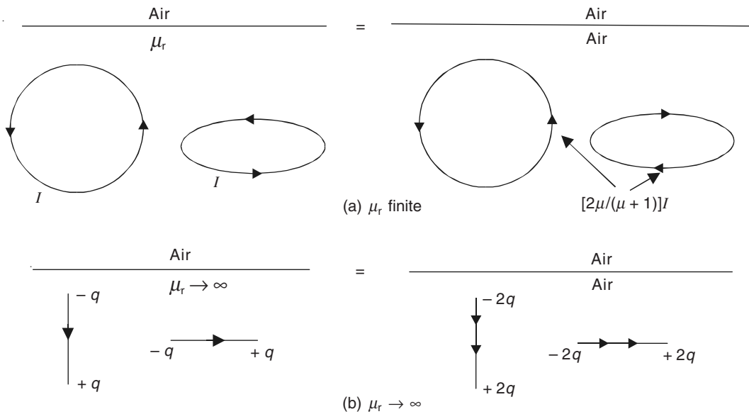
Figure 9.13 Images when the sources are embedded in iron of (a) finite \mu and (b) infinite \mu .
