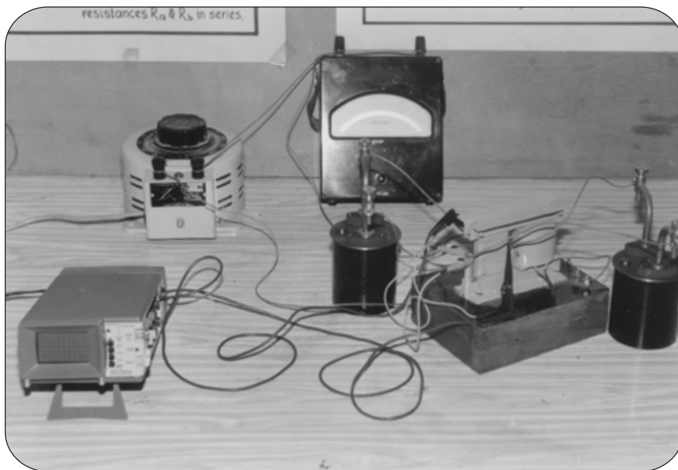
Plate 4 A view of the model experiment to demonstrate the double-valued P.D. in the circulating current circuit.
