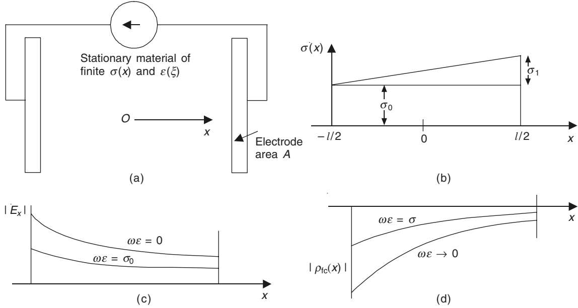
Figure 16.2 (a) A partially conducting material, bounded by plane electrodes; (b) \sigma distribution between the electrodes; (c) E_x distribution; and (d) \rho_{fc} distribution.
