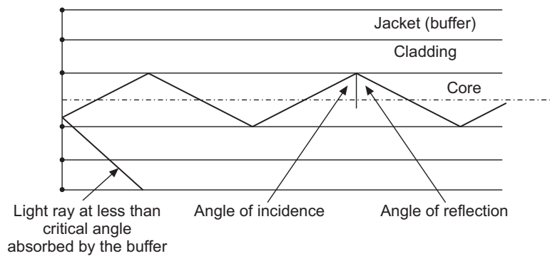
Figure 22.7 Behaviour of light ray in a fibre.
