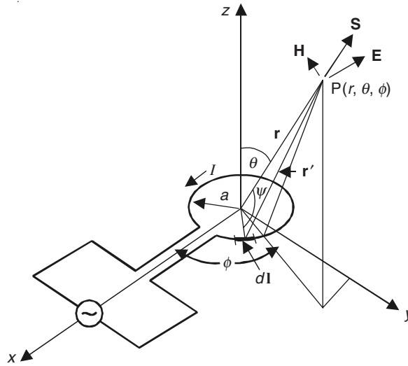
Figure 19.10 Magnetic dipole antenna fed by an oscillator.
