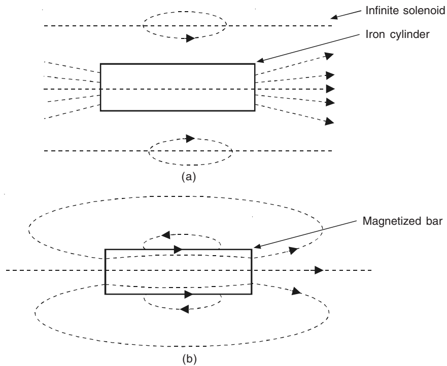
Figure 8.10 (a) H lines of the iron cylinder inside a solenoid and (b) H lines of the magnetized bar.
