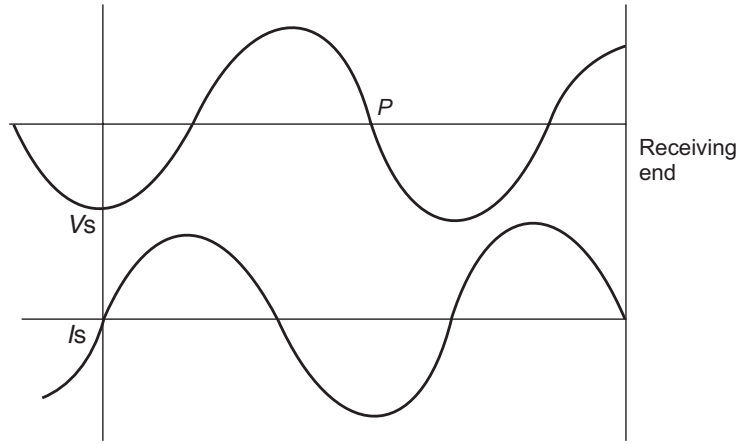
Figure 18.5 Standing wave patterns for V and I for an O.C. transmission line.
