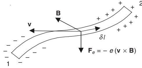
Figure 10.5 A piece of wire moving in a magnetic field.
