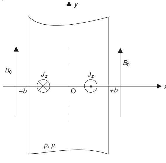
Figure 15.6 Plane faced metal block.
