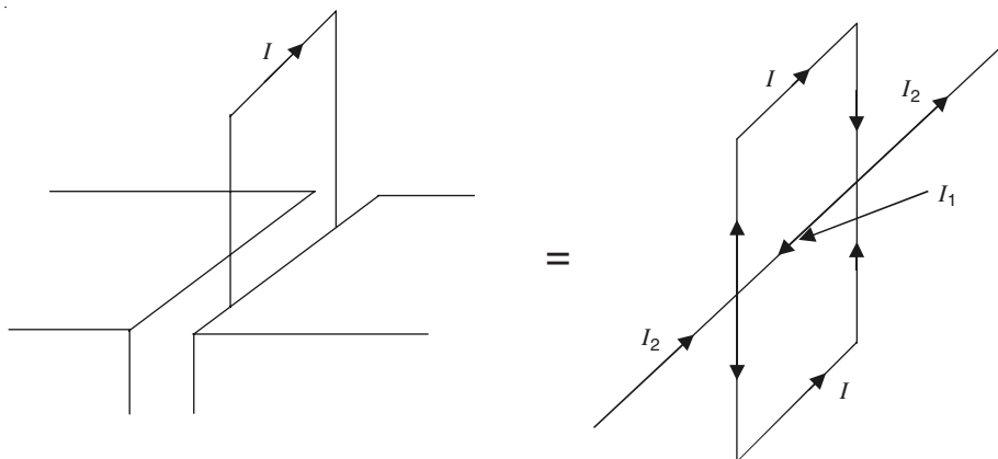
Figure 9.21 Image representation of air-gap of finite length and a coil-end of any general pitch.
