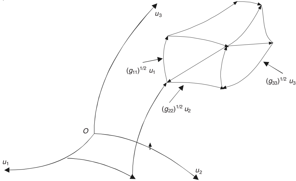
Figure A.4.2 Length elements in a general curvilinear coordinate system.
