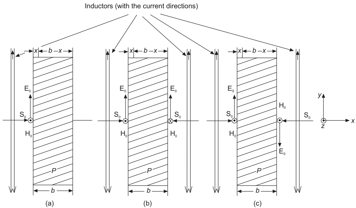
Figure 15.31 Induction heating systems of flat plate: (a) unilateral heating, (b) bilateral heating with compatible currents, and (c) bilateral heating with inverse currents.
