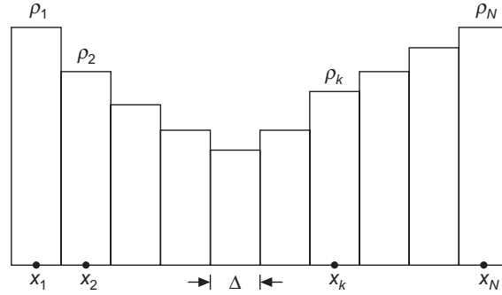
Figure A.11.2 Charged wire sub-divided into N segments.
