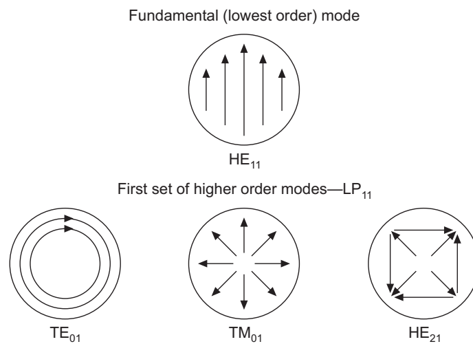
Figure 22.11 E field vectors in step-index waveguide lowest order modes.
