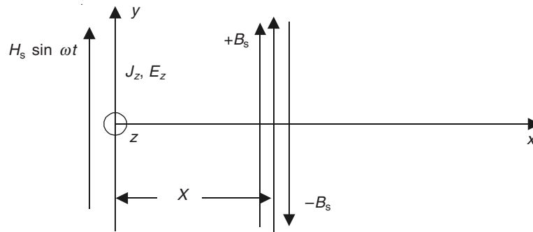
Figure 15.25 Penetration of flux in a semi-infinite iron block.
