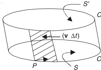
Figure 10.7 The path of integration moves from C to C' in the time \Delta t . The displacement is general (involving translation, rotation, and distortion).
