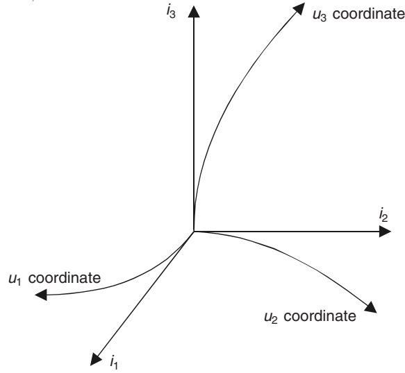
Figure A.4.1 Orthogonal curvilinear coordinates.
