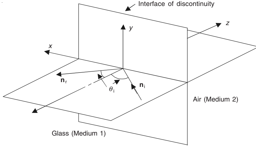
Figure 17.20 Total reflection.
