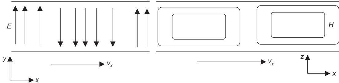
Figure 18.10 \mathbf{E} and \mathbf{H} lines along the direction of propagation: (a) \mathbf{E} lines and (b) \mathbf{H} lines.
