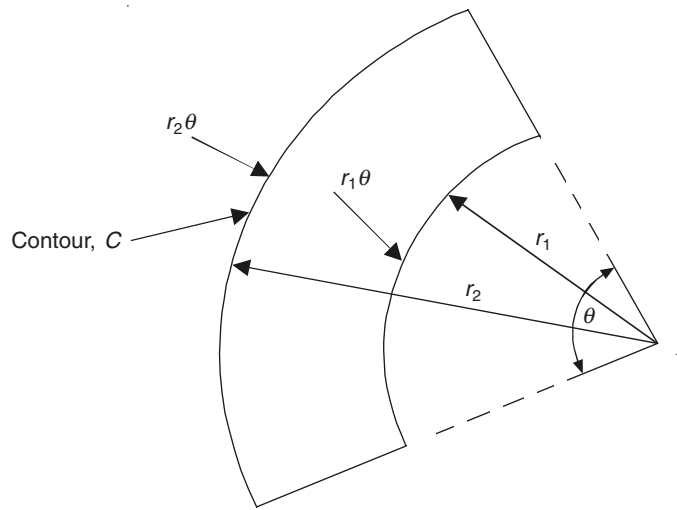
Figure 7.15 A contour not enclosing the current filament.
