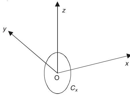
Figure 12.3 Loop for Ampere's law.
