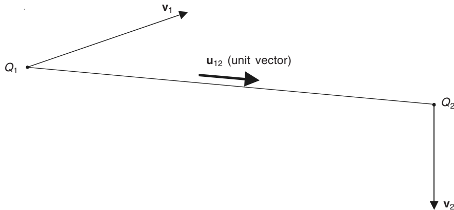
Figure 7.1 Two moving point charges.
