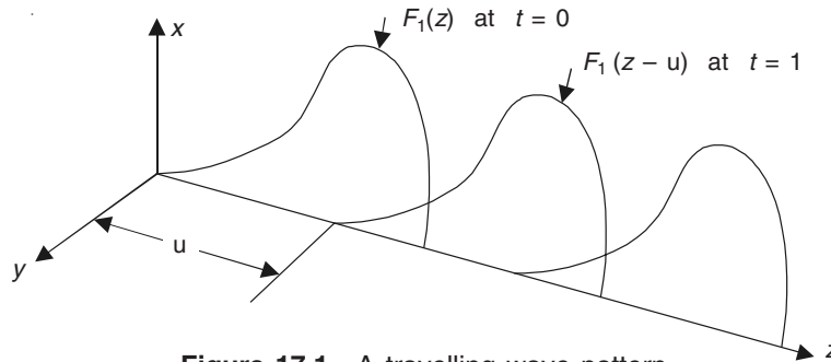
Figure 17.1 A travelling wave pattern.
