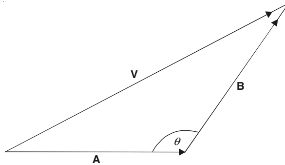
Figure 0.1 Vector addition.
