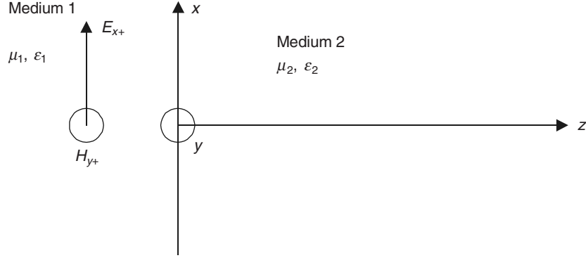
Figure 17.9 A plane wave incident on a dielectric interface.
