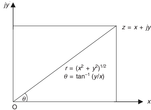
Figure 4.9 Point z = x + jy in the complex plane ( r is the modulus and \theta the argument of the complex number z ).
