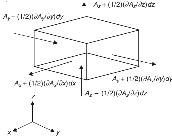
Figure 0.14 Divergence of a vector point function.
