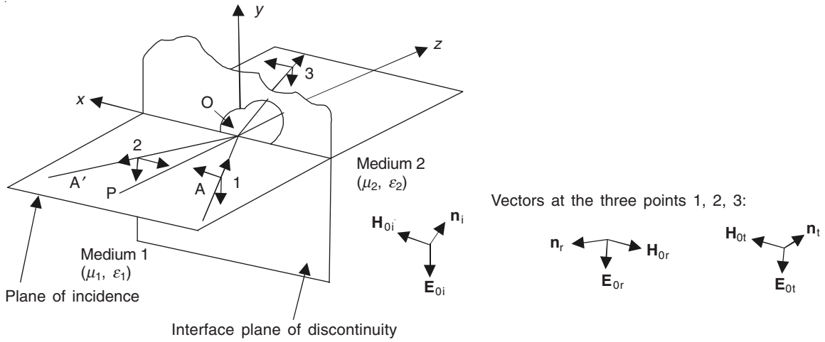
Figure 17.14 The incident, reflected and transmitted waves, when the incident wave has its \mathbf{E} wave polarized normal to the plane of incidence.
