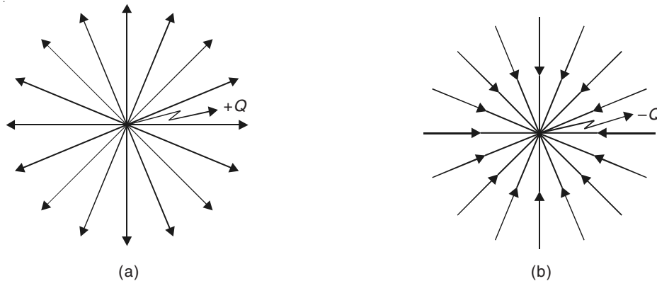
Figure 1.3 Graphical representation of electric lines of force of a point charge (a) +Q , (b) -Q , each in isolation.
