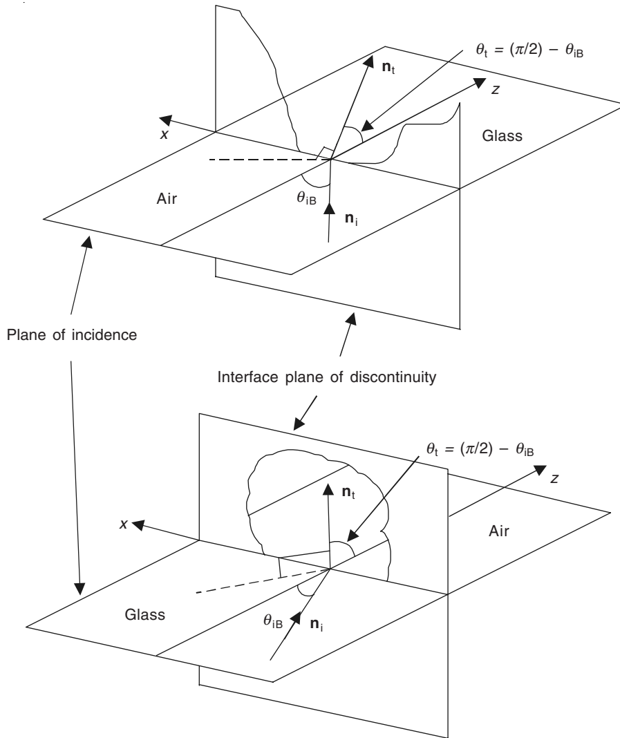
Figure 17.19 Brewster angle for air to glass and for glass to air.
