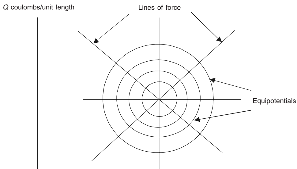
Figure A.1.1(a) Electric field of a straight, infinitely long line charge.
