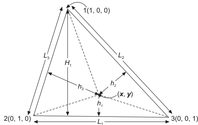
Figure 21.21 Triangular element with its shape function dimensions.
