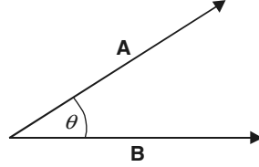
Figure 0.3 Scalar product of the vectors \mathbf{A} and \mathbf{B} .
