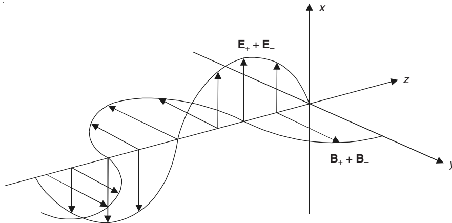
Figure 17.8 Standing wave patterns for \mathbf{E} and \mathbf{B} .
