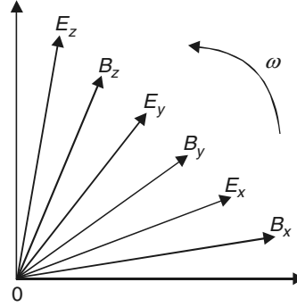
Figure 0.17 Complex plane representation of 'rotating vector'. The figure shows the reference component, or the real parts of the three-dimensional Cartesian components of the \mathbf{E} and \mathbf{B} vector at a particular point in space.
