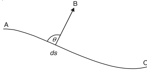
Figure 0.10 Line integral for a vector function.
