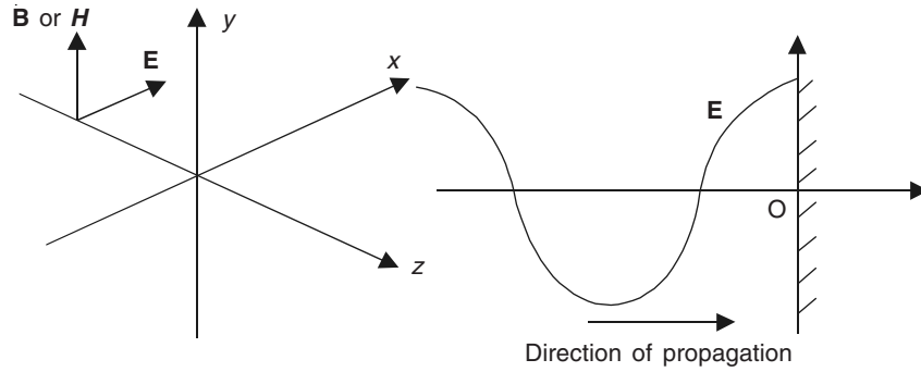
Figure 17.7 Incident E wave meeting z = 0 perfectly conducting surface, normally.
