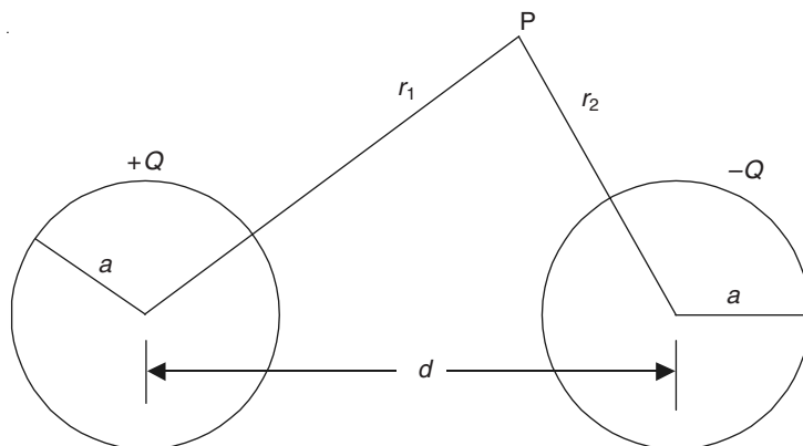
Figure 2.12 Two spheres of equal diameters.
