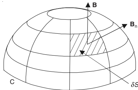
Figure 10.20 Open surface S .
