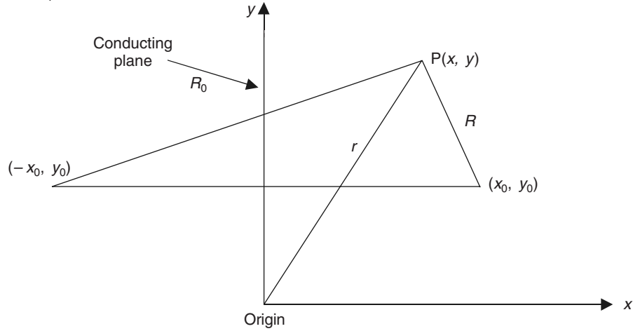
Figure 4.7 Line charge in front of a conducting plane.
