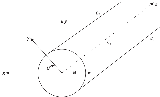
Figure 18.21 Circular dielectric waveguide.
