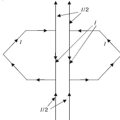
Figure 9.20 Image of a full-pitched coil-end in an infinitely permeable iron-block with finite-length air-gap.
