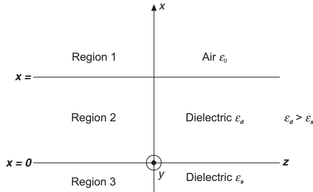
Figure 18.21 Dielectric slab waveguide.
