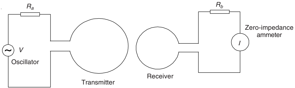
Figure 19.18 A pair of loop antennae. The one on the left (transmitter) is excited by an oscillator, supplying a voltage V . The other (receiver) is connected to a load resistance R_b through a zero-impedance ammeter, measuring the current I .
