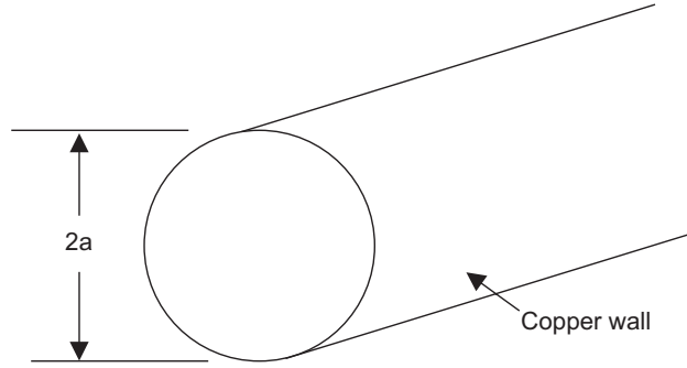
Figure 18.17 A cylindrical waveguide.
