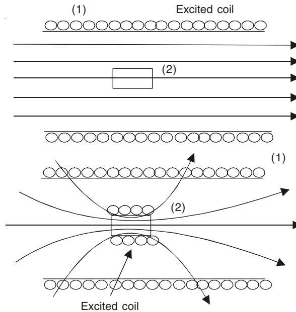
Figure 10.14 A short coil inside a long coil, for the equivalence of M_{12} and M_{21} .
