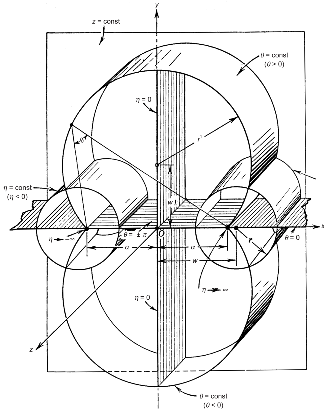
Figure A.10.2 Bicycylindrical coordinates. The surfaces \eta = \text{const} are circular cylinders with axes in the xz -plane, surfaces \theta = \text{const} are portions of circular cylinders with axes in the yz -plane, surfaces z = \text{const} are parallel planes.
