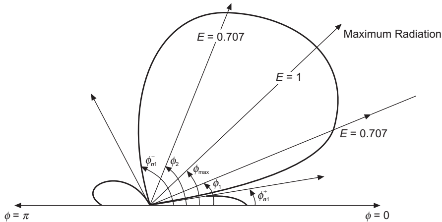
Figure 19.14(b) Half-power beam-width of a radiation pattern.
