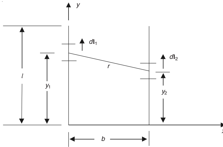
Figure 13.10 Parallel conductors of length l .
