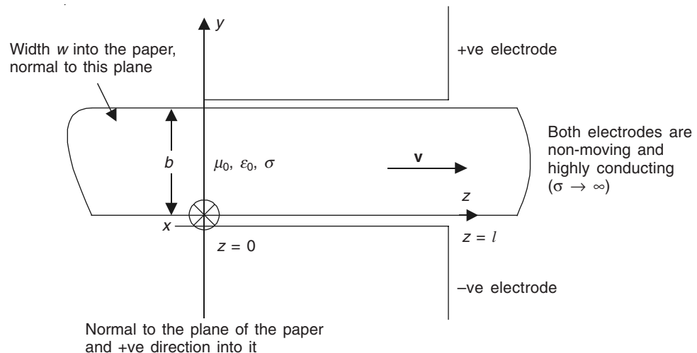
Figure 15.19 Geometry for diffusion in presence of steady motion only.
