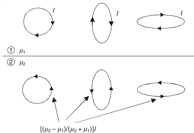
Figure 9.10 Images of current loops.
