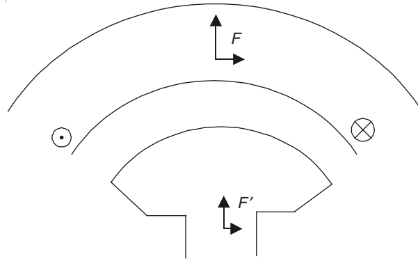
Figure 20.13 Stator and rotor of an alternator to explain the concept of a moving field.
