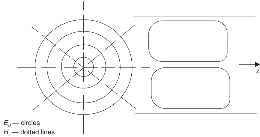
Figure 18.18 Field pattern for circular waveguide when n = 0 .
