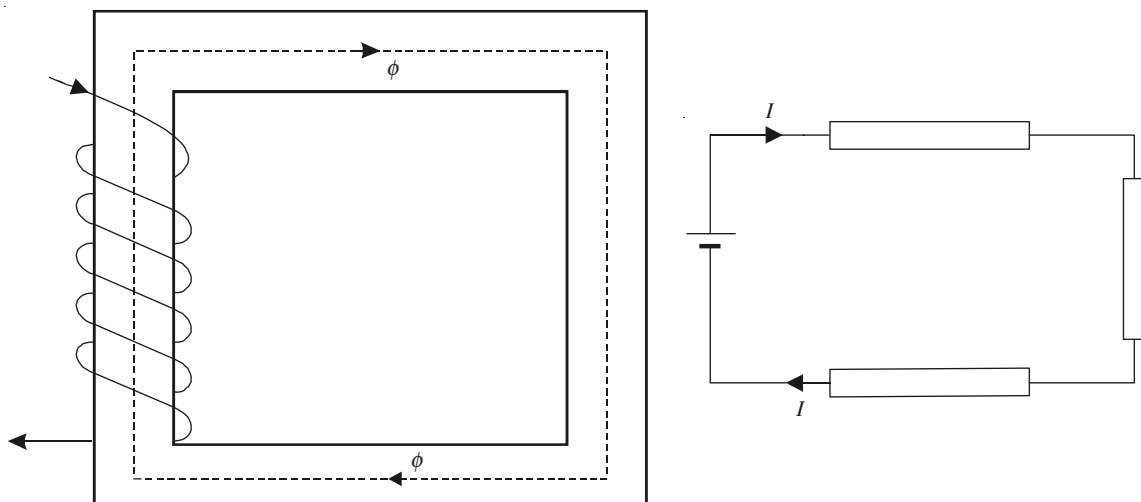
Figure 8.14 Analogy between magnetic circuit and current circuit.
