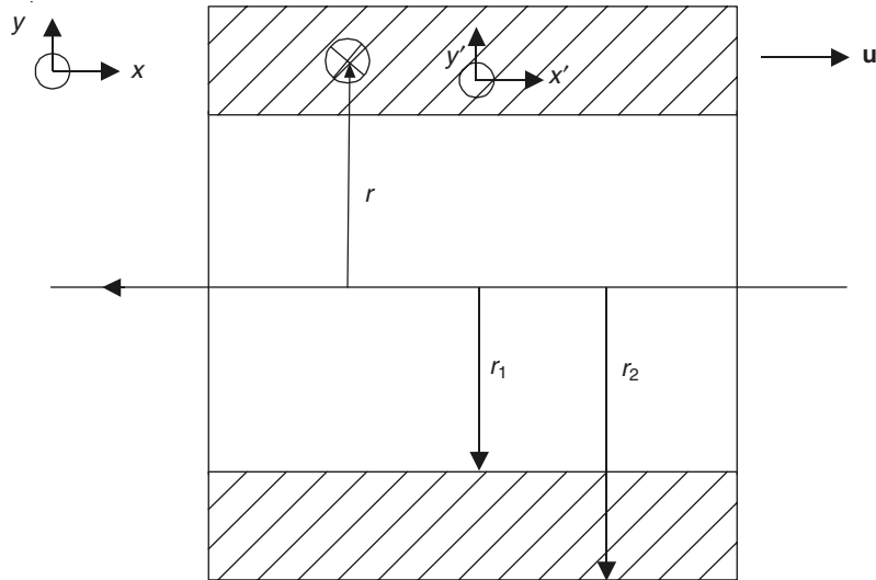
Figure 20.20 The Cullwick experiment, showing the frames of reference.
