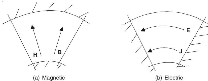
Figure 9.26 Magnetic field problem and its electric analogue ( / / / indicates equipotentials).
