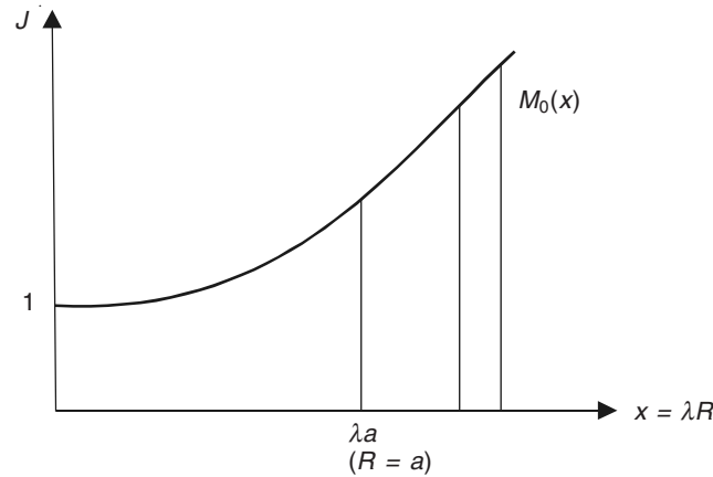
Figure 15.11 Current density amplitude as a function of radius R of the conductor.
