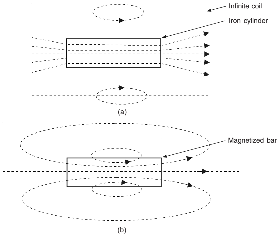
Figure 8.9 (a) B field of an iron cylinder inside a solenoid and (b) B field of the magnetized bar.
