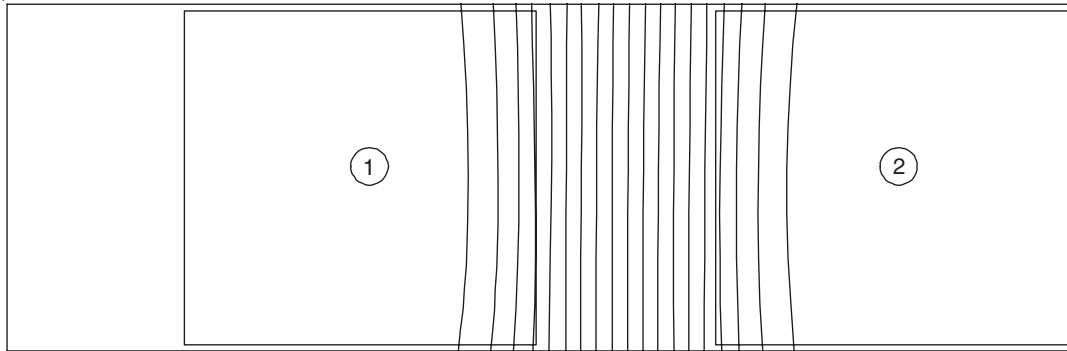
Figure 21.4 Conductor in a slot with eddy currents—FEM solution—analysis in x-y coordinates at t = 0 .
