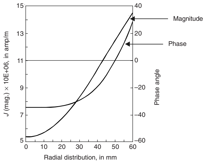
Figure 21.1 Current density distribution inside a circular conductor.
