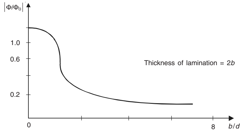
Figure 15.7 Penetration of \Phi as a function of b .
