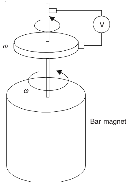
Figure 20.15 Faraday's disc with rotating cylindrical bar magnet.
