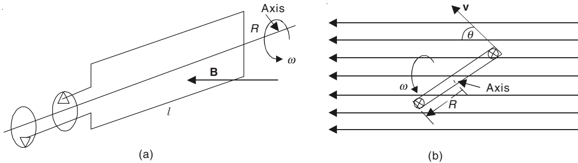
Figure 10.29 A simple AC generator: (a) perspective view and (b) cross-section perpendicular to the axis.
