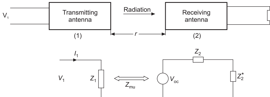
Figure 19.17(c) Transmitting and receiving antennae system.
