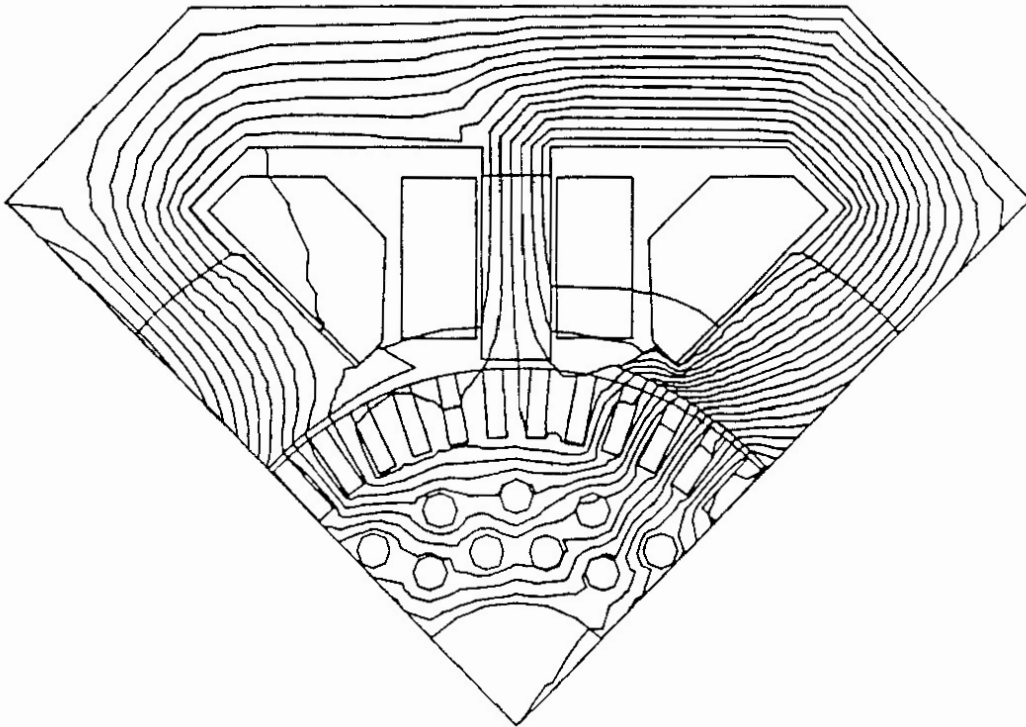
Figure 21.12 DC machine—flux distribution on 200% load.
