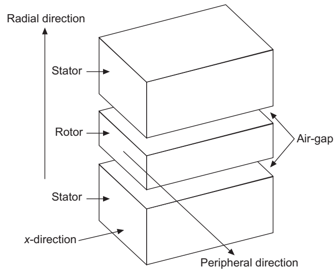
Figure 22.16 Schematic of a double-sided flat linear machine.
