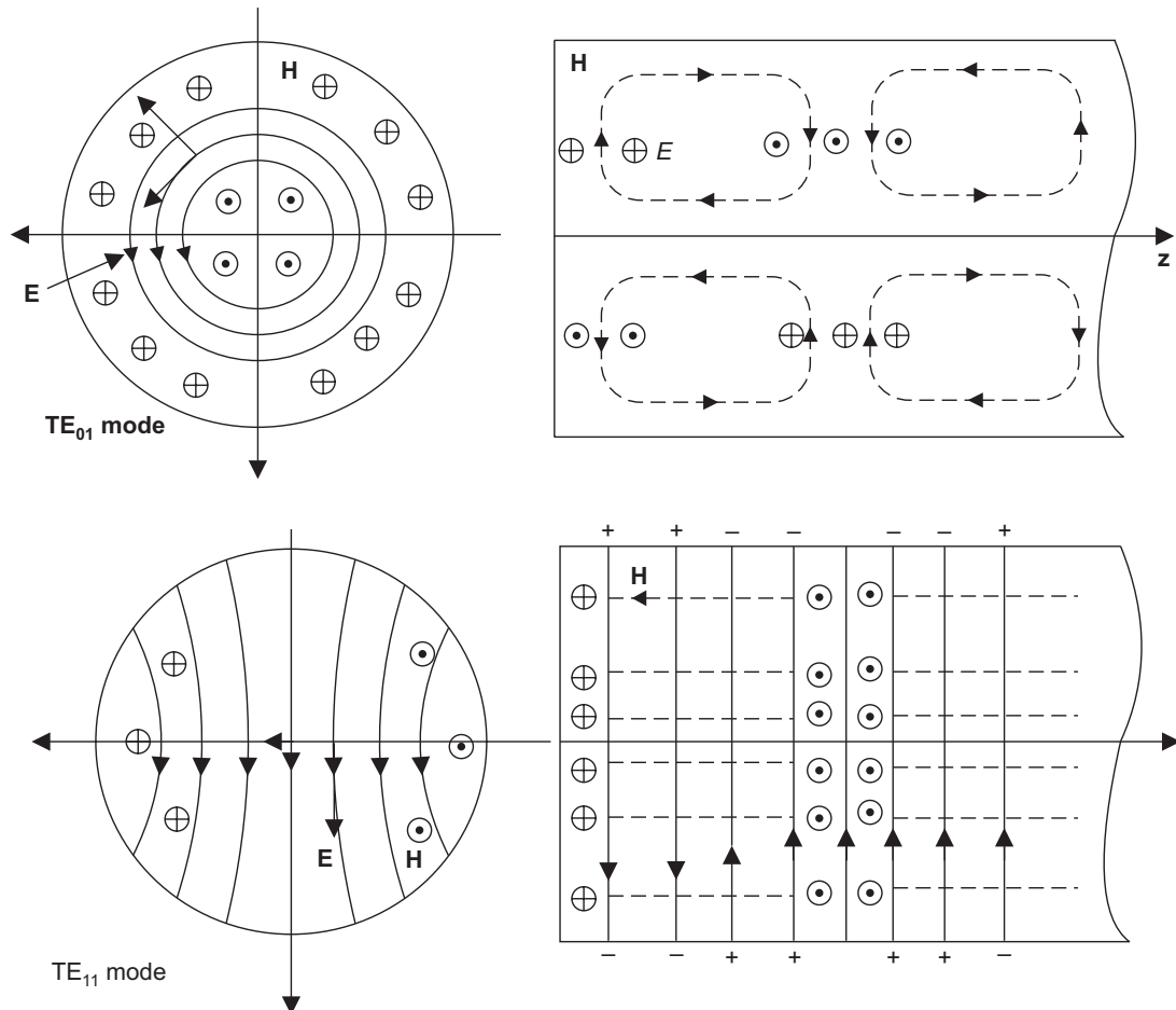
Figure 18.20 TE_{01} and TE_{11} modes in a circular waveguide.
