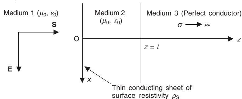
Figure 17.11 A plane wave normally incident on a thin conducting sheet, placed in front of a perfectly conducting plane.
