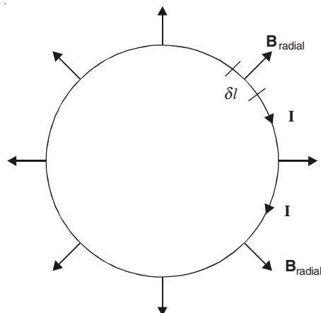
Figure 11.9 Effect of the radial component of \mathbf{B} on the circular coil-turn.
