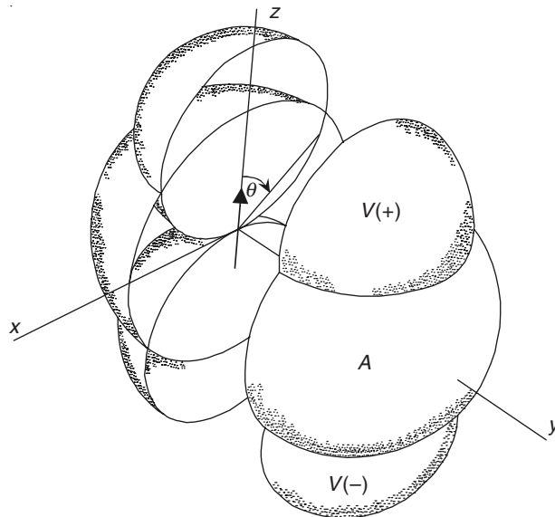
Figure 19.5 The scalar potential V and the magnitude of the magnetic vector potential, i.e. |\mathbf{A}| , shown as functions of \theta and \phi about the dipole oriented as shown.
