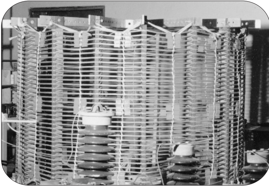
Plate 1 A view of the reactor subjected to high current short-circuit test.
