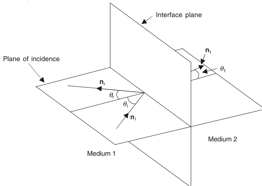
Figure 17.6 An electromagnetic wave in medium 1, incident on the interface between media 1 and 2, giving rise to both the reflected wave in the medium 1 and the transmitted wave in the medium 2.
