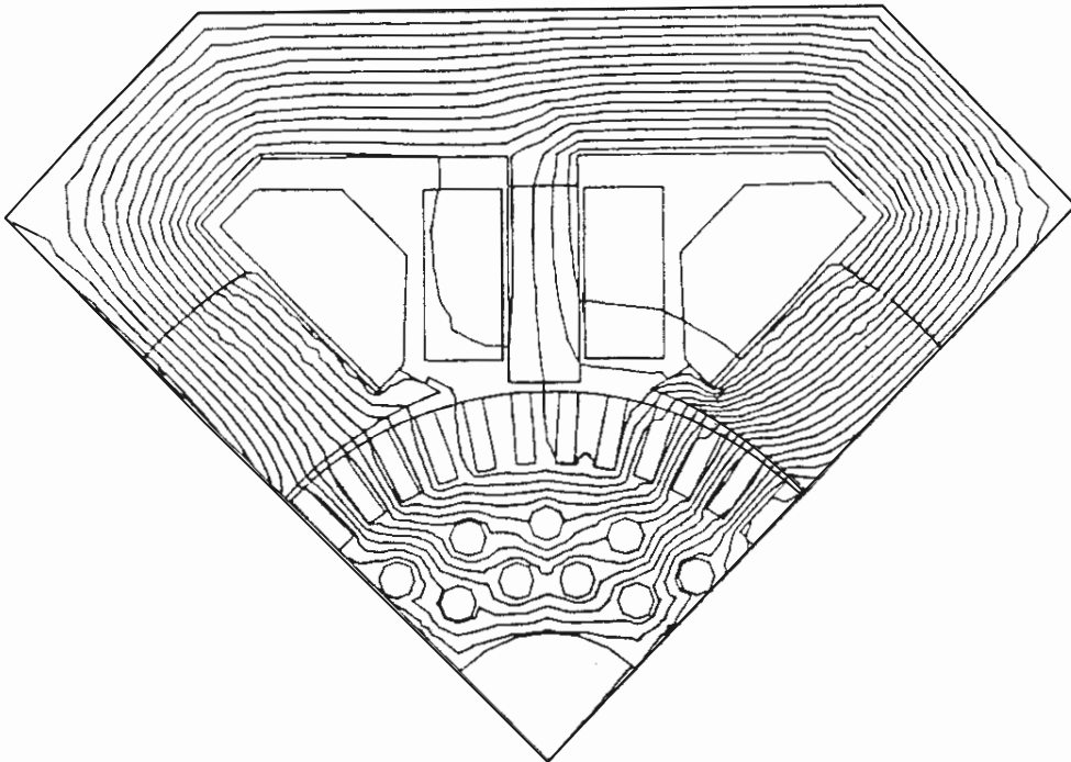
Figure 21.11 DC machine—flux distribution on 100% load.
