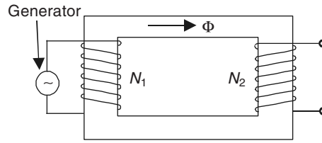
Figure 10.8 A schematic representation of a single-phase two-limb two-winding transformer.
