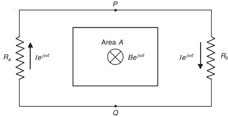
Figure A.6.2 Cross-section of the magnetic flux area within the circulating current circuit.
