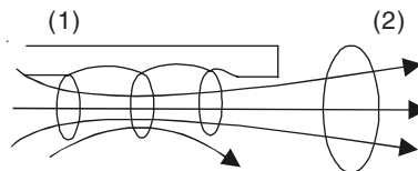
Figure 10.12 Mutual inductance between two circuits.
