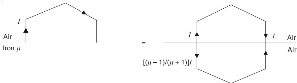
Figure 9.14 Incorrect image of the partially embedded coil, in the air-region.
