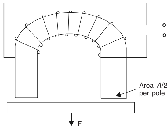
Figure 11.17 U-shaped electromagnet.
