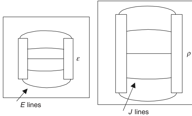
Figure 6.4 Current-flow analogue (either conducting paper or electrolytic tank).
