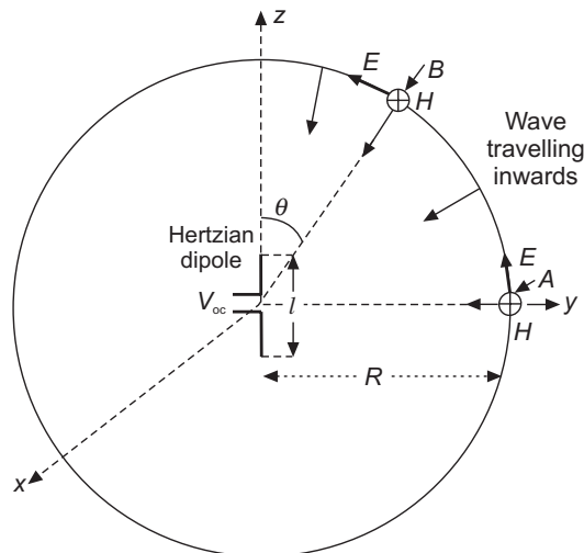
Figure 19.17(c) Hertzian dipole as a receiving antenna.
