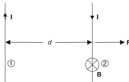
Figure 11.6 Parallel go-and-return circuit.
