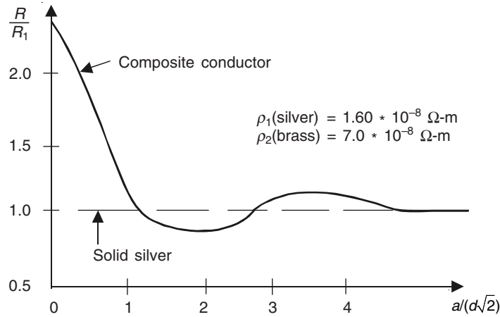
Figure 15.14 Resistance ratio for a silver-plated brass block.
