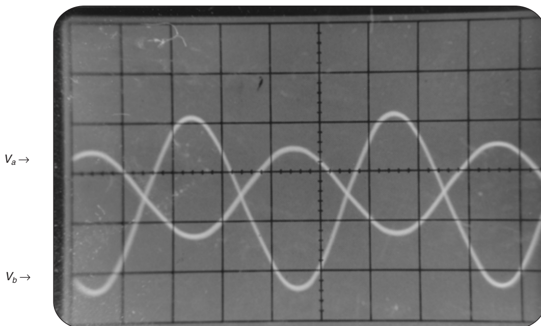
Plate 5 Wave shapes of V_a and V_b from the demonstration experiment (Plate 4) as observed on the CRO screen.
