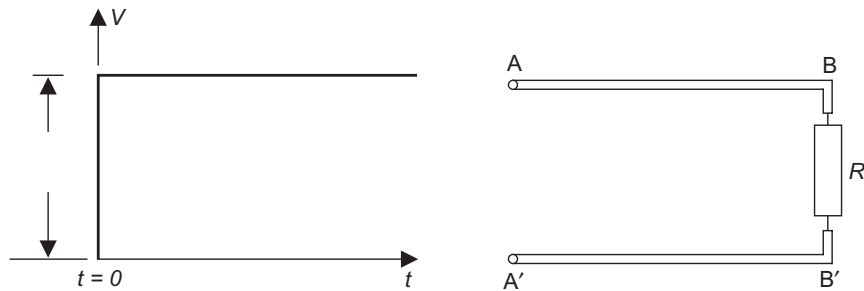
Figure 18.2 A unit-step function of voltage applied to the end AA' of a transmission line whose other end BB' has been terminated by a resistance R .
