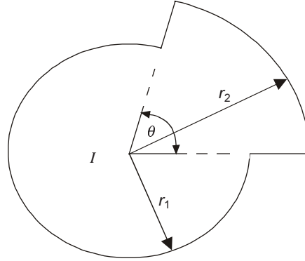
Figure 7.14 First step of the generalized contour of \mathbf{H} \cdot d\mathbf{l} in the plane normal to the current filament.
