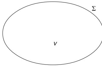
Figure 12.1 A closed surface with space charge of density \rho_C .
