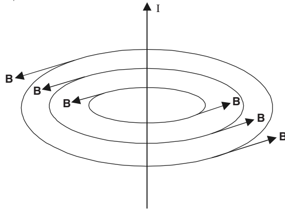
Figure 7.11 Lines of \mathbf{B} for a straight current filament.
