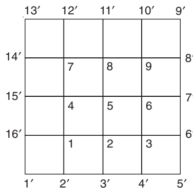
Figure 5.10 Poissonian field region.
