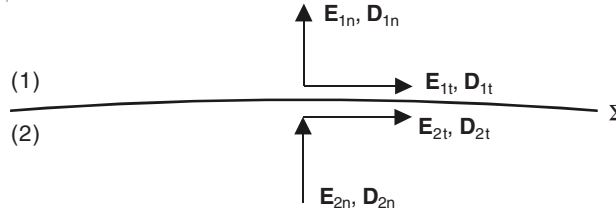
Figure 12.10 Dielectric discontinuity.
