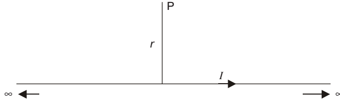
Figure 7.13 An infinitely long conductor carrying current I .
