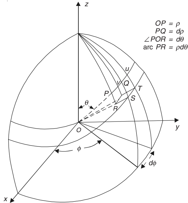
Figure A.4.5 Spherical polar coordinate system (showing the details of the volume elements).
