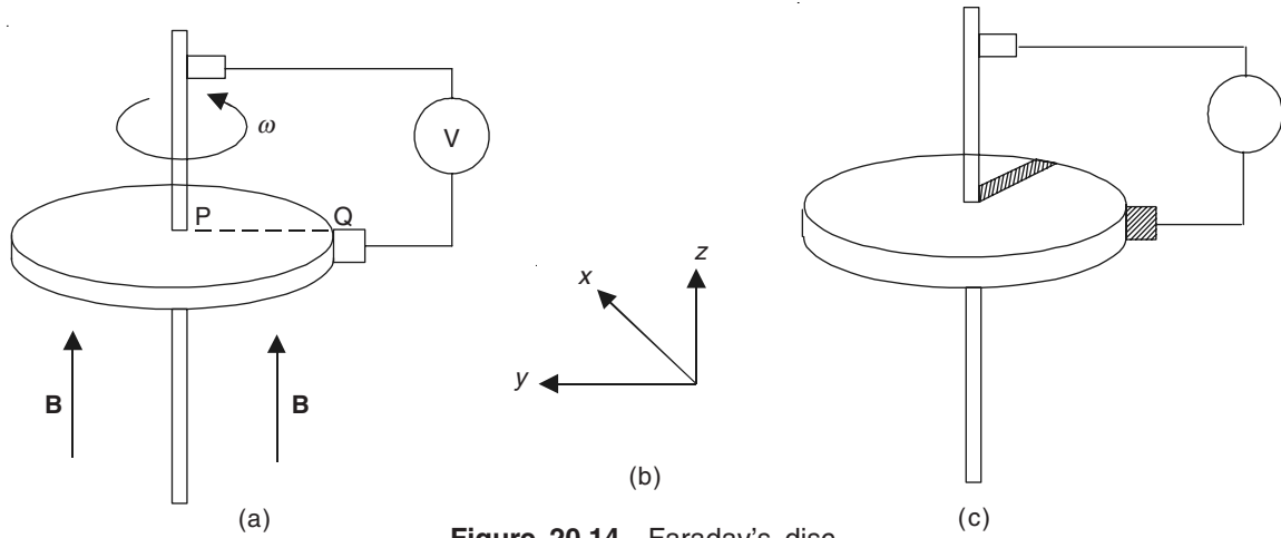
Figure 20.14 Faraday's disc.
