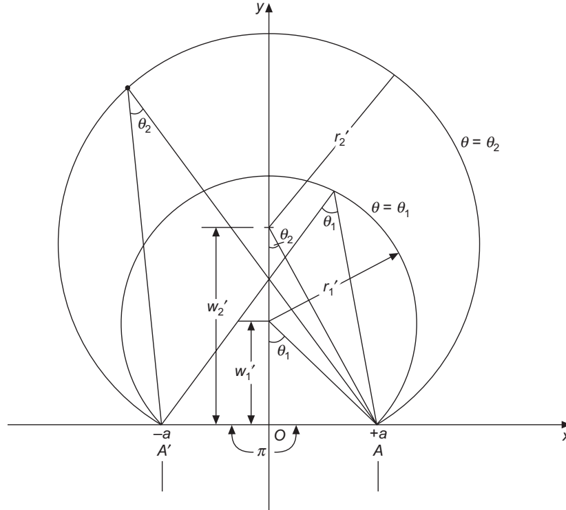
Figure A.10.4 Relationship for (\theta = \text{constant}) circles.
