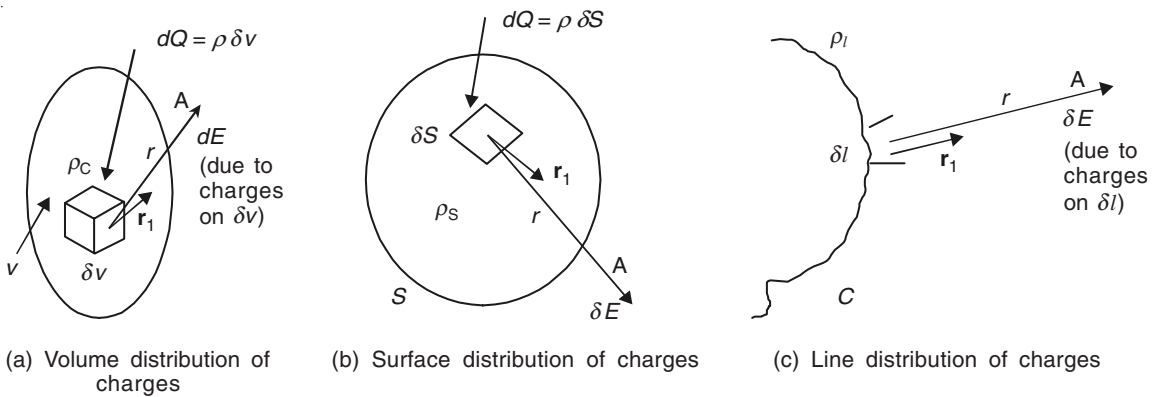
Figure 1.4 Distribution of charges.
