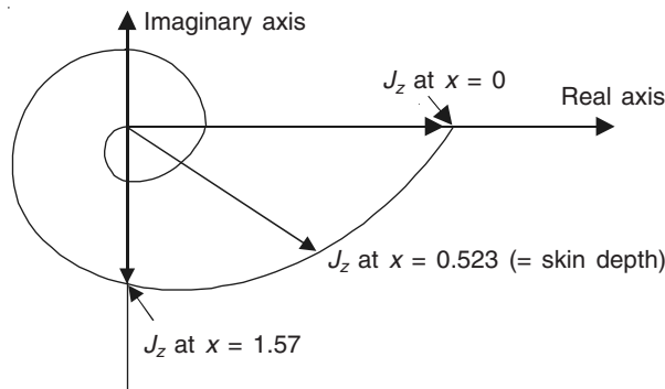
Figure 15.3 Complex plane diagram for J_z at various distances x from the surface of the semi-infinite metal block.
