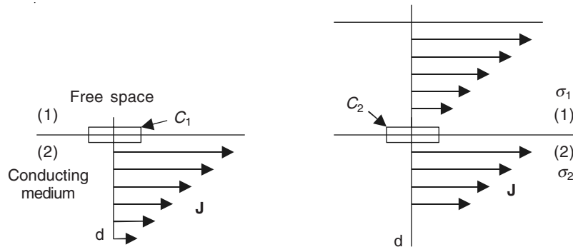
Figure 12.11 Alternating current distributions in conducting media, and interface conditions.
