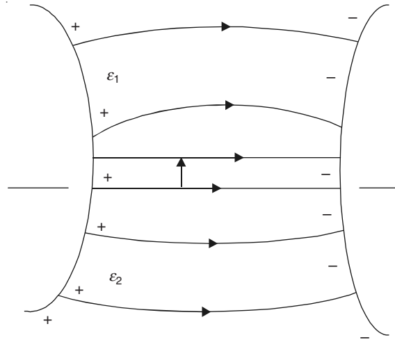
Figure 3.5 An interface between two dielectrics parallel to the \mathbf{E} vector.
