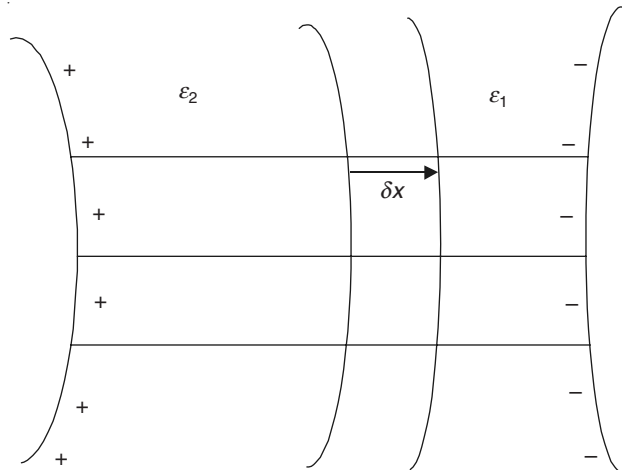
Figure 3.6 An interface between two dielectrics perpendicular to the \mathbf{E} vector.
