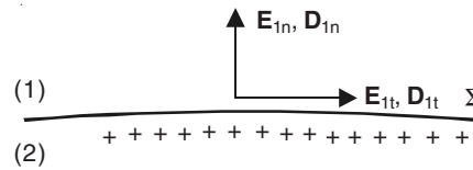
Figure 12.9 Static charge density on the surface of a perfect conductor.
