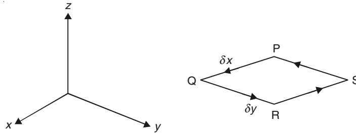
Figure 0.16 Contour for the line integral for deriving the curl.
