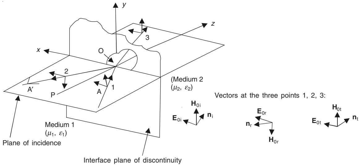
Figure 17.15 The incident, reflected, and transmitted waves, when the incident wave has its \mathbf{E} wave polarized in the plane of incidence.
