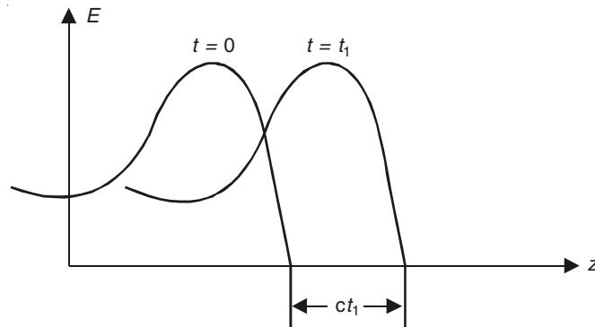
Figure 12.5 A travelling wave pattern.
