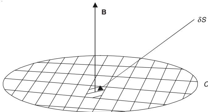
Figure 13.1 A closed contour in a magnetic field \mathbf{B} .
