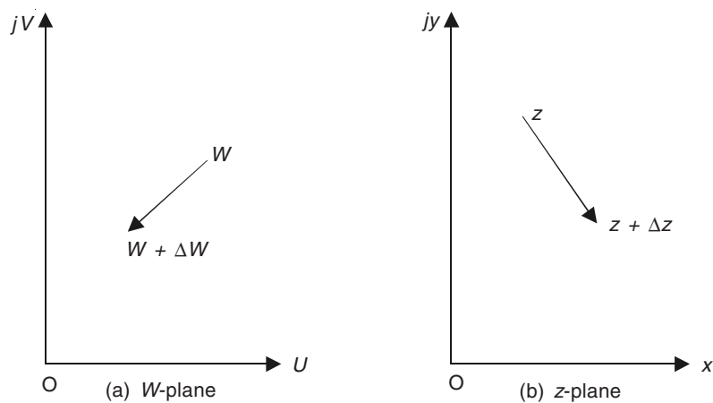
Figure 4.10 The function W(z) = U(x, y) + jV(x, y) in the W -plane and the derivative ( dW/dz ) from the changes in W and z .
