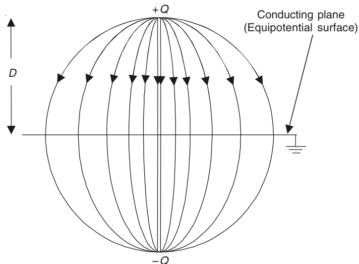
Figure 4.19 Image charge of the point charge Q near a plane conducting surface.
