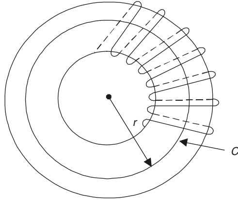
Figure 7.27 Toroidal solenoid.
