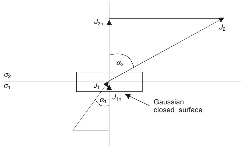
Figure 6.6 Conductor interface.
