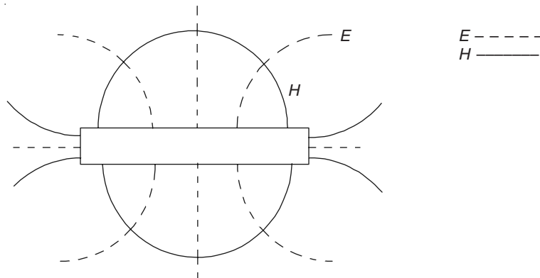
Figure 14.9 An electrically charged magnet.
