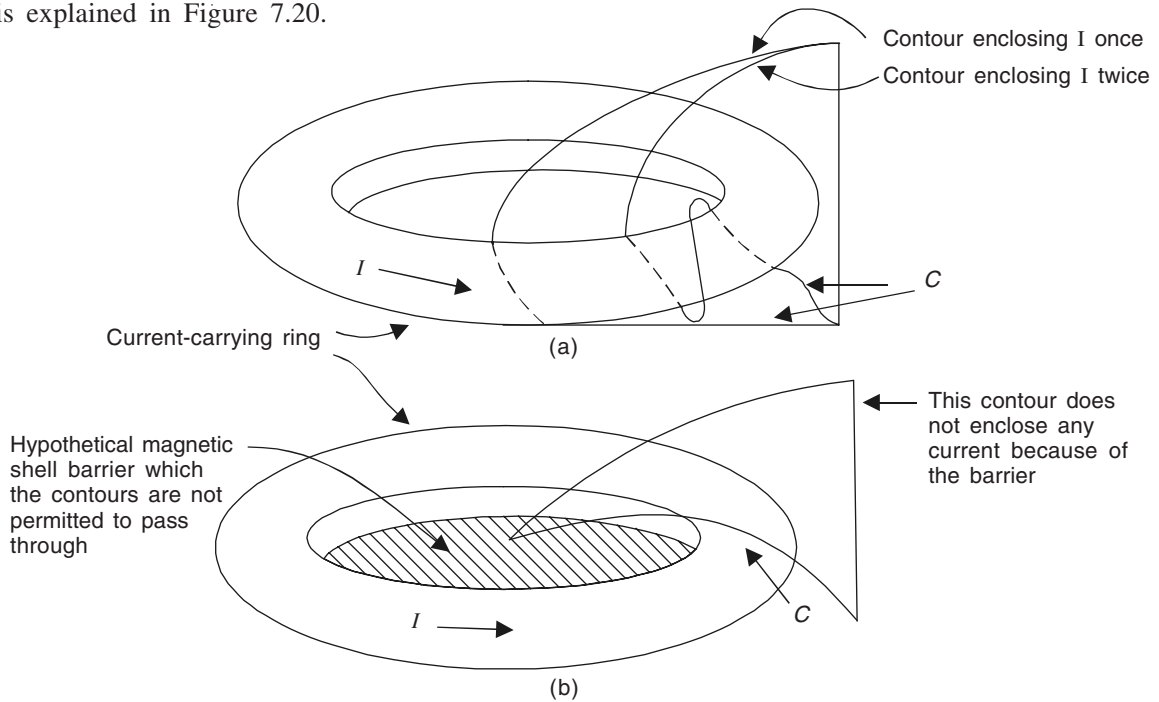
Figure 7.20 (a) Multivaluedness of (\mathbf{H} \cdot d\mathbf{l}) and \Omega ; (b) magnetic barrier to avoid the multivalued nature of (\mathbf{H} \cdot d\mathbf{l}) and \Omega .
