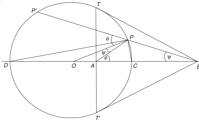
Figure A.2.1 Inverse points of a circle and the relevant angles.
