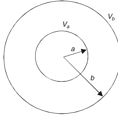
Figure 2.20 Concentric spheres.
