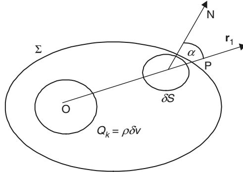
Figure 1.6 Construction for Gauss' theorem.
