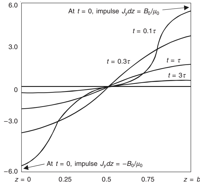
Figure 15.18 Current distribution in one-dimension diffusion.
