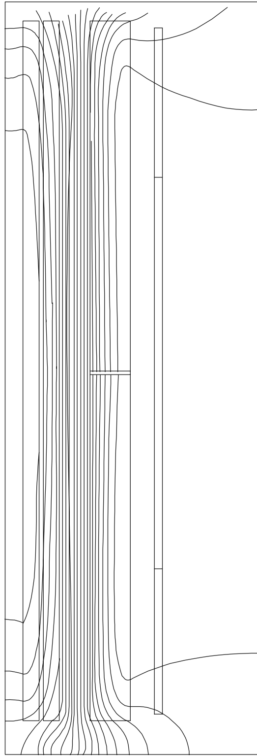
Figure 21.9 250 MVA 220 kV generator transformer—orthogonal section—analysis in r - z coordinates.
