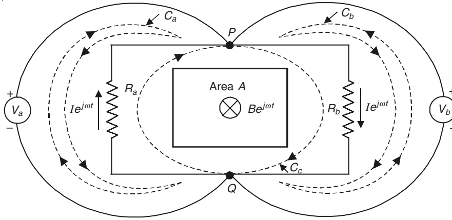
Figure A.6.3 Circulating current circuit with measuring voltmeters, and showing the contours for integration.
