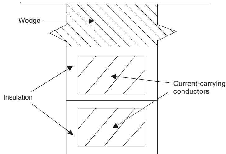
Figure 11.6(a) Stator slot of a turbogenerator.
