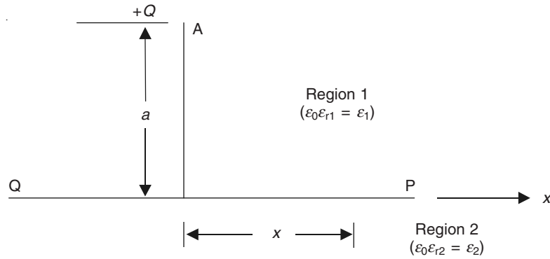
Figure 4.17 A line charge in front of a semi-infinite dielectric block.
