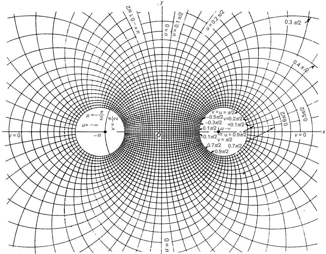
Figure A.10.1 Bipolar coordinates obtained by the transformation z^* = \frac{a(e^w + 1)}{e^w - 1} and inversion of polar coordinates.
