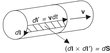
Figure 10.6 Geometry for the law of induction applied to a moving conductor.
