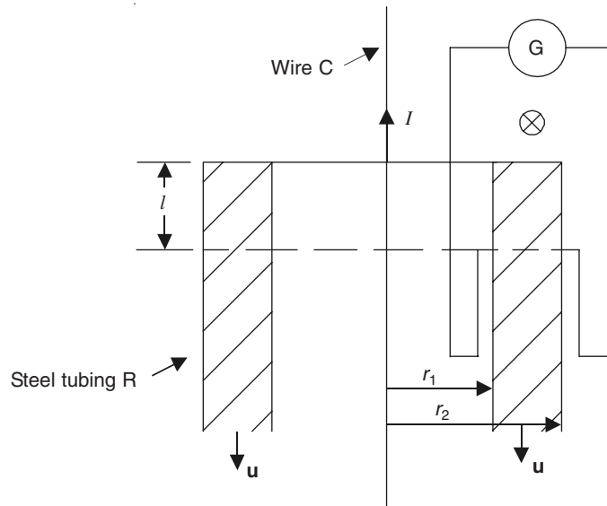
Figure 20.19 The Cullwick experiment.
