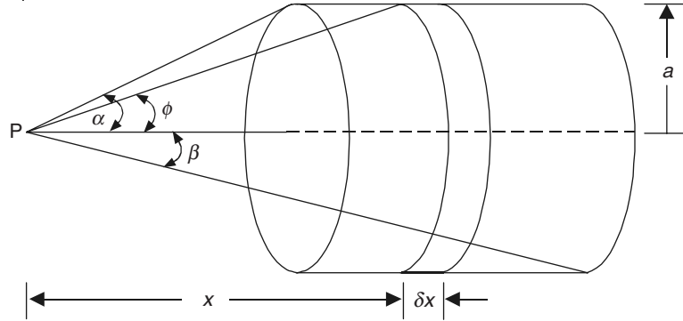
Figure 7.9 A circular solenoid of finite axial length.
