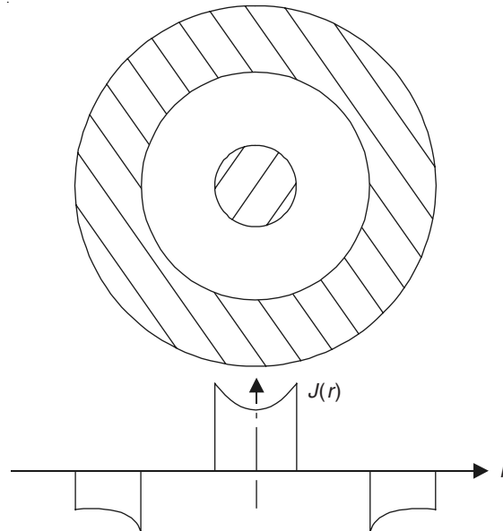
Figure 15.28 Proximity effect in a coaxial cable.
