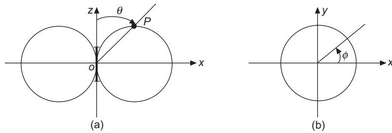
Figure 19.10(a) and (b) Field patterns of the Hertzian dipole: (a) normalized E -plane, \phi = 0 ; (b) normalized H -plane, \theta = \pi/2 .
