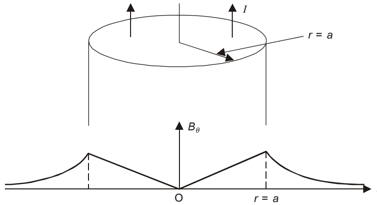
Figure 7.23 B due to a long straight current-carrying conductor.
