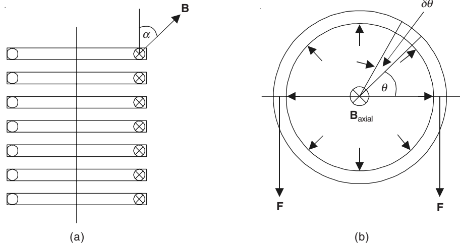
Figure 11.8 Forces between the turns of a multiturn coil.
