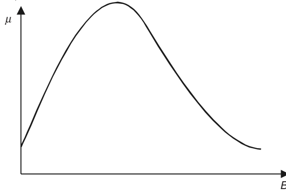
Figure 8.12 \mu as a function of B for iron.
