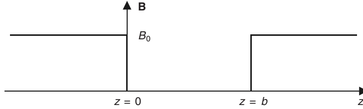
Figure 15.16 Distribution of B_x at t = 0^+ in the conducting slab.
