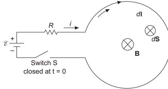
Figure A.6.8 Single-turn loop circuit.
