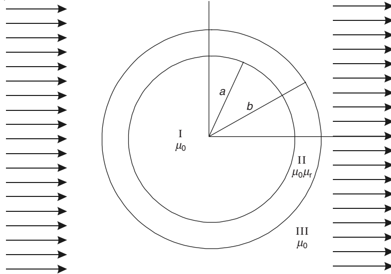
Figure 9.1 Hollow magnetic cylinder in a homogeneous magnetic field.
