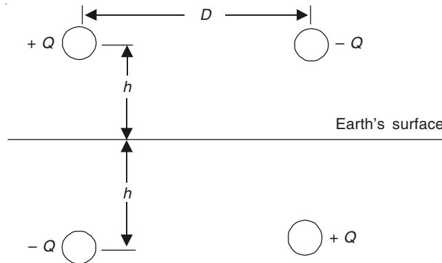
Figure 4.21 Two-wire transmission line parallel to the earth's surface and its image.
