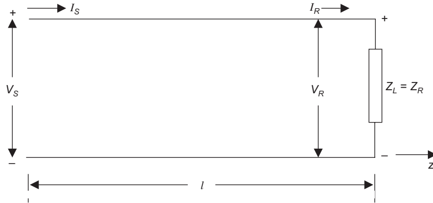
Figure 18.7 Transmission line terminated with a load impedance ( Z_L = Z_R ) at the receiving end.
