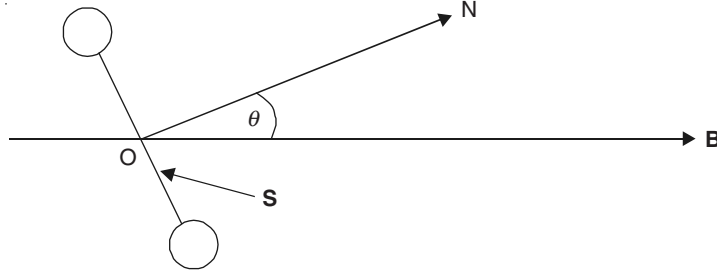
Figure 11.1 A circular coil in a magnetic field.
