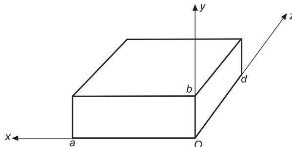
Figure 18.22 A rectangular resonant cavity.
