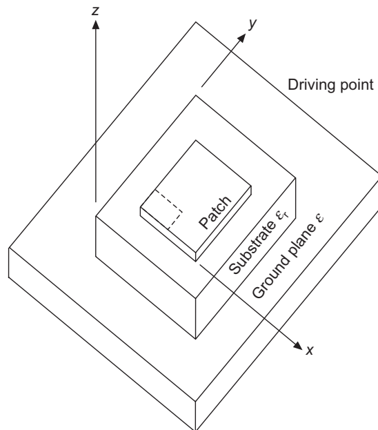
Figure 22.21 Rectangular microstrip antenna. Patch geometry is shown to be rectangular here, though it can be of any shape. The feed point is located at a point which is chosen to match the antenna with a desired impedance.
