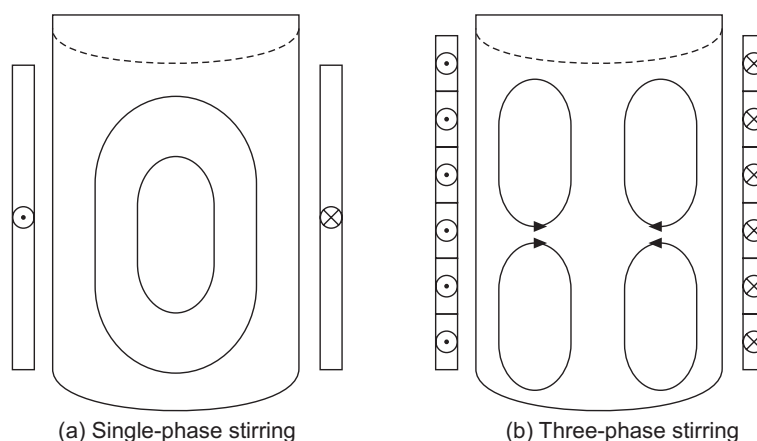
Figure 22.19 Induction stirring action in molten metal.
