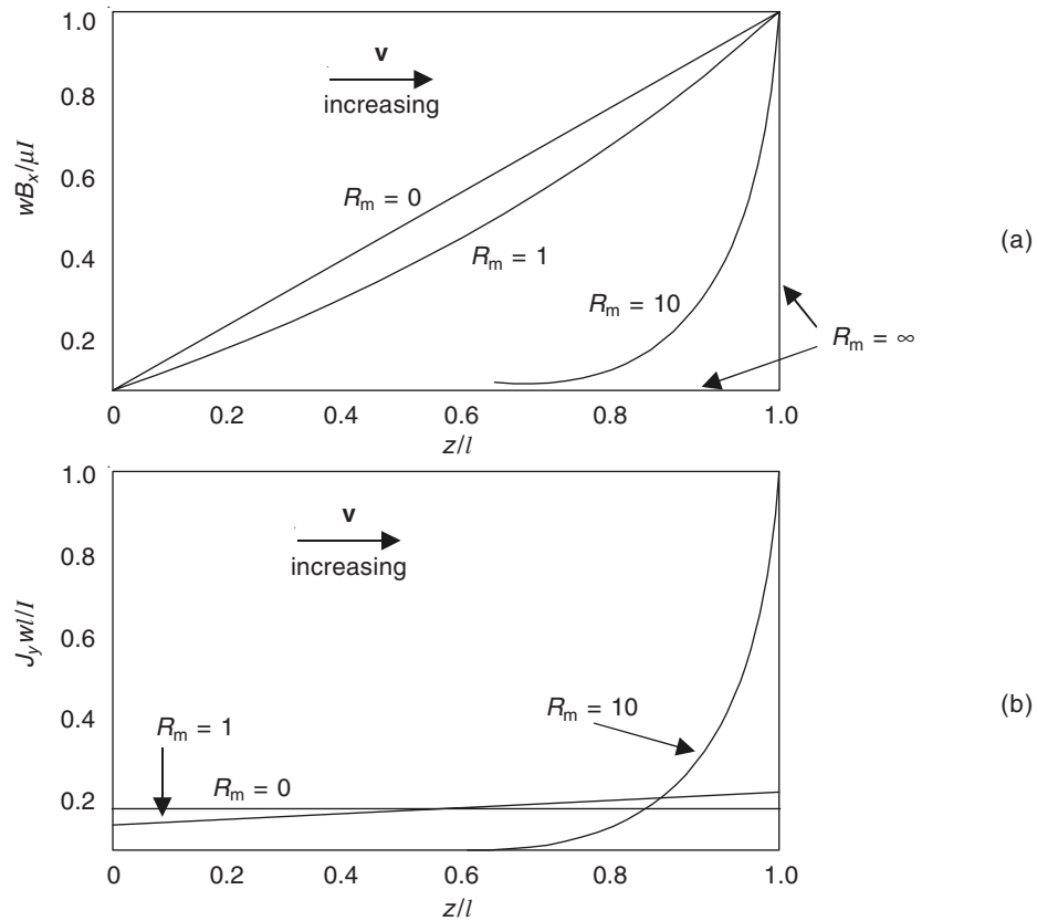
Figure 15.20 B and J distributions in the system of Figure 15.19 as functions of z and R_m : (a) B_x distribution and (b) J_y distribution.
