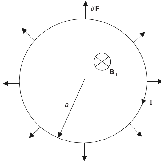
Figure 8.1 The total force on a closed current loop in a uniform magnetic field is zero.
