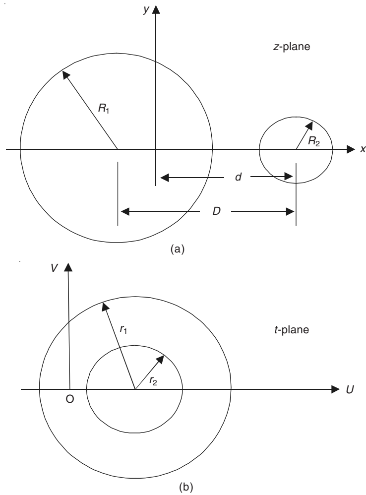
Figure 4.14 Z-plane to t -plane transformation of the two-cylinder problem.
