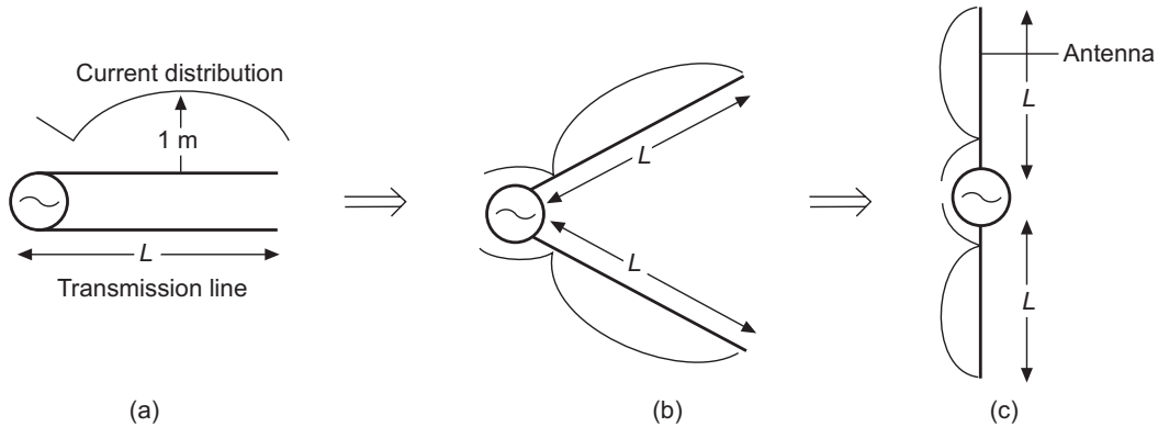
Figure 19.7(b) A dipole antenna as a flared version of a transmission line.
