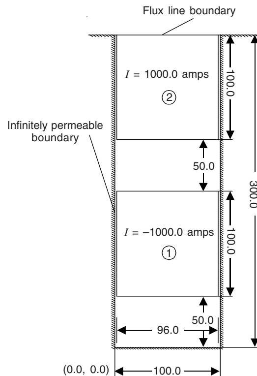
Figure 21.2 Conductors in a slot.
