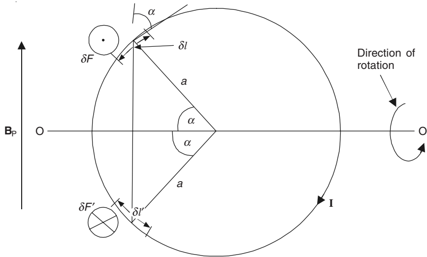
Figure 8.2 Torque of the magnetic forces on the closed current loop.
