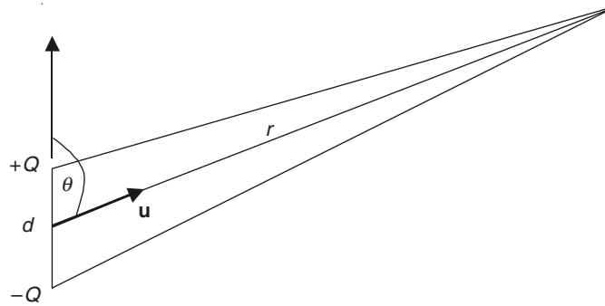
Figure 2.3 An electric dipole.
