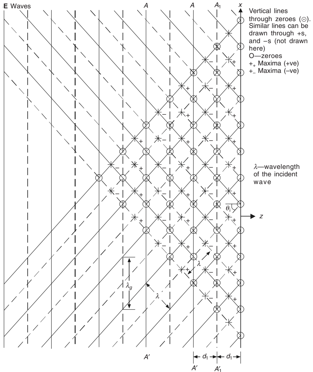
Figure 17.24 Resultant E wave pattern, when the incident E wave, normal to the plane of incidence, meets a perfectly conducting surface obliquely.
