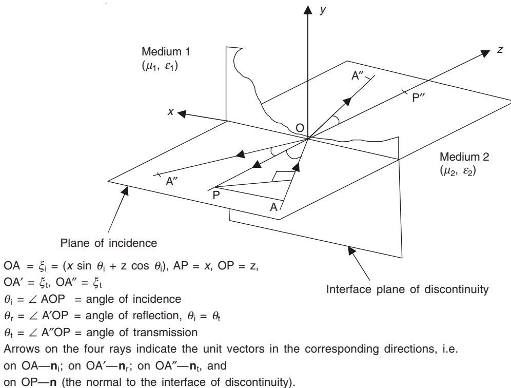
Figure 17.13 Coordinate system used for reflection and refraction of waves.
