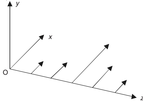
Figure 12.4 A uniform plane wave.
