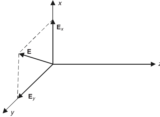
Figure 17.4 Resolution of \mathbf{E} into two orthogonal components.
