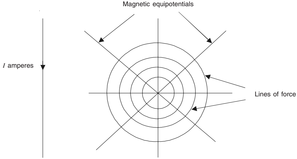
Figure A.1.1(b) Magnetic field of a straight line current.
