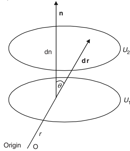
Figure 0.12 Gradient of a scalar.
