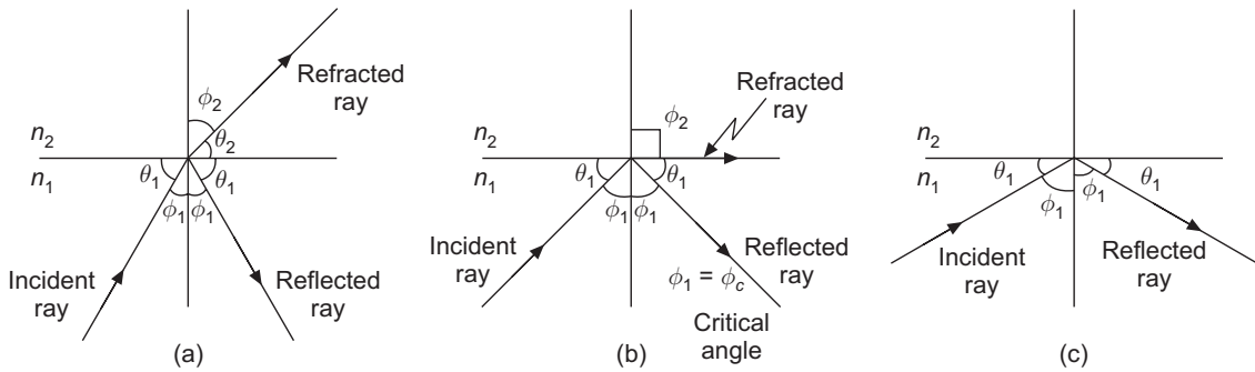
Figure 22.9 Total internal reflection, n_1 > n_2 : (a) \phi_1 < \phi_c ; (b) \phi_1 = \phi_c ; (c) \phi_1 > \phi_c
