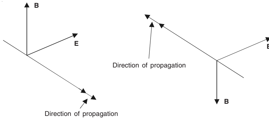
Figure 12.6 Direction of propagation of \mathbf{E} and \mathbf{B} (or \mathbf{H} ) waves.
