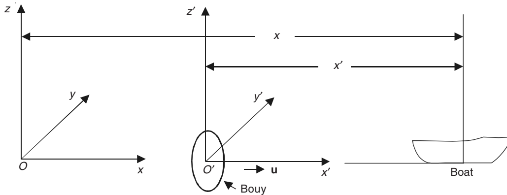
Figure 20.1 Coordinate systems S and S' .
