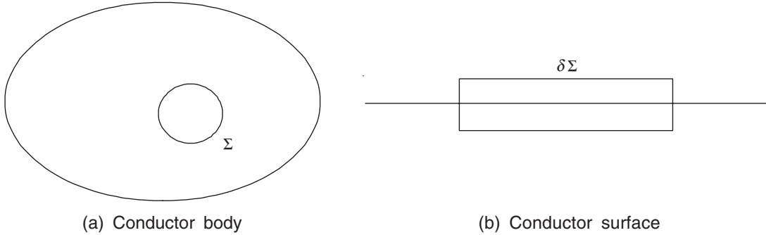
Figure 2.1 Gaussian surfaces inside and on the surface of a conducting body.
