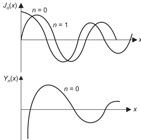
Figure 18.15 Approximate plots of J_n(x) and Y_n(x) .
