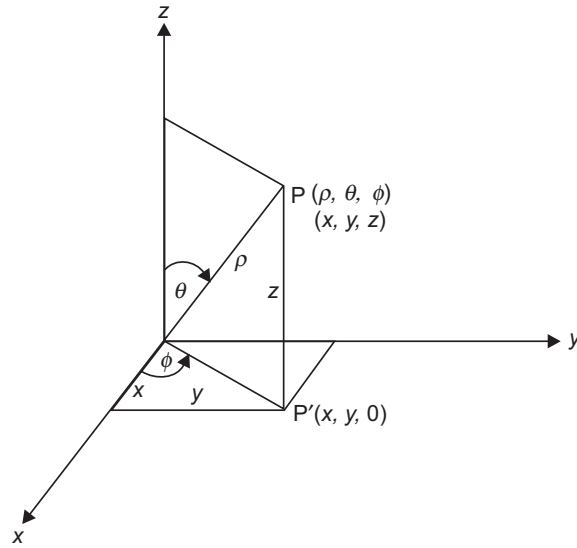
Figure 0.8 Spherical polar coordinate system.
