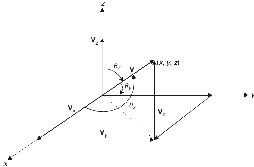
Figure 0.2 Orthogonal components of a vector.
