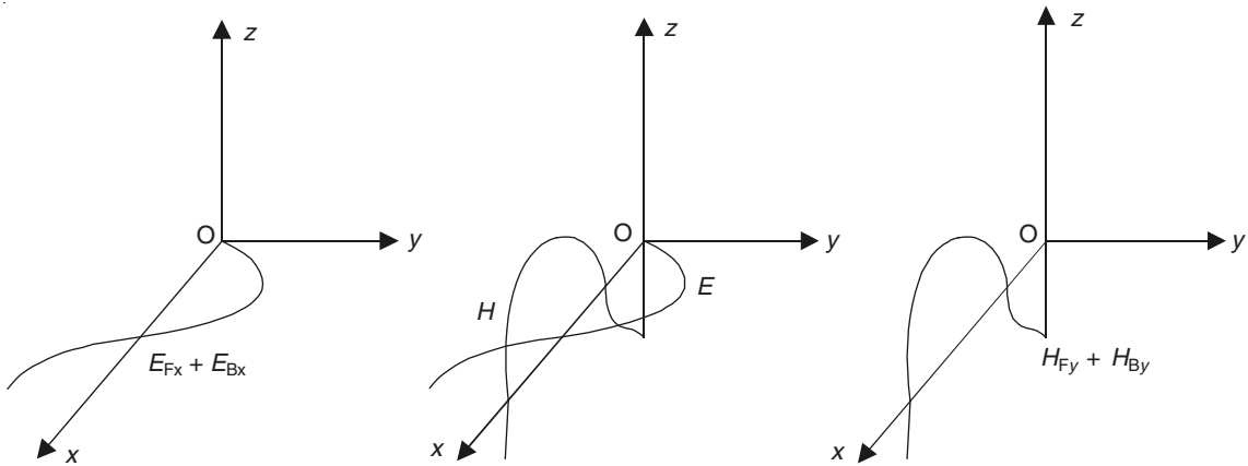
Figure 17.2 Standing wave patterns.
