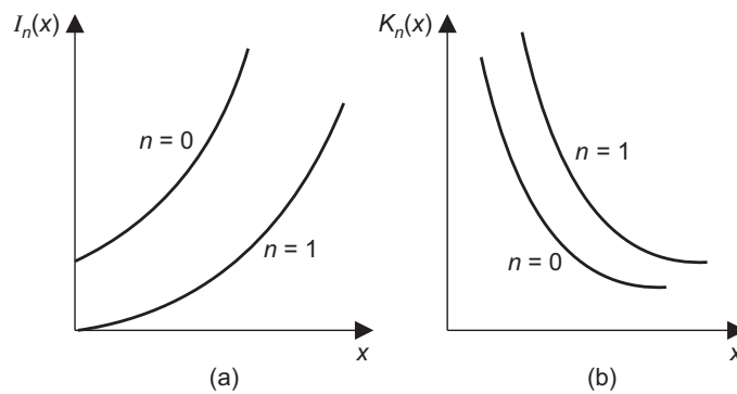
Figure 18.16 Modified Bessel's functions: (a) of the first kind and (b) of the second kind.
