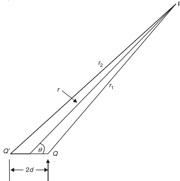
Figure 1.19 Electric dipole ( r \gg d ).
