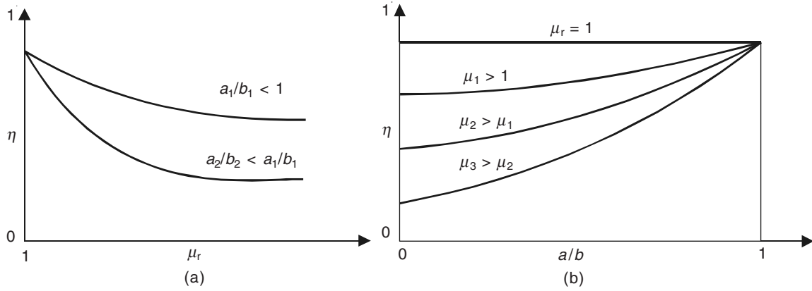
Figure 9.3 Degree of shielding \eta as a function of the two parameters— \mu_r and a/b .
