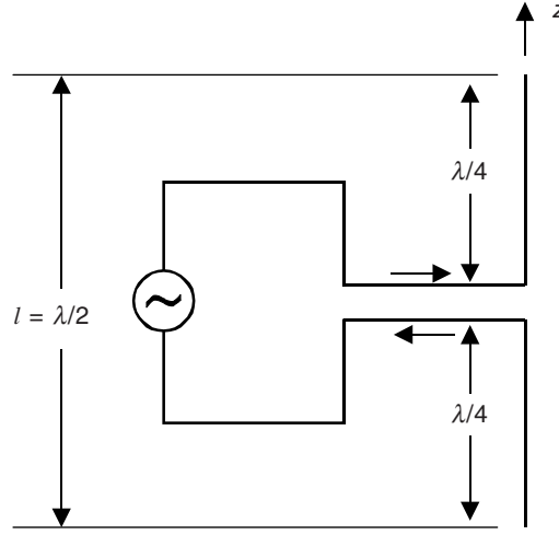
Figure 19.8 Centre-fed half-wave antenna.
