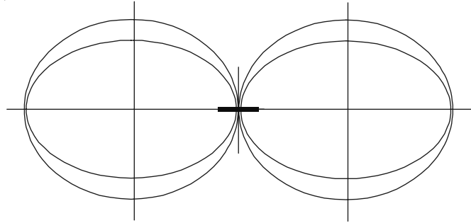
Figure 19.9 Angular plots of [\cos \{(\pi/2) \cos \theta\}/\sin \theta] and [\cos^2 \{(\pi/2) \cos \theta\}/\cos^2 \theta] showing respectively the angular distributions of \mathbf{E} and \mathbf{S}_{av} for a half-wave antenna at r \gg \lambda . The plots are similar to those of the dipole (Figure 19.7) except that these are flatter compared to those of the dipole, indicating a larger fraction of its power in the equatorial plane.
