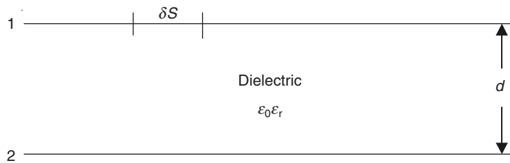
Figure 2.7 A parallel plate capacitor.
