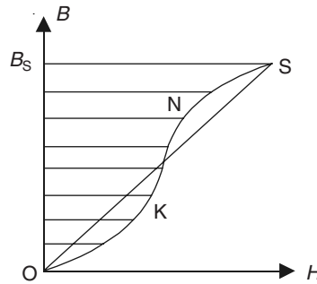
Figure 11.16 B-H curve for iron.
