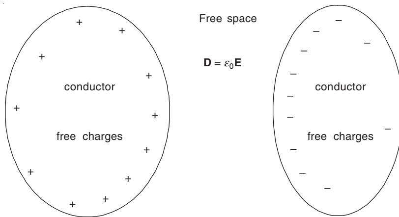
Figure 2.5 Free charges on a two-conductor system.
