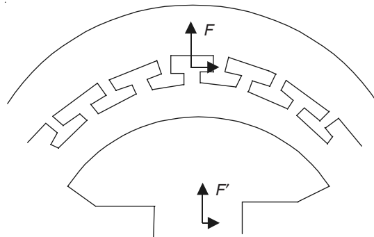
Figure 20.11 Stator and rotor of a rotating alternator.
