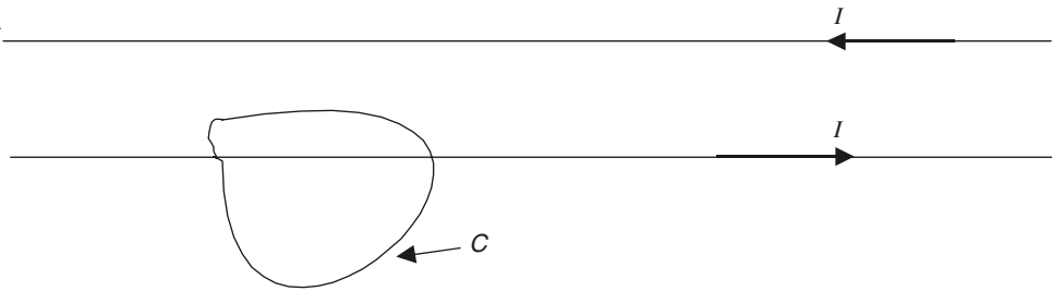
Figure 7.17 Effect of a return wire on the \mathbf{H} \cdot d\mathbf{l} contour.
