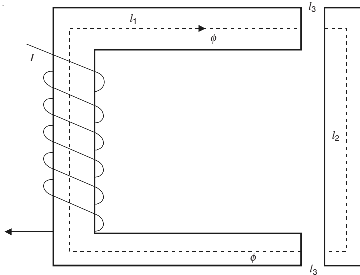
Figure 8.15 Magnetic circuit with air-gaps.
