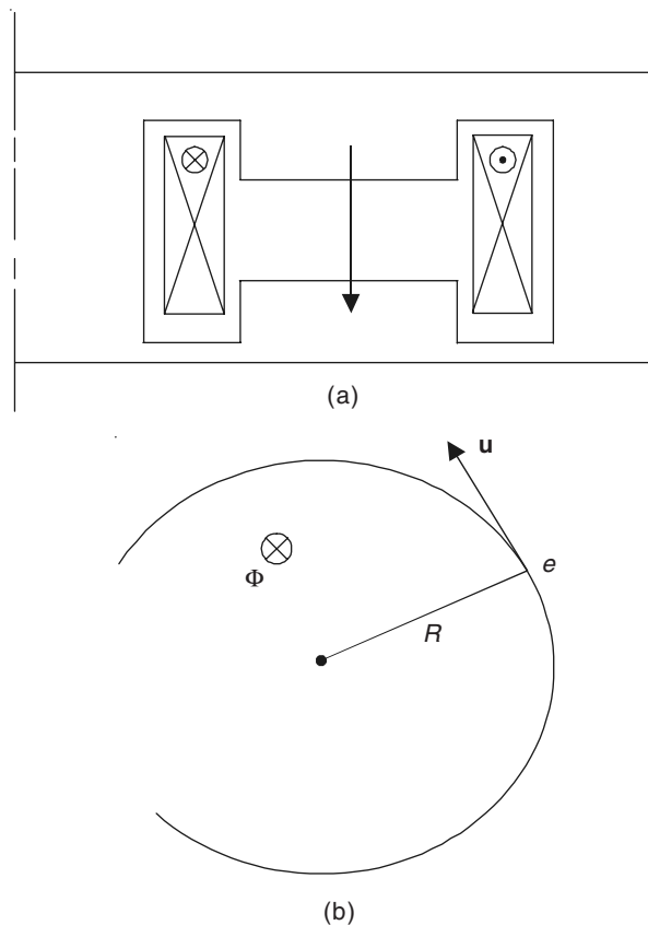
Figure 20.8 (a) Section of a Betatron and (b) the orbital path of electrons in a Betatron.
