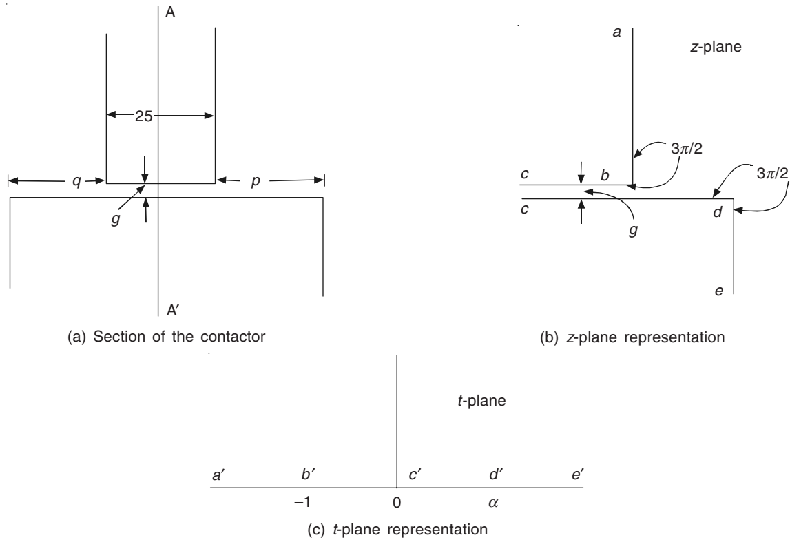
Figure 9.4 The problem of the magnet and the armature of the contactor, with the transformations.
