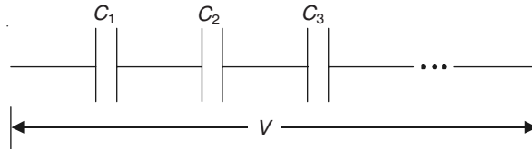
Figure 2.14 Capacitors in series.
