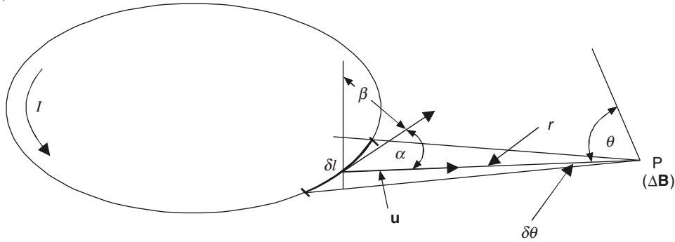
Figure 7.10 A planar current-carrying contour.
