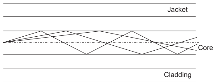
(b) Step-index Multimode
