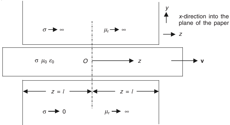
Figure 15.21 A thin slab of conductor moving in the +z-direction in the air-gap of a magnetic circuit.
