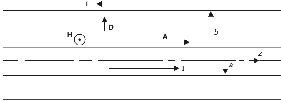
Figure 14.14 Coaxial cable, carrying time-varying current.
