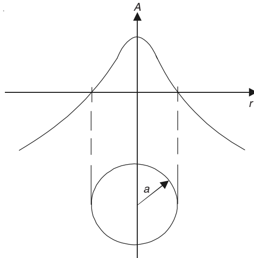
Figure 13.12 Vector potential of a single straight conductor of circular cross-section.
