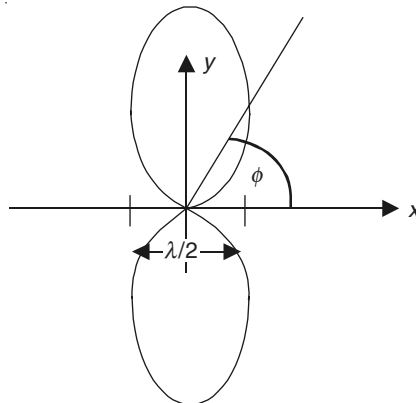
Figure 19.12 Two-element broadside array.
