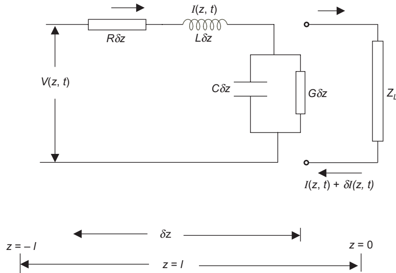
Figure 18.6 Circuit representation of a section of a lossy transmission line.
