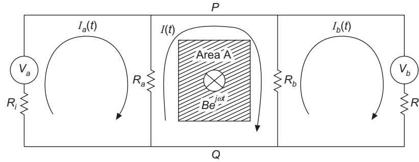
Figure A.6.5 Circulating current circuit showing the loop currents.
