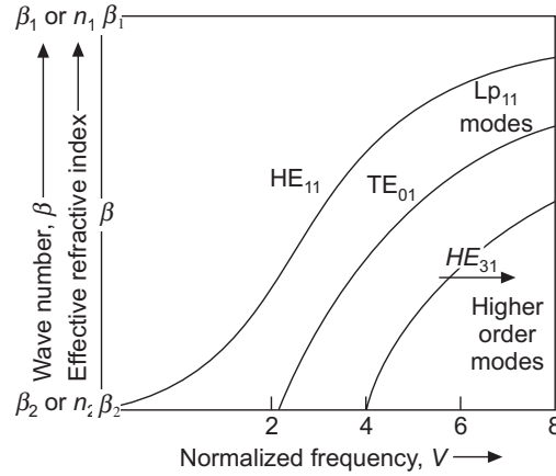
Figure 22.12 Mode chart or b - V diagram of an optical fibre (step-index).
