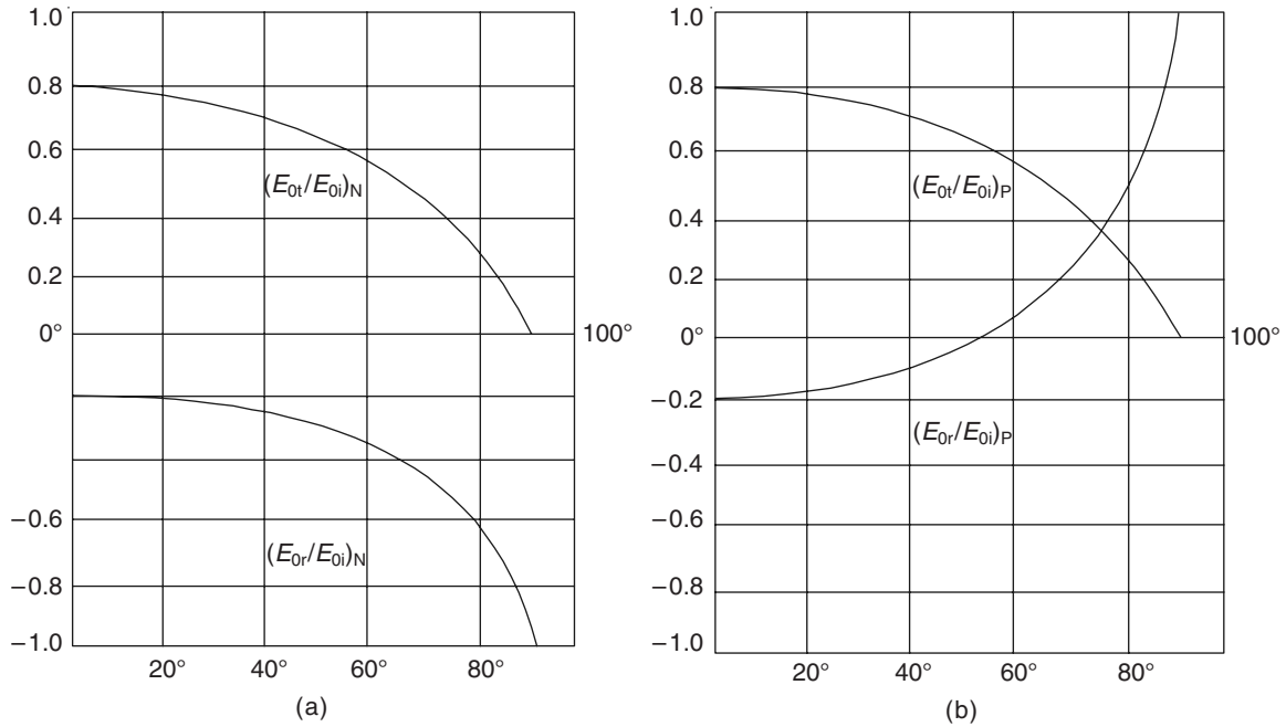
Figure 17.18 The ratios (E_{0t}/E_{0i}) and (E_{0r}/E_{0i}) as functions of the angle of incidence \theta_i for n_1/n_2 = 1.0/1.5 , for (a) E vector normal to the plane of incidence; and for (b) E vector parallel to the plane of incidence.
