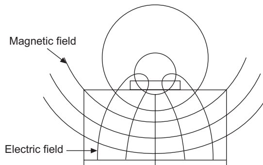
Figure 22.20(b) Pattern of electromagnetic field of a microstrip line (at any section normal to the direction of transmission).
