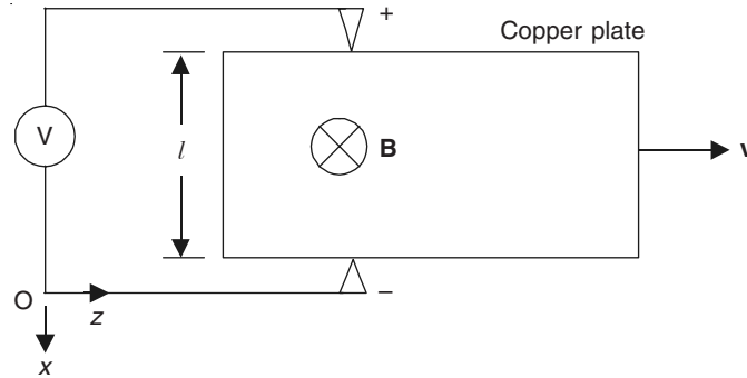
Figure 10.27 A rectangular plate type unipolar generator.
