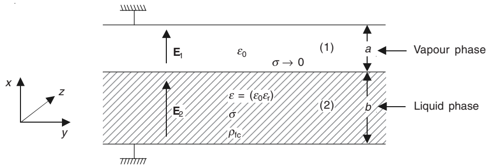
Figure 16.1 Simplified one-dimensional model of a tank containing charged liquid.
