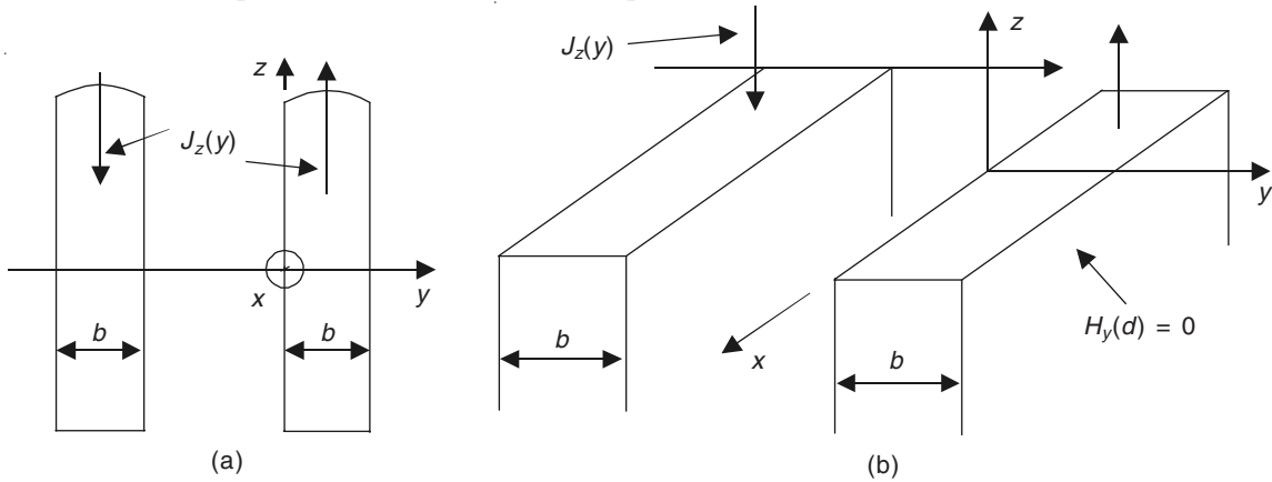
Figure 15.29 Two parallel strip conductors of thickness b carrying the same alternating current in opposite directions: (a) sectional view in the plane x = 0 and (b) isometric view.
