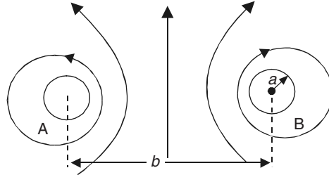
Figure 10.15(b) Self-inductance of parallel conductor circuit.
