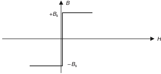
Figure 15.26 Step-function B - H characteristic of the material.
