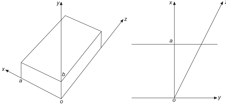
Figure 18.13(c) Rectangular waveguide ( a \times b ) and its limit as b \rightarrow \infty giving the plane parallel waveguide.
