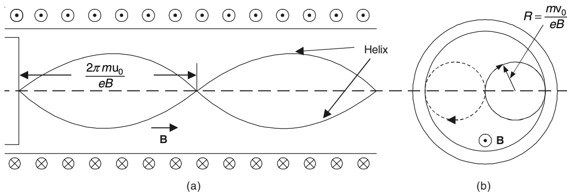
Figure 20.9 Magnetic focussing of an electron beam: (a) side view and (b) end view.
