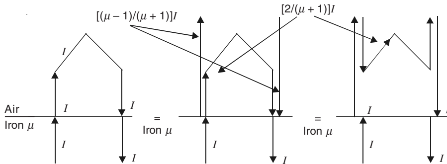
Figure 9.16 Images of partially embedded coil-end, giving the field in iron, as obtained by Hammond and Carpenter respectively.
