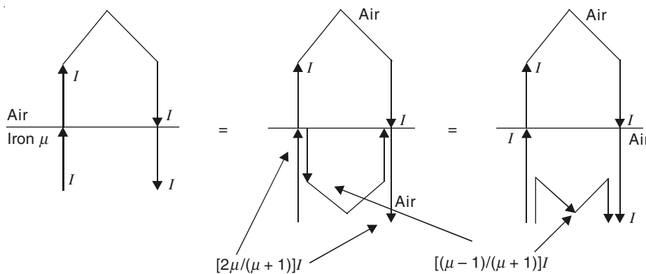
Figure 9.15 Alternative images in air, for the partially embedded coil-ends as derived by Hammond and Carpenter respectively.
