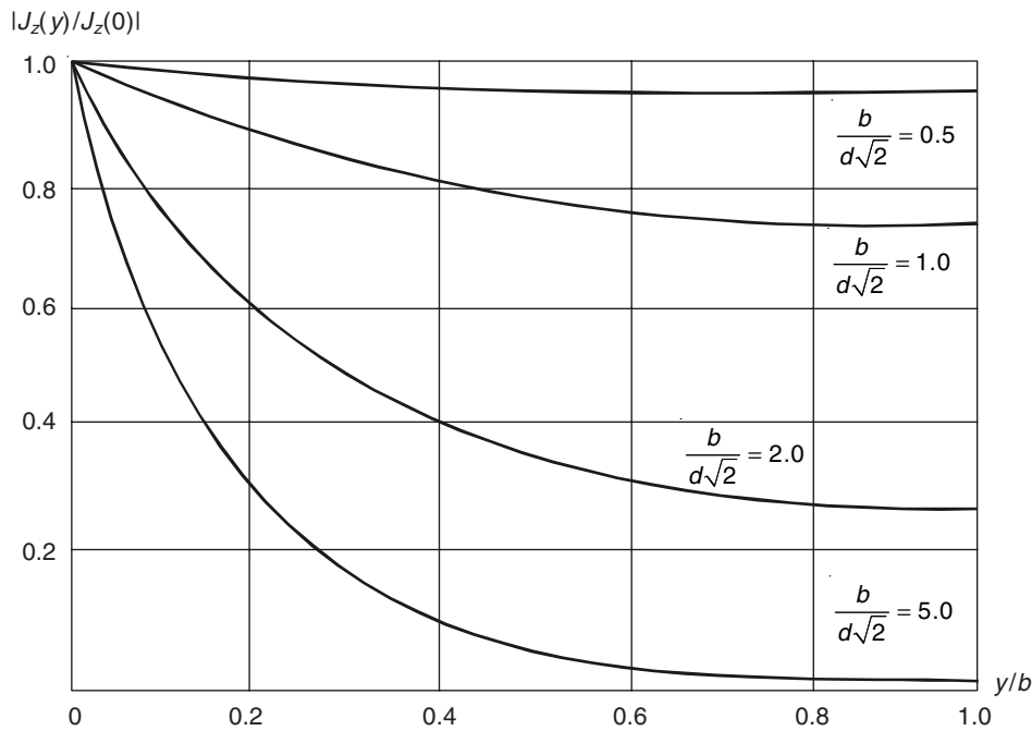
Figure 15.30 Current distribution in the strips of Figure 15.29.
