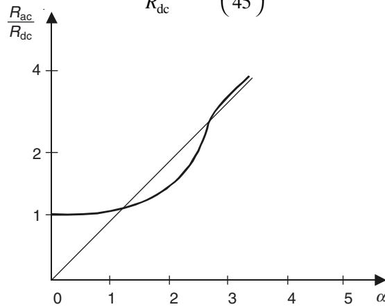
Figure 15.9 AC resistance of a flat sheet.
