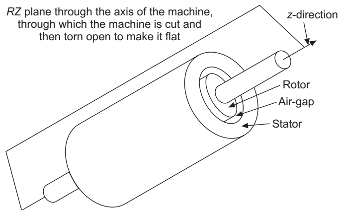
Figure 22.13 Schematic of the basic structure of a rotating machine (not to scale). Slots and windings are not shown. Also the end-structure has been omitted. The magnetic field in the air-gap is radial, the current flow in the conductors located in the slots is axial. The effective current sheet has axially flowing currents. The magnetic field in the air gap is rotating circumferentially. The air gap magnetic field and the rotor currents interact to produce a force on the rotor such that it also rotates in the same direction as the magnetic field.
