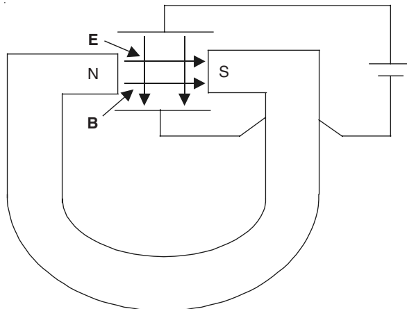
Figure 14.13(b) U-shaped magnet and parallel plate capacitor.
