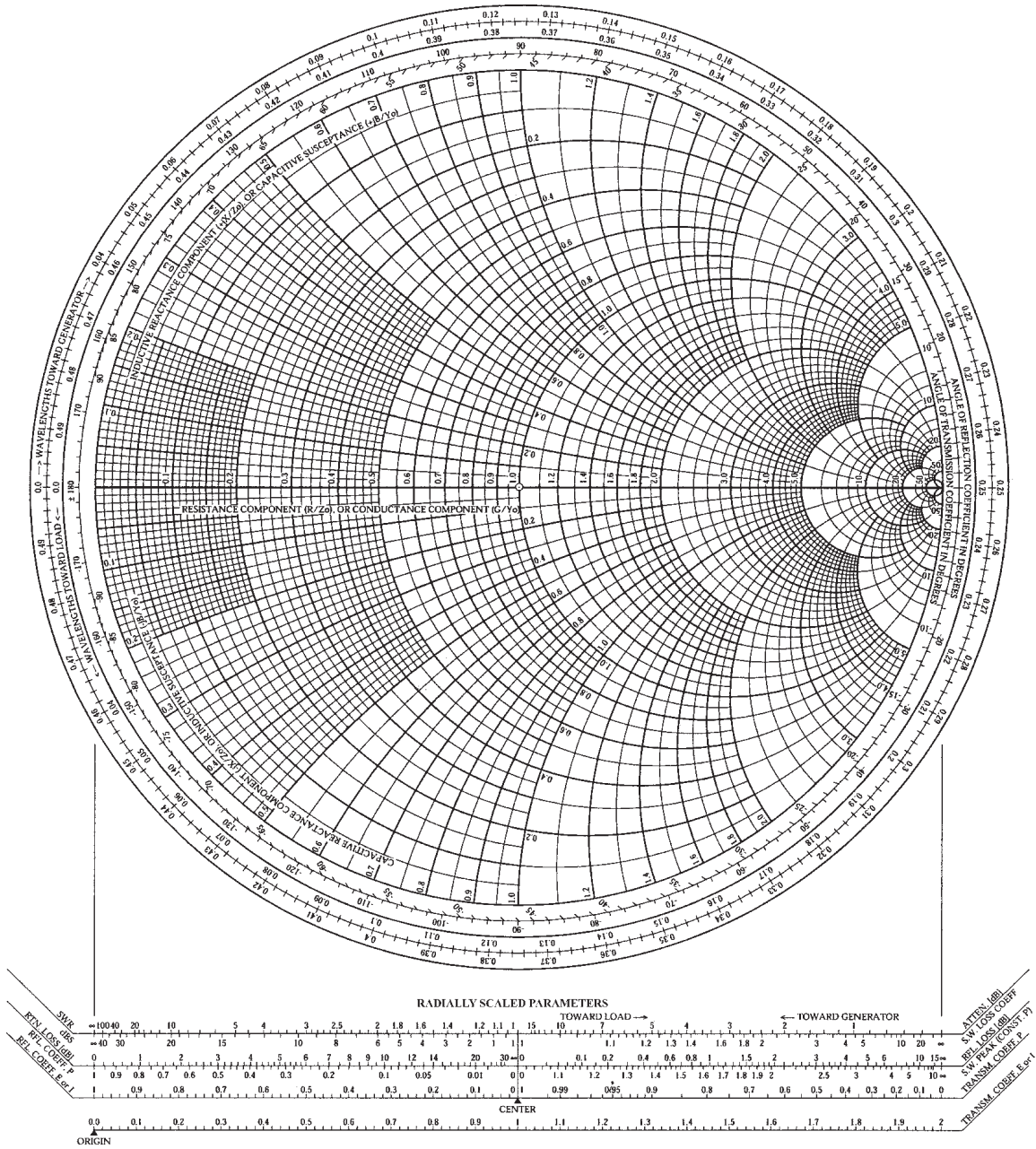
Figure A.7.7 Impedance or admittance coordinates.
