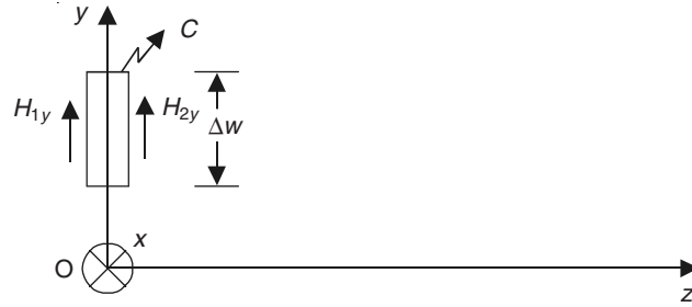
Figure 17.12 A closed contour C in the plane z = 0 (view of the y - z plane). Induced currents are in the x -direction into the plane of the paper.
