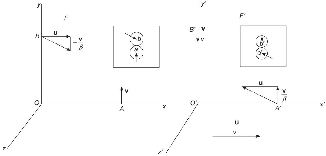
Figure 20.4(a) Experiment with colliding spheres.
