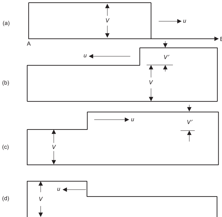
Figure 18.3 Repeated reflections on the transmission line.
