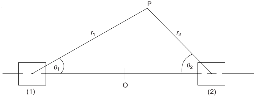
Figure 13.11 Inductance of a pair of parallel long conductors of any cross-section.
