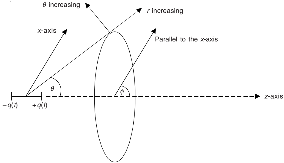
Figure 19.2 Oscillating dipole with spherical polar coordinate system.
