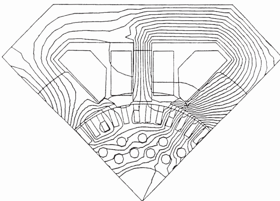
Figure 21.13 DC machine—flux distribution on 300% load.
