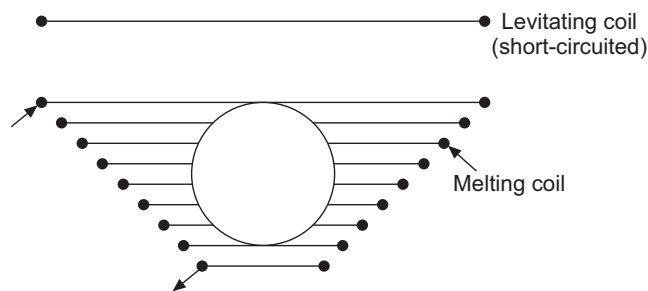
Figure 22.18(a) Induction melting of a spherical metal ball with levitation.
