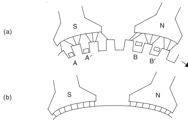
Figure 10.10 Section of a dc generator.
