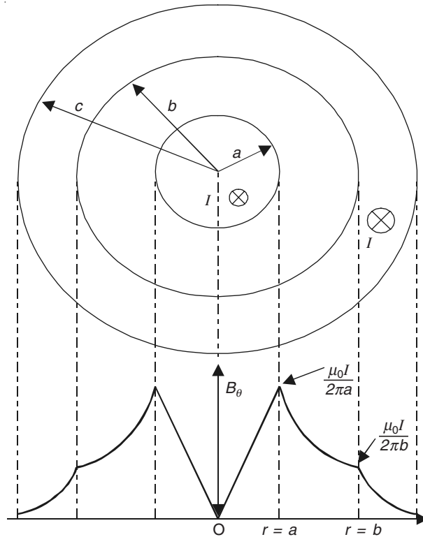
Figure 7.24 A coaxial cable.
