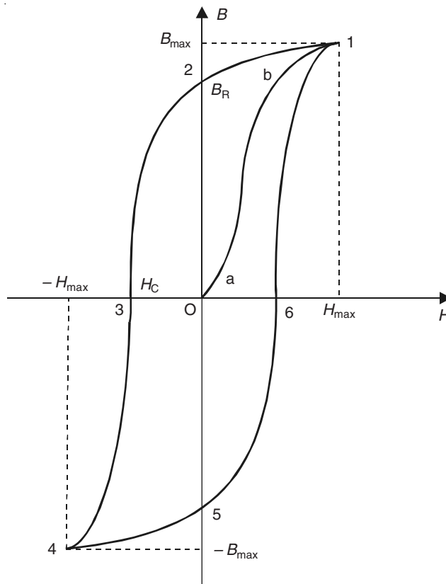
Figure 8.11 \mathbf{B} - \mathbf{H} loop for an iron specimen.
