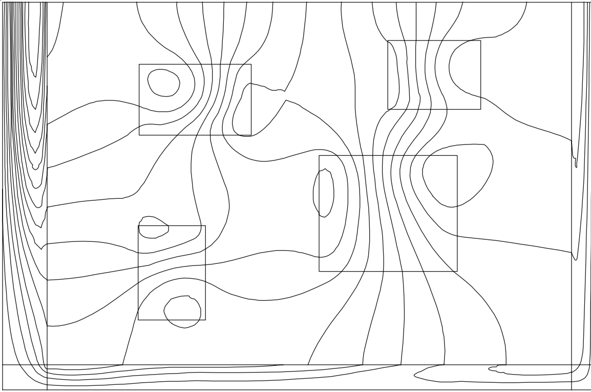
Figure 21.7 Busbars enclosed in a conducting box of mild steel—half geometry with dummy bar—analysis in x - y coordinates at t = \frac{\pi}{2} .
