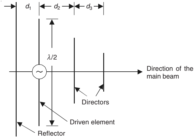
Figure 19.14 An Uda-Yagi array.
