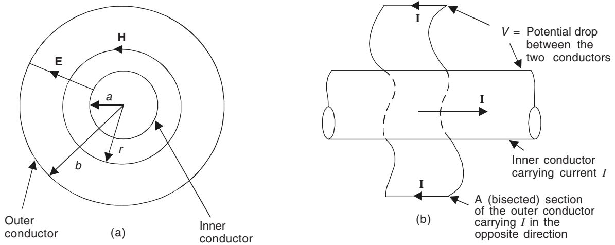
Figure 14.7 A coaxial cable carrying direct current.
