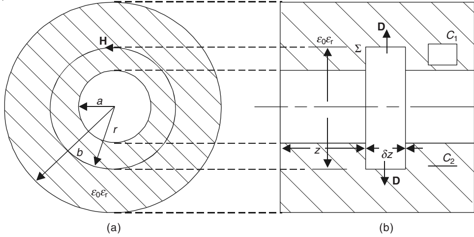
Figure 14.11 A perfect coaxial cable carrying time-varying current.
