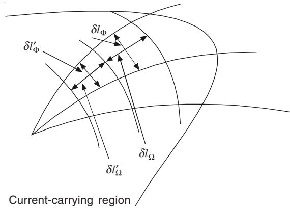
Figure 9.23 Kernel and field-lines within the current-carrying region.
