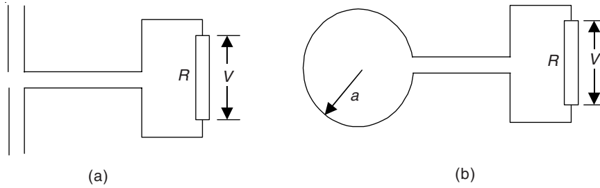
Figure 19.15 Oscillating electric and magnetic dipoles used as receiving antennae.
