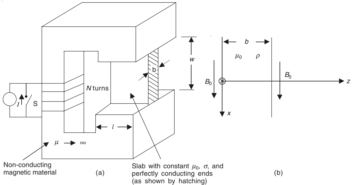
Figure 15.15 (a) System devised to study magnetic diffusion as an electrical transient; (b) coordinate system for the one-dimensional diffusion model.
