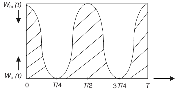
Figure 14.4 Oscillation of energy between the capacitor and the inductor of a resonant oscillatory circuit.
