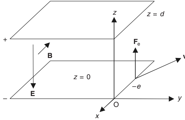
Figure 11.13 A parallel-plate diode with transverse magnetic field.
