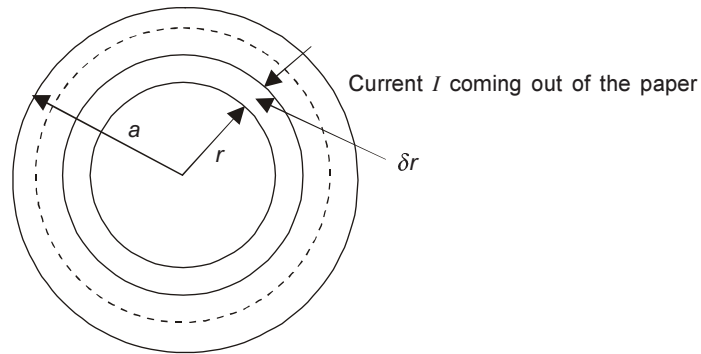
Figure 11.21 A circular conductor.
