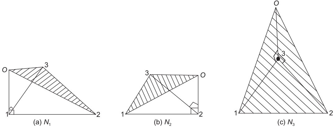
Figure 21.18 Shape functions (or linear interpolation functions) for the triangular element 1–2–3.
