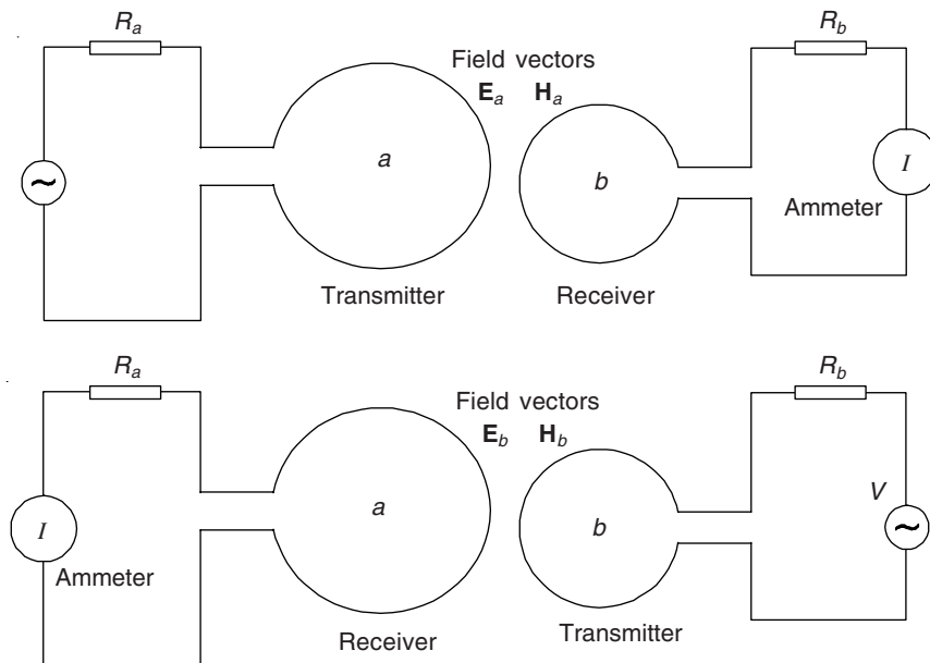
Figure 19.19 A pair of loop antennae with the source in a at the top, and then in b (bottom). The frequency and the impedances remain unchanged.
