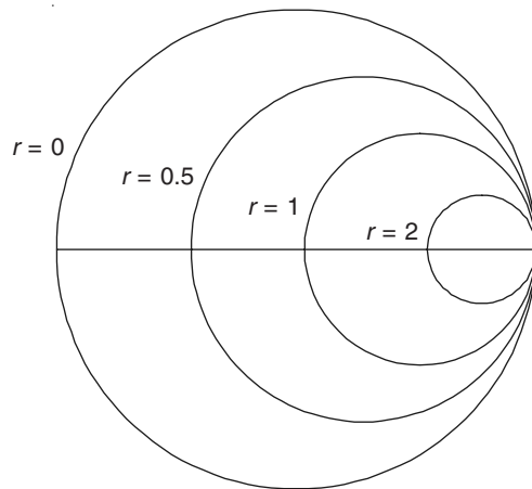
Figure A.7.5 Representation of real part of \Gamma(l) in Smith chart.
