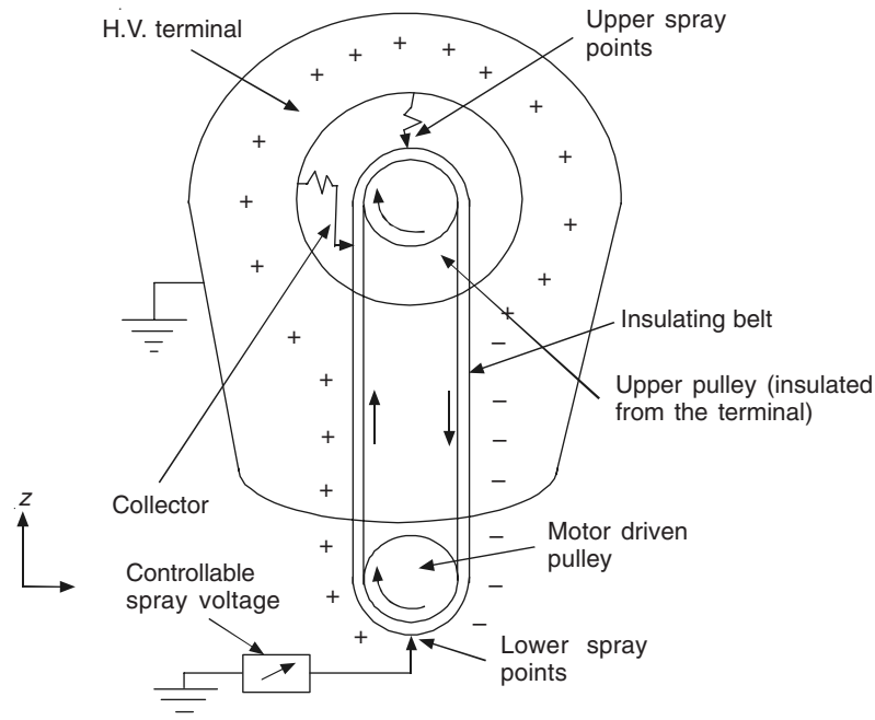
Figure 16.3 Section of a Van-de-Graff generator.
