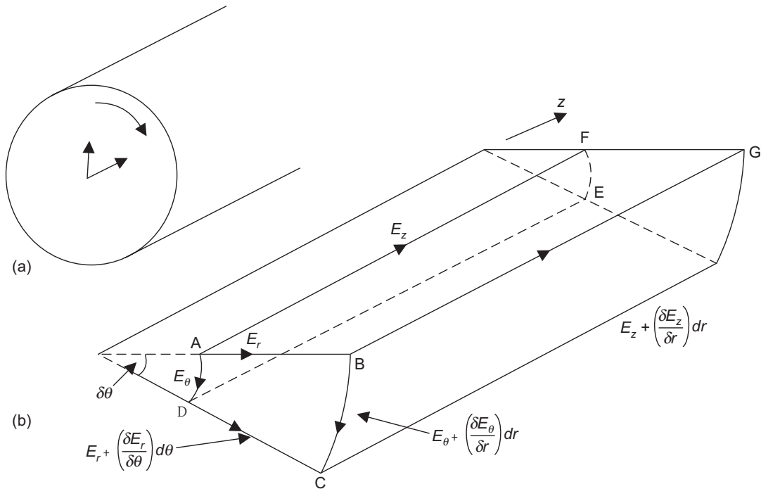
Figure 18.14 A cylindrical waveguide and its elemental section.
