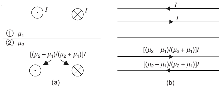
Figure 9.9 Images of infinite line currents on a plane interface.
