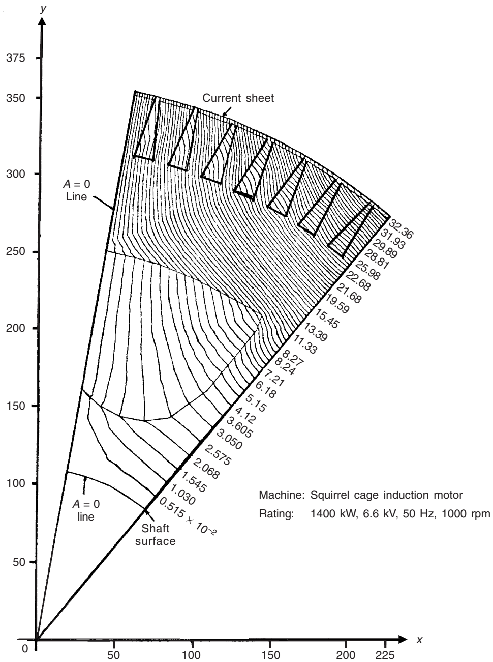
Figure 21.15 Magnetic flux distribution in the rotor region for modified shape ventilating hole, without shaft.
