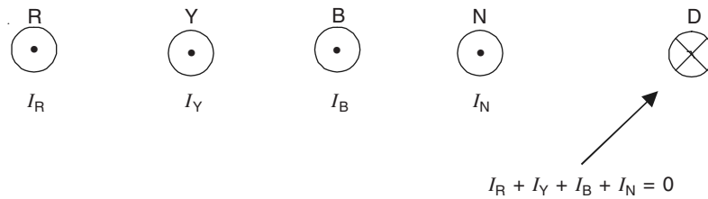
Figure 13.14 Three-phase transmission line with a neutral and a dummy return.
