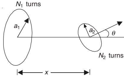
Figure 10.16 A small circular coil on the axis of a large circular coil.
