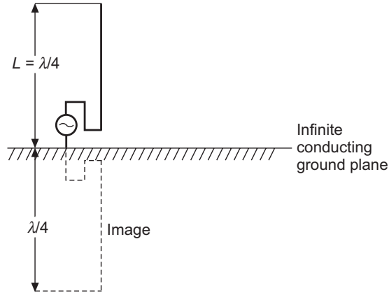
Figure 19.9(a) The monopole antenna. (Its image is also shown in the figure.)
