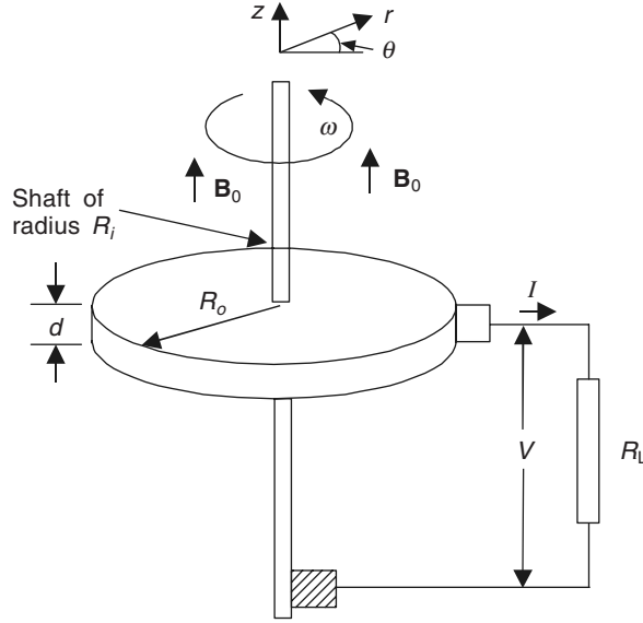
Figure 20.17 Faraday's disc generator, connected to a load resistor.
