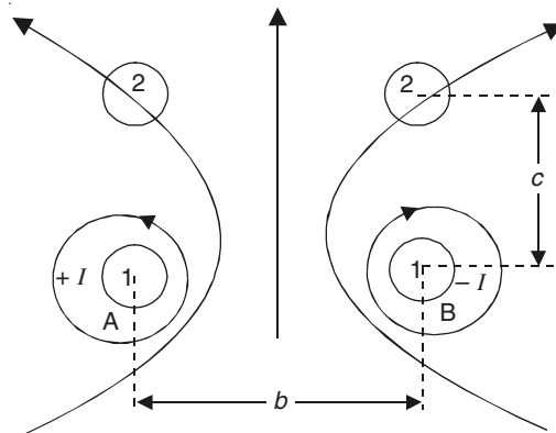
Figure 10.15(a) Mutual inductance between parallel conductors of finite cross-section.
