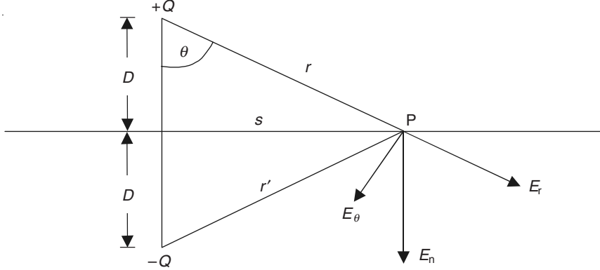
Figure 4.20 E_n on the conducting surface.
