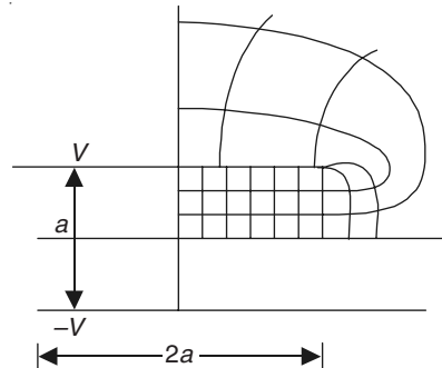
Figure 5.4 Curvilinear squares for an electrode system.
