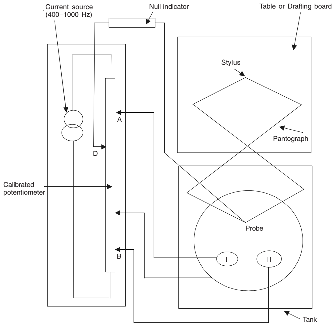
Figure 5.6 Electrolytic tank for the experimental solution of the Laplace's equation.
