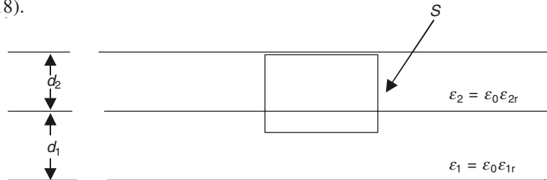
Figure 2.18 Parallel plate capacitor with mixed dielectrics.
