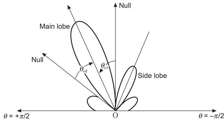
Figure 19.10(d) Radiation pattern as a polar plot.
