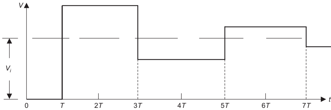
Figure 18.4 The voltage wave at any point on the cable AB.
