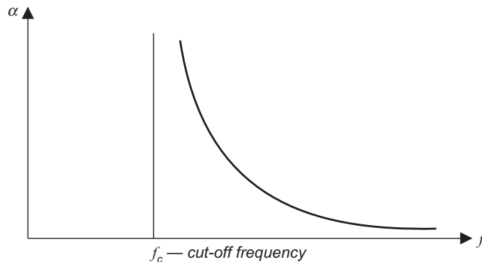
Figure 18.19 Attenuation as a function of the frequency.
