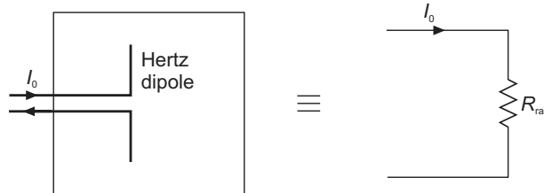
Figure 19.4(a) Equivalent resistance of the Hertz dipole.
