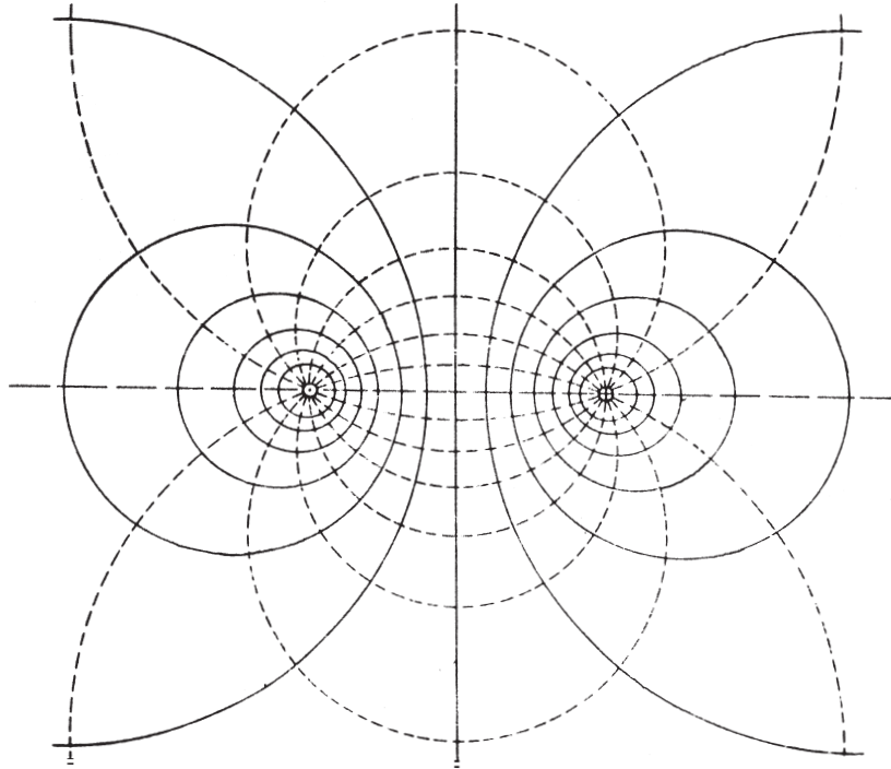
Figure 7.26(b) Flux plot about two equal and opposite parallel currents.
