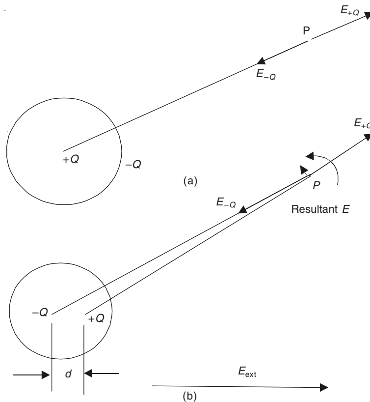
Figure 2.2 (a) Model of a neutral atom; (b) the same atom in an external electric field.
