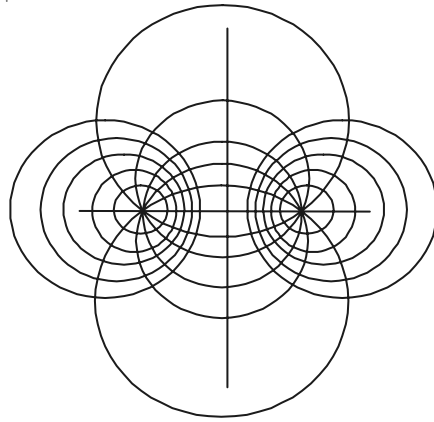
Figure 4.13 Field between two charged cylindrical conductors with uniform dielectric.
