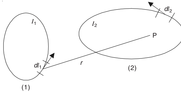
Figure 13.9 Mutual inductance between two loops.
