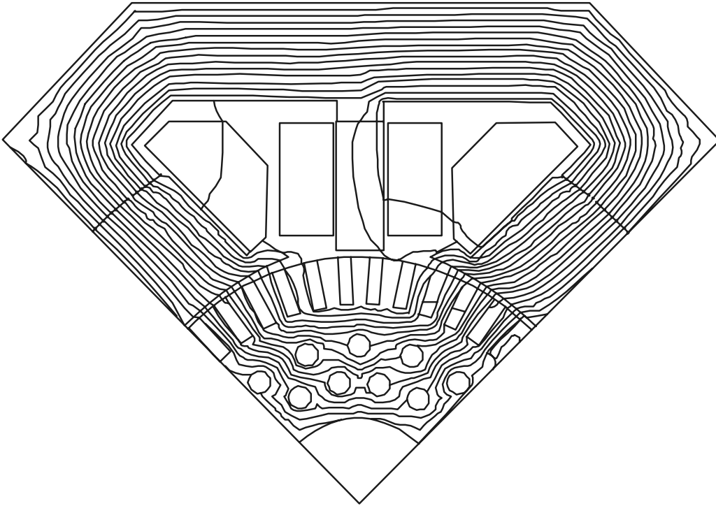
Figure 21.10 DC machine—flux distribution on 50% load.
