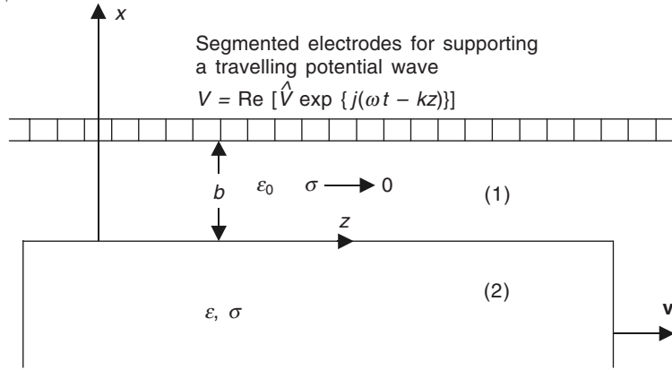
Figure 16.5 A semi-infinite block of slightly conducting material moving to the right with a constant velocity \mathbf{v} = \mathbf{i}_z v .
