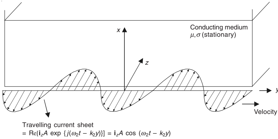
Figure 15.23 Stationary conducting medium, subjected to a travelling current sheet.
