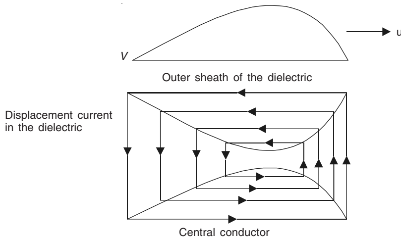
Figure 14.12 Voltage and current waves in the dielectric of the coaxial cable carrying time-varying current.
