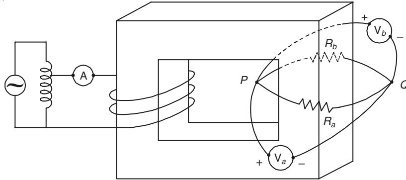
Figure A.6.1 Pictorial view of a magnetic circuit for generating circulating current.
