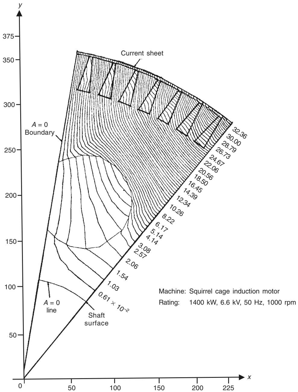
Figure 21.14 Magnetic flux distribution in the rotor region for circular ventilating hole, without shaft.
