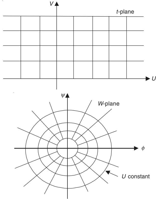
Figure 4.16 The logarithmic transformation W = \phi + j\psi = (\Psi_1/\pi) \ln t .
