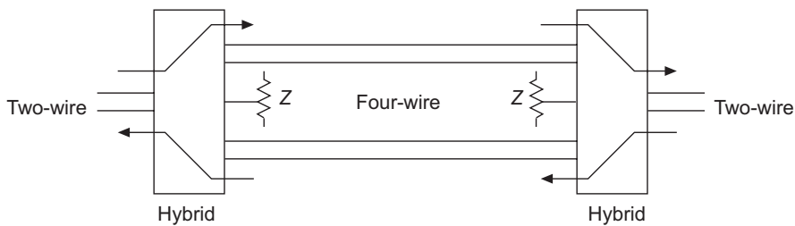
Figure 22.3 Two-wire to four-wire connections in telephone lines using hybrids.
