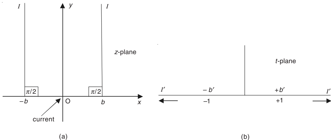
Figure 9.5 Current between two infinite parallel permeable planes: (a) z -plane representation and (b) t -plane representation.
