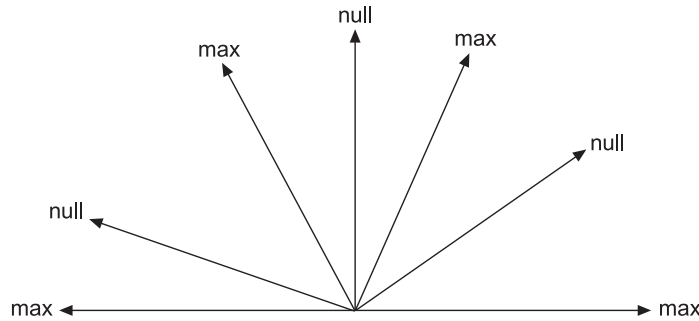
Figure 19.13(b) Maxima and nulls in a radiation pattern of a two-element array.
