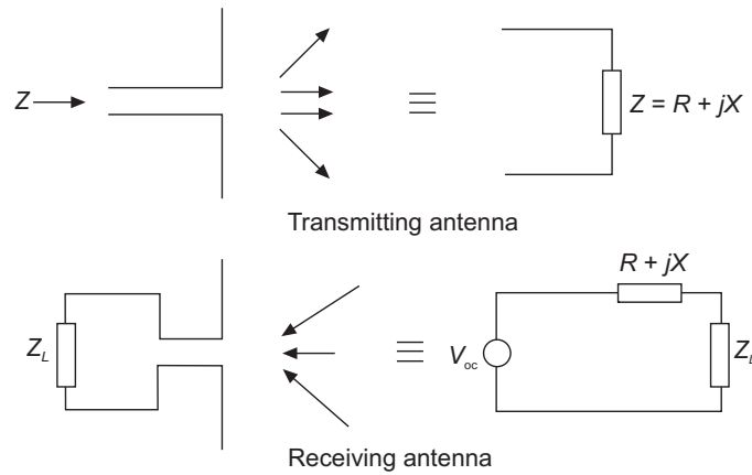
Figure 19.17(b) Equivalent circuits of the antenna.
