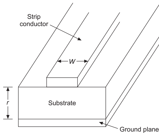
Figure 22.20(a) Microstrip transmission line.
