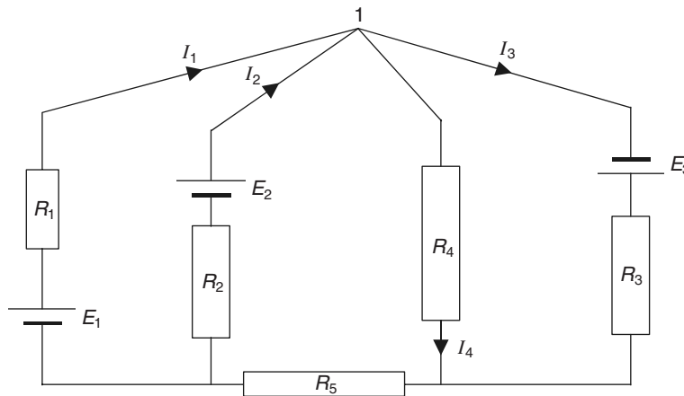
Figure 6.9 An electrical network.
