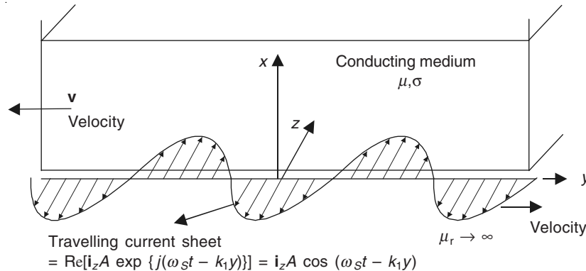
Figure 15.22 Moving conducting medium, subjected to a travelling current sheet.
