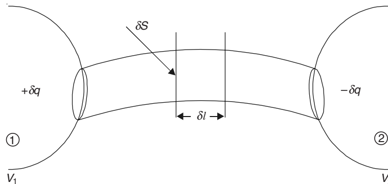
Figure 3.1 Energy in terms of field quantities.
