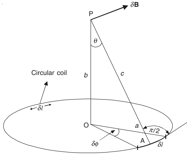
Figure 7.8 A circular coil.
