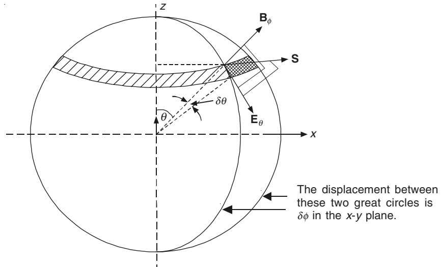
Figure 19.4 Surface of integration around the dipole. Note that the three vectors \mathbf{E}_{\theta} , \mathbf{B}_{\phi} and \mathbf{S} are mutually orthogonal.
