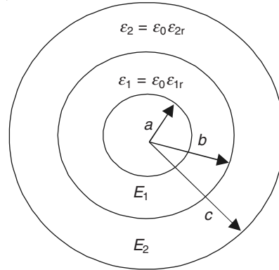
Figure 2.19 Concentric cylinders with mixed dielectrics.
