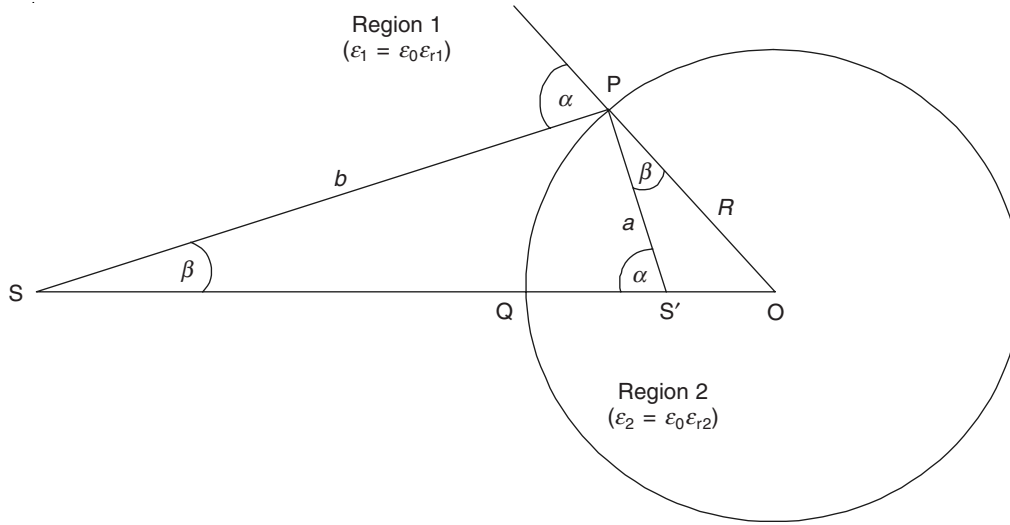
Figure 4.22 Line charge Q running parallel to the circular cylinder of radius R .
