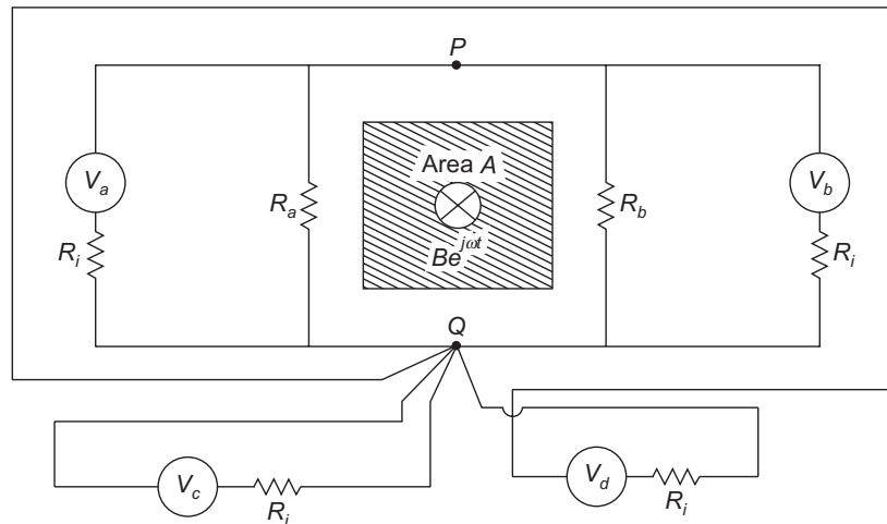
Figure A.6.6 Circulating current circuit with two additional voltmeters apparently shorted at the point Q .
