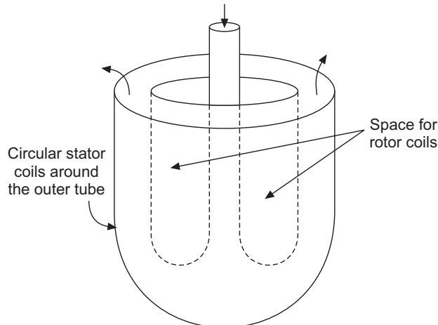
(b) A possible shape of a tubular linear induction pump
