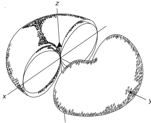
Figure 19.7 Plots of angular distributions of \mathbf{E} (or \mathbf{H} ) and \mathbf{S}_{av} of the Hertzian dipole.
