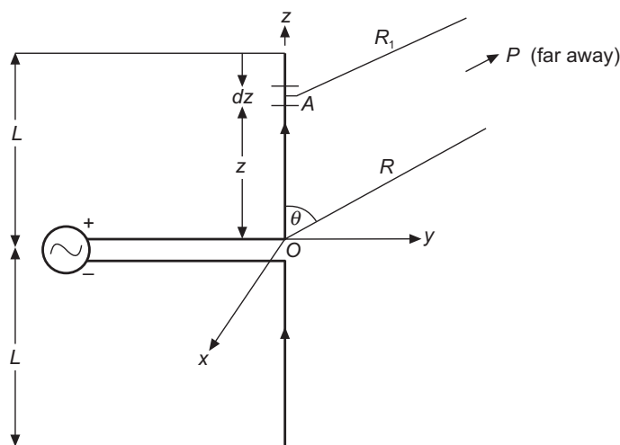
Figure 19.7(a) A linear dipole antenna of length 2L .
