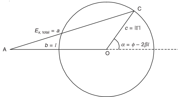
Figure A.7.3 Graphical representation of components of E wave.
