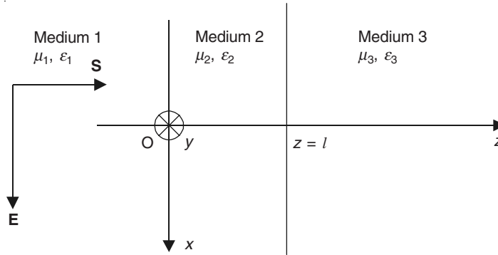
Figure 17.10 Plane wave in three dielectrics.
