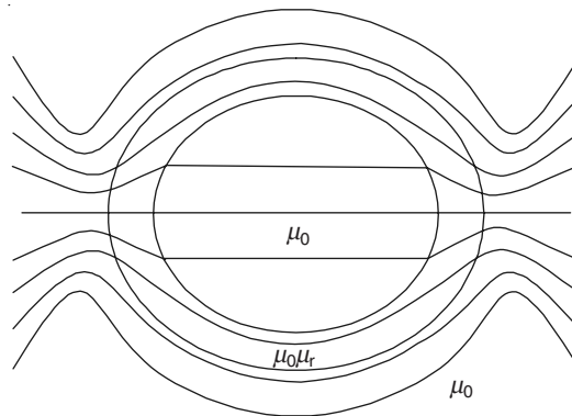
Figure 9.2 \mathbf{H} field in a screening cylinder.
