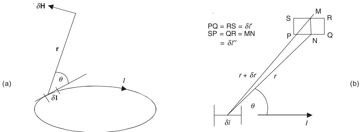
Figure 13.3 A current circuit and its element \delta l .
