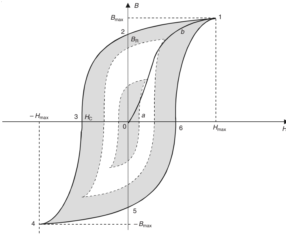
Figure 8.13 B - H corresponding to different values of H_{\max} for a material.
