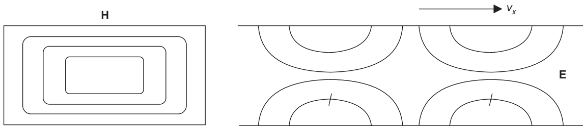
Figure 18.11 TM_{11} mode in a rectangular waveguide.
