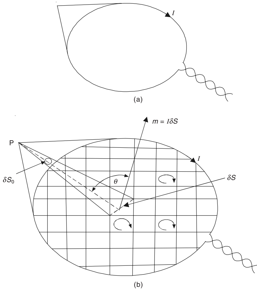
Figure 7.21 (a) The actual circuit and (b) the equivalent magnetic shell.
