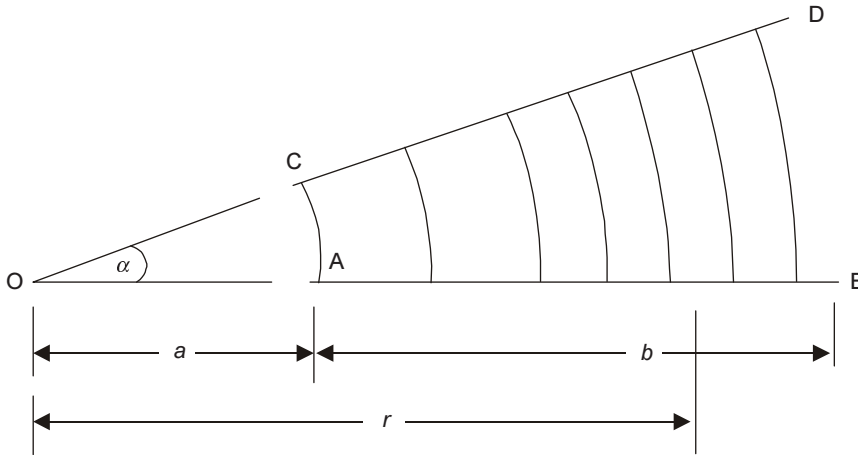
Figure 2.8(a) Two-plate tapered capacitor.
