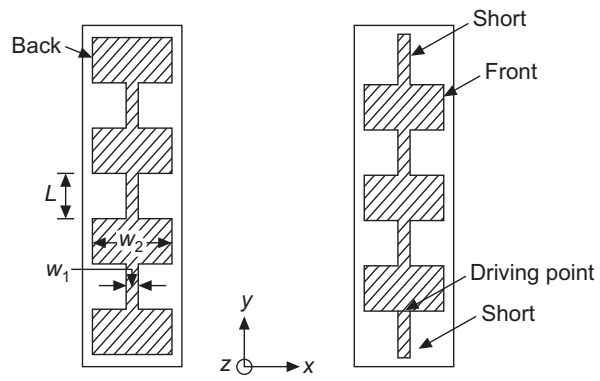
Figure 22.22 A printed antenna: seven-section omnidirectional microstrip antenna.
