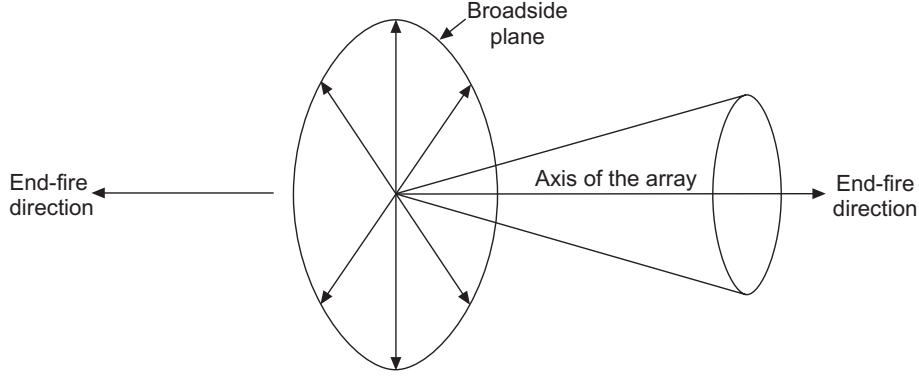
Figure 19.14(a) Broadside and end-fire directions of an antenna array.
