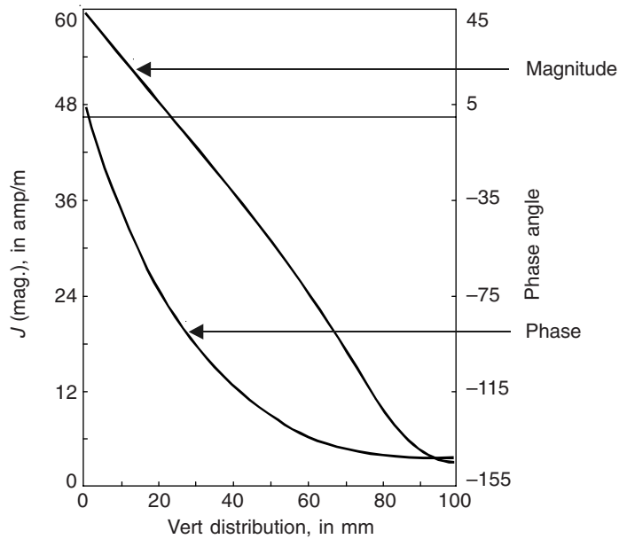
Figure 21.3 Current density distribution inside a conductor in a slot.
