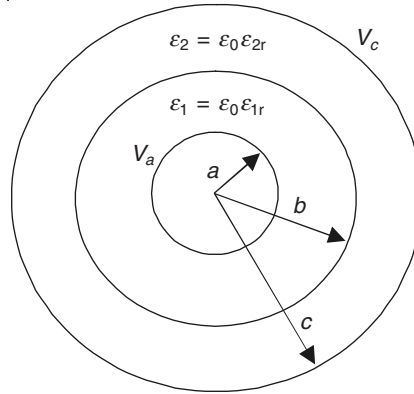
Figure 2.21 Concentric spheres with mixed dielectrics.
