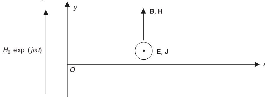
Figure 15.1 Semi-infinite conducting block subjected to an alternating magnetic field.
