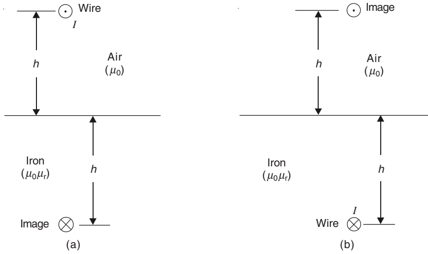
Figure 9.6 Images of a wire carrying a current I : (a) outside a plane block of iron of permeability \mu_0\mu_r and (b) embedded in the same block of iron.
