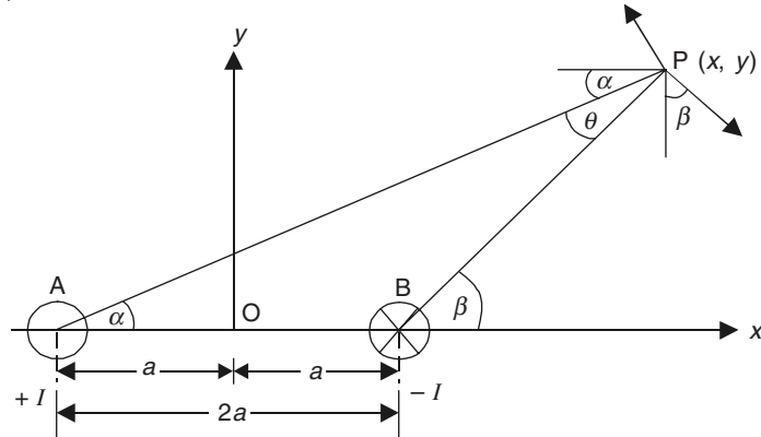
Figure 7.26(a) Magnetic field due to a parallel go-and-return circuit.
