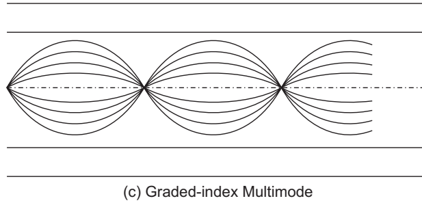
(c) Graded-index Multimode Figure 22.8 Optical fibres transmission modes.
