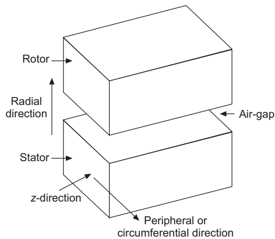
Figure 22.15 Topologically opened form of the rotating machine, converting it into flat linear machine (the dimensions are not to scale). The windings and slots have not been shown. (Basis for a single-sided flat linear machine).
