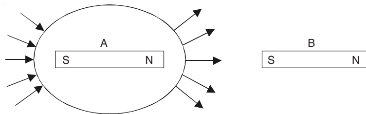
Figure 11.19 Force between two bar-magnets and stresses in the field space.
