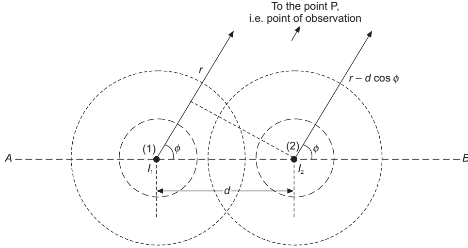
Figure 19.13(a) A two-element array of isotropic antennae.
