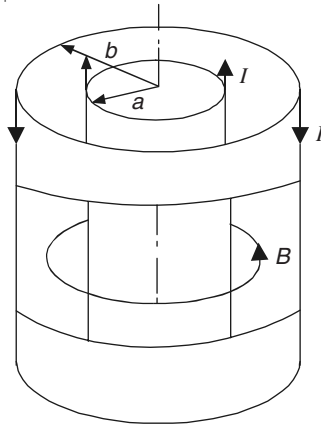
Figure 11.20 A portion of concentric tubes carrying current +I and -I in opposite directions.
