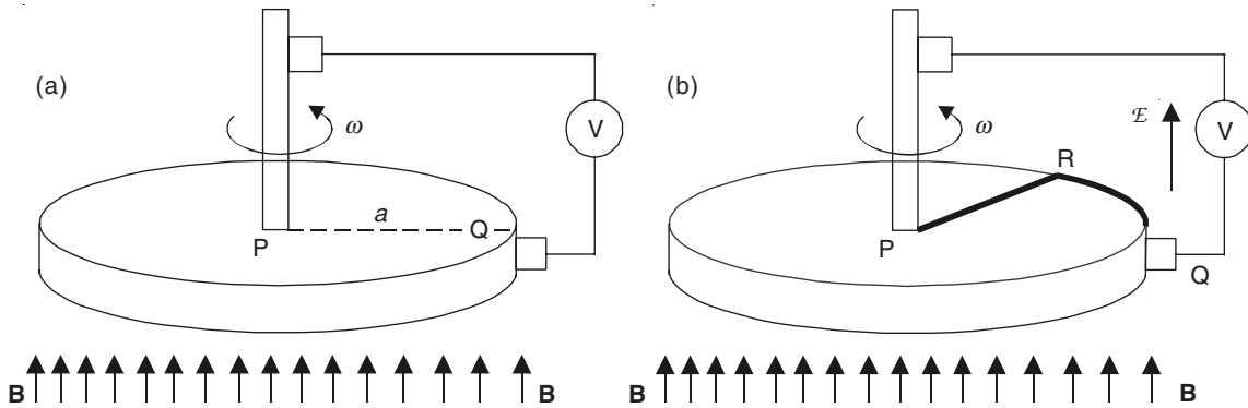
Figure 10.30 A Faraday disc.
