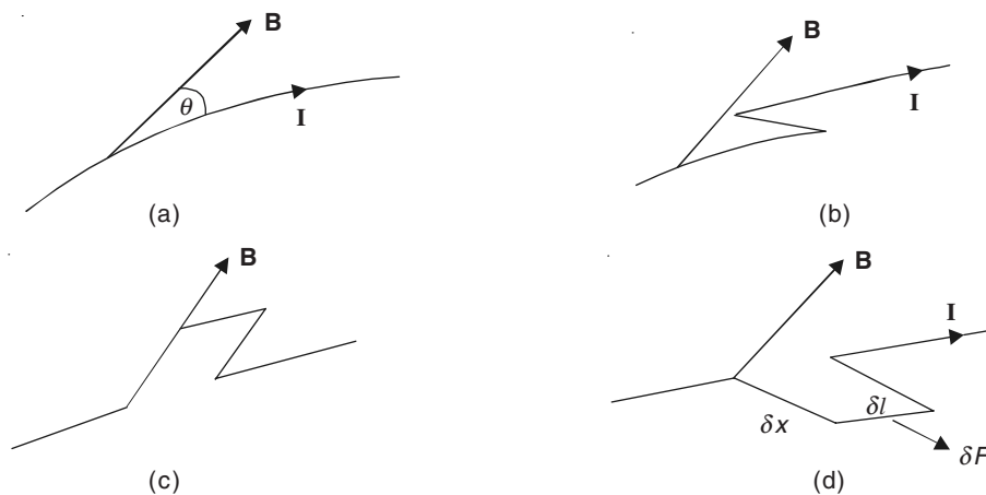
Figure 11.2 A deformable circuit in a magnetic field \mathbf{B} .
