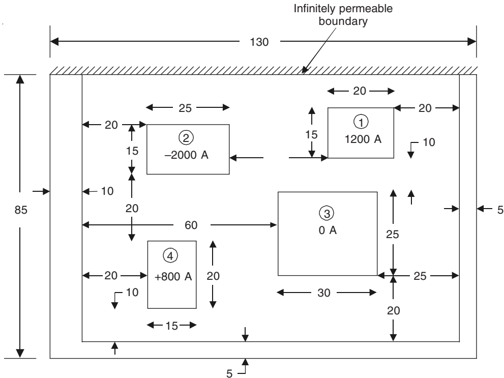
Figure 21.5 Busbars enclosed in a conducting box.
