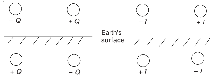
Figure 13.7 Charges and line currents above the equipotential earth surface, and their equivalent images.
