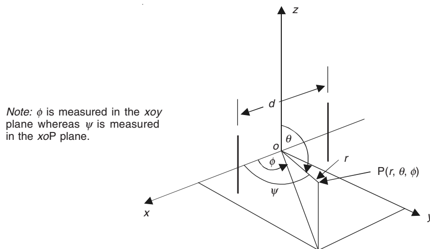
Figure 19.11 A pair of parallel half-wave antennae, d metres apart.
