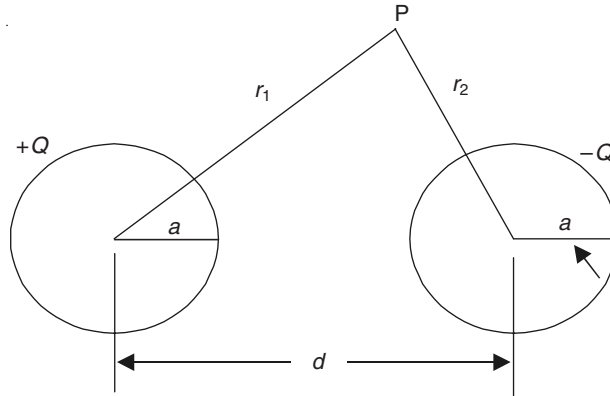
Figure 2.10 Parallel circular cylinders.
