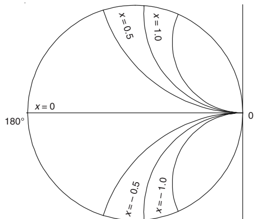
Figure A.7.6 Representation of coefficient of j in Smith chart.
