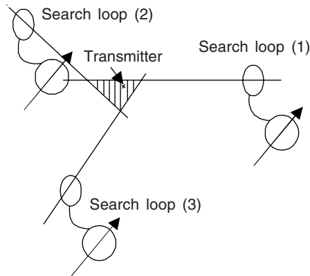
Figure 19.16 Locating a transmitter by search loop antennae.
