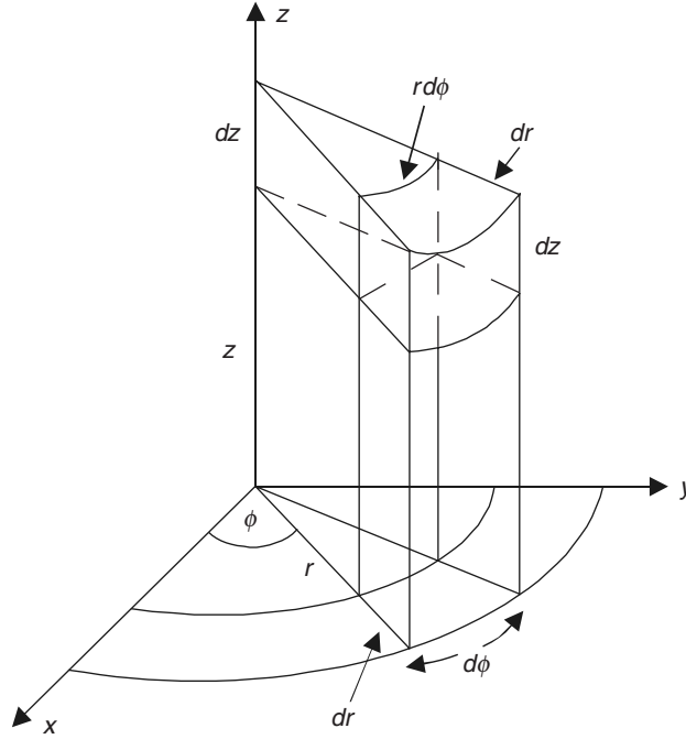
Figure A.4.4 Cylindrical polar coordinate system.
