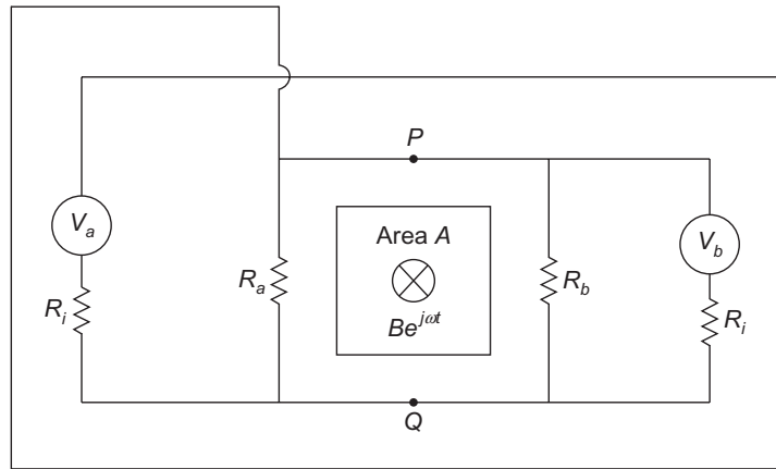
Figure A.6.7 Circulating current circuit with the voltmeter V_a connected with an additional loop around the non-conservative field region.
