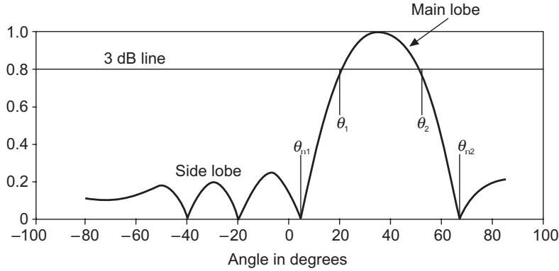
Figure 19.10(e) Cartesian plot of the radiation pattern.
