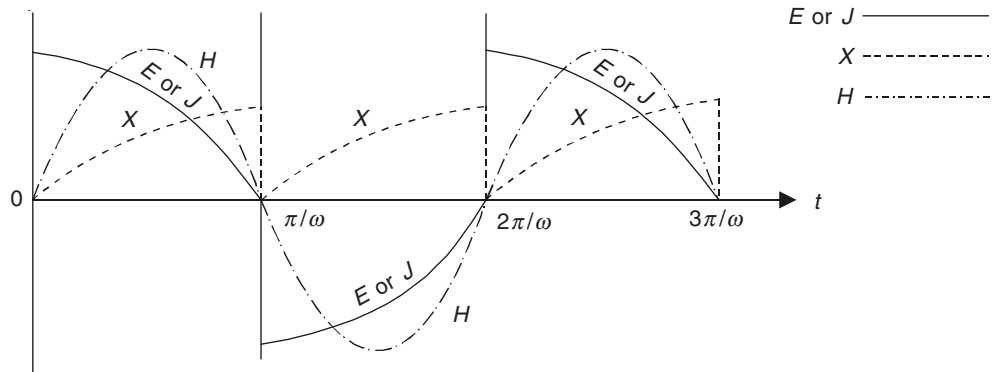
Figure 15.27 Plots of wave-shapes of E (or J ), X and H in a thick saturated block of iron.
