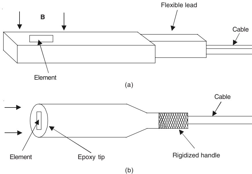
Figure 9.25 Some typical Hall probe configurations: (a) typical flat (transverse) probe and (b) axial probe.
