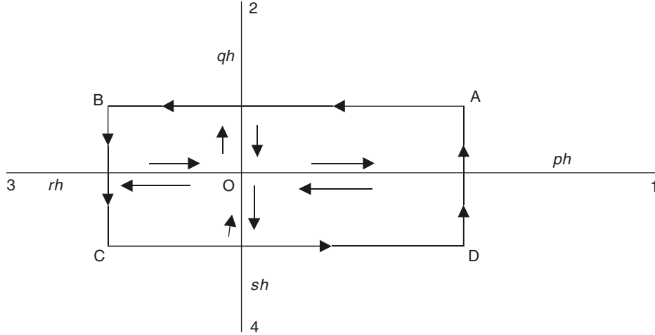
Figure 5.9 Asymmetrical 5-point star with the integration paths shown.
