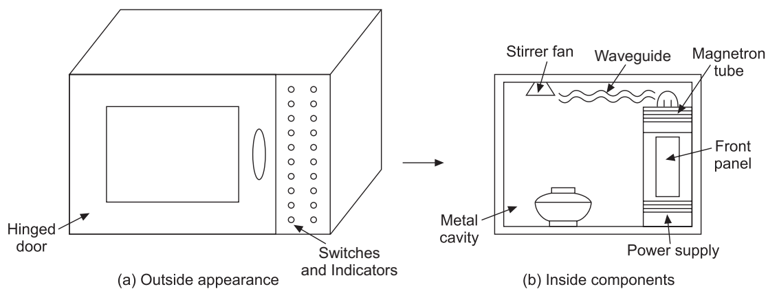
Figure 22.1 Microwave oven (a typical one).
