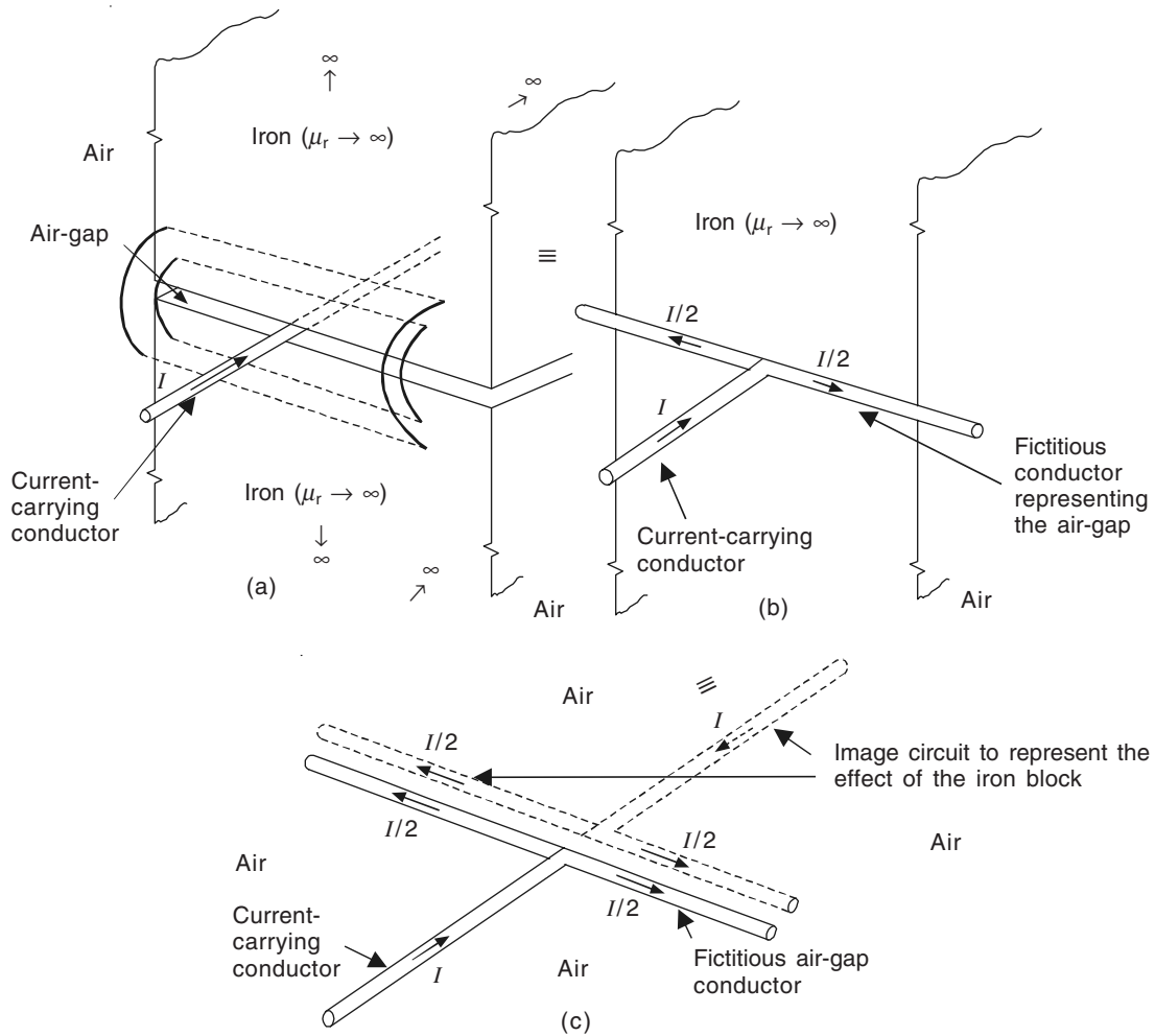
Figure 9.18 A line conductor penetrating an infinitely permeable iron block with a short width air-gap. (The block is semi-infinite, and the air-gap and the conductor extend to infinity. The diagram shows a section of the whole region.) (a) Current-carrying conductor in the air-gap. It also gives a pictorial view of the imaginary fringing flux across the air-gap. (b) Air-gap discontinuity from the iron has been replaced by its fictitious current-carrying conductor. (c) Iron has been removed and its effect produced by the image circuit.
