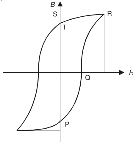
Figure 11.18 Hysteresis loop of iron.
