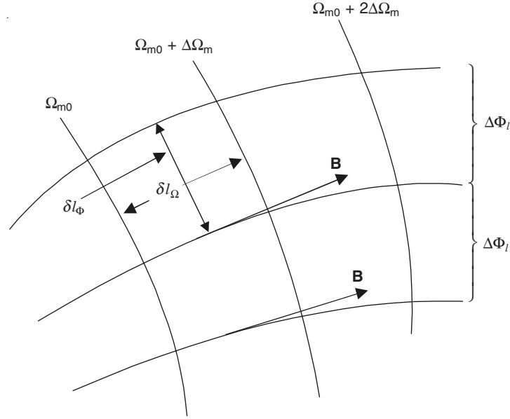
Figure 9.22 A two-dimensional magnetostatic field.
