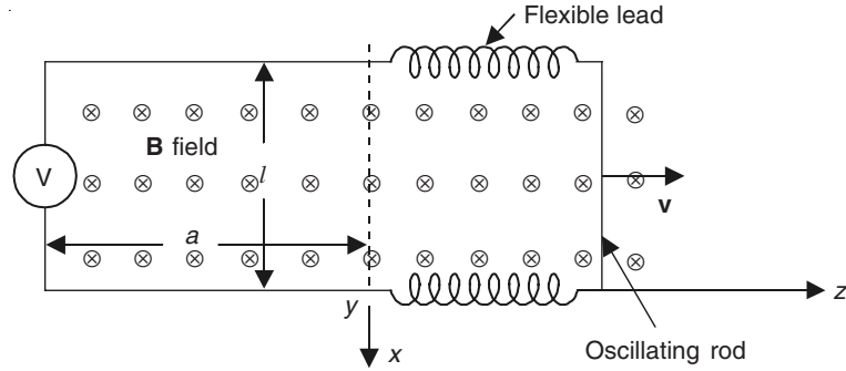
Figure 10.26 Principle of operation of the commutatorless dc generator.
