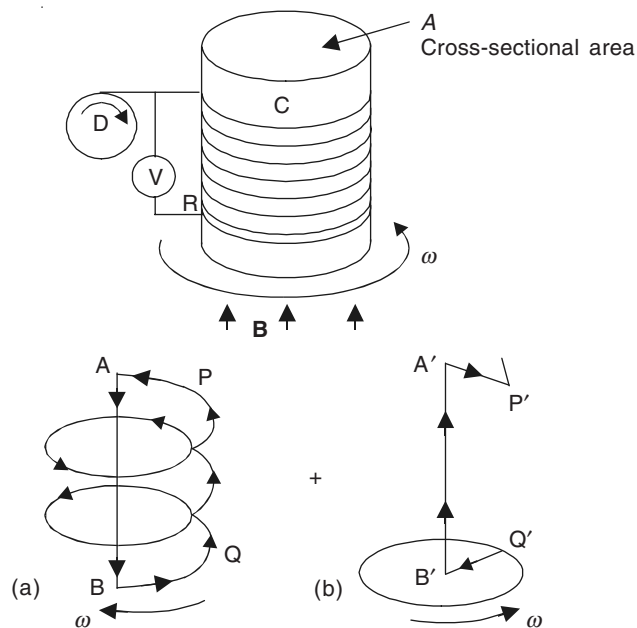
Figure 10.23 Time-varying number of turns on a coil in a uniform steady magnetic field.
