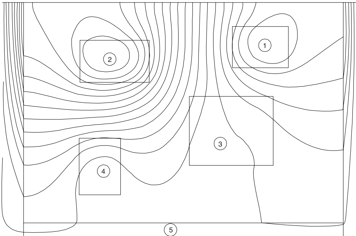
Figure 21.6 Busbars enclosed in a conducting box of mild steel—half geometry with dummy bar—analysis in x - y coordinates at t = 0 .
