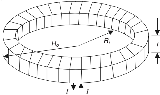
Figure 10.17 Inductance of a toroidal coil.
