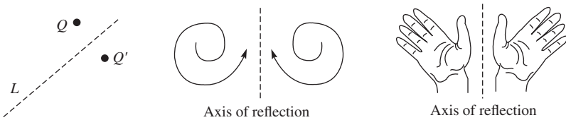
Figure 27.1 Reflected images
