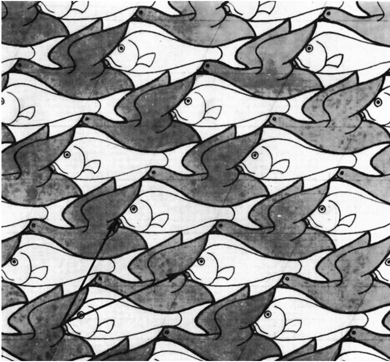
Figure 28.12 Study of Regular Division of the Plane with Fish and Birds, 1938. Escher drawing with symmetry group p1 . The arrows are translation vectors.
