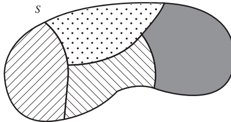
Figure 0.5 Partition of S into four subsets.
