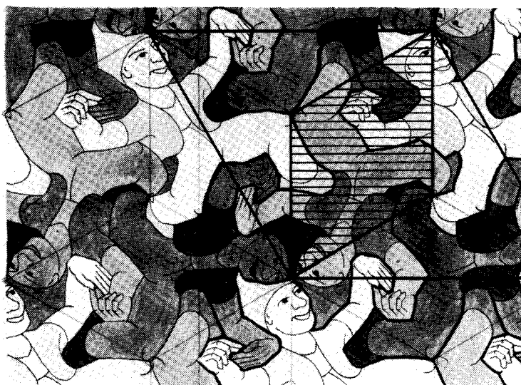
Figure 28.21 A lattice unit and generating region for the patterns in Figures 28.12, 28.13, and 28.14. Generating regions are shaded with bars.
