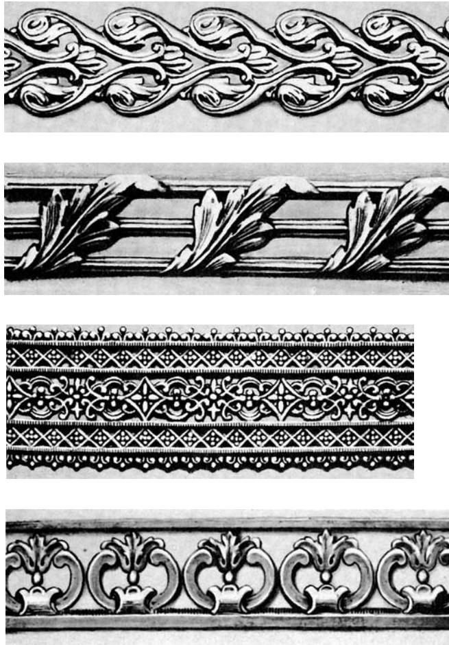
Figure 28.1 Frieze patterns
