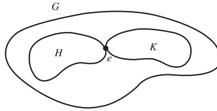
Figure 9.1 For the internal direct product, H and K must be subgroups of the same group.
