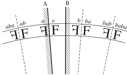
Figure 26.3 The group D_{180} —reflections in mirrors at a 1^\circ angle
