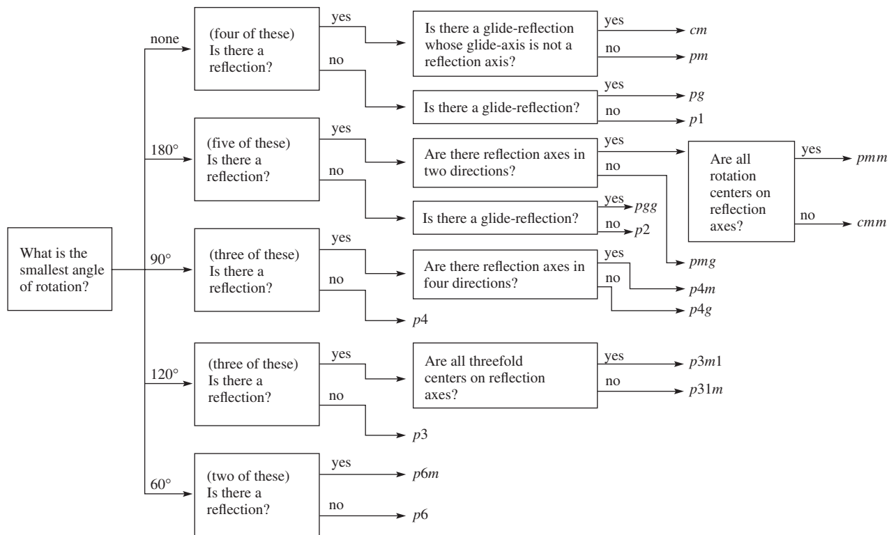
Figure 28.18 Identification flowchart for symmetries of plane periodic patterns
