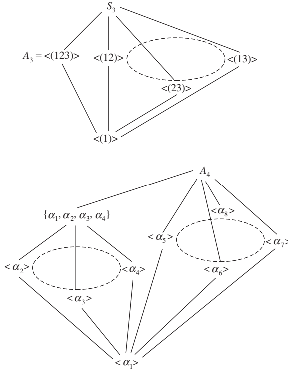
Figure 24.1 Lattices of subgroups for S_3 and A_4 .
