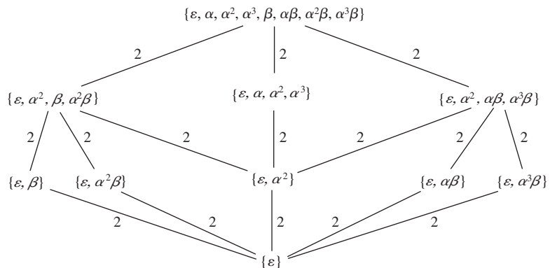
Figure 32.1 Lattice of subgroups of the group of field automorphisms of Q(\sqrt[4]{2}, i) , where \alpha : i \rightarrow i and \sqrt[4]{2} \rightarrow -i\sqrt[4]{2} , \beta : i \rightarrow -i , and \sqrt[4]{2} \rightarrow \sqrt[4]{2}
