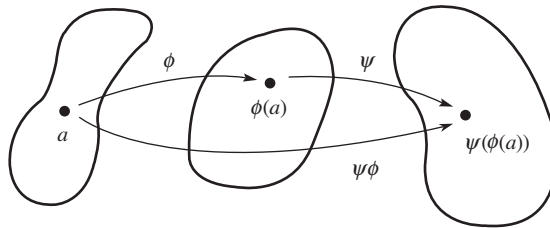
Figure 0.6 Composition of functions \phi and \psi .
