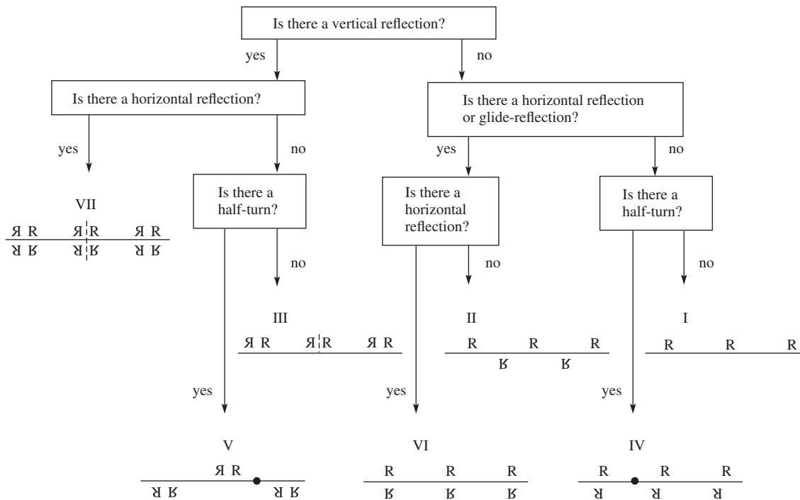
Figure 28.10 Recognition chart for frieze patterns. Adapted from [6, p. 83].
