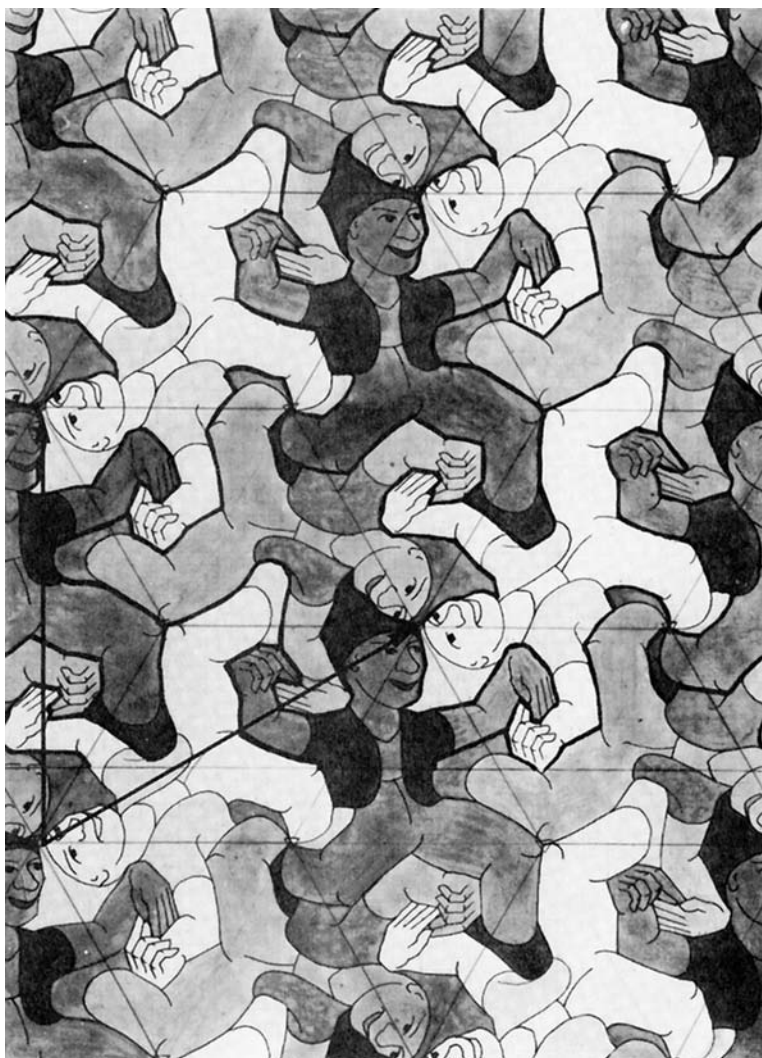
Figure 28.14 Study of Regular Division of the Plane with Human Figures, 1938. Escher drawing with symmetry p3 (disregarding shading). The inserted arrows are translation vectors.
